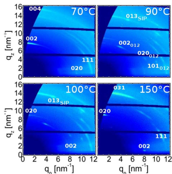
Figure 3: Grazing incidence X-ray diffraction patterns of various samples heat-treated at defined temperatures. Adjacent patterns share axis for sake of comparability.
