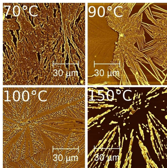
Figure 1: AFM height images of individual phenytoin thin films after heat treatment at various temperatures for two hours, respectively, in an oven.
