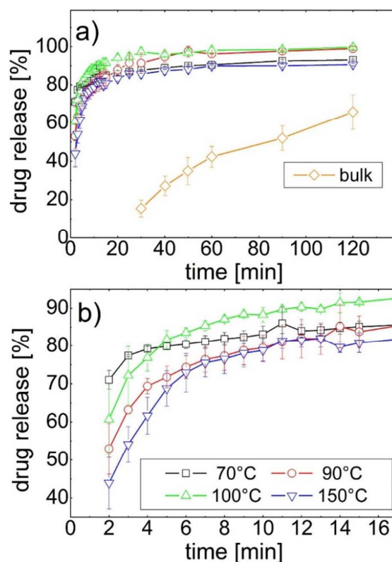
Figure 4: Drug release as function of time for samples prepared at various temperatures (a). (The bulk powder shows not significant value before 30 minutes.) The same data zoomed for the initial release region (b).
