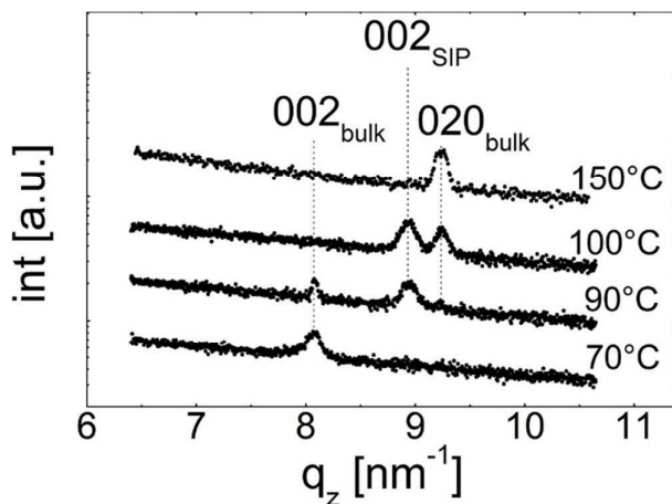
Figure 2: Specular X-ray diffraction scans of phenytoin samples heat treated at various temperatures.
