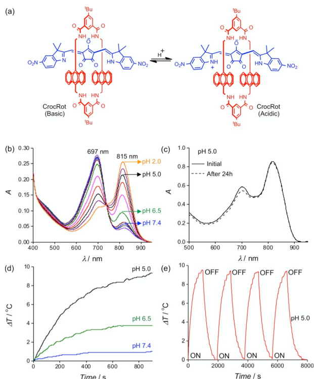
Figure 2. (a) pH sensitive croconaine rotaxane (CrocRot). (b) UV/Vis absorption of CrocRot-SL at various pH values, [CrocRot] = 3 \mu M. (c) UV/Vis absorption plots of CrocRot-SL in buffer at pH 5.0, acquired initially (solid line) and after standing for 24 hour (dashed line) at 4°C. (d) Temperature changes during laser irradiation (808 nm, 3.5 W/cm 2 ) of CrocRot-SL samples at different pH values. (e) Multiple heating cycles of CrocRot-SL at pH 5.0 due to periodic laser irradiation (808 nm).
