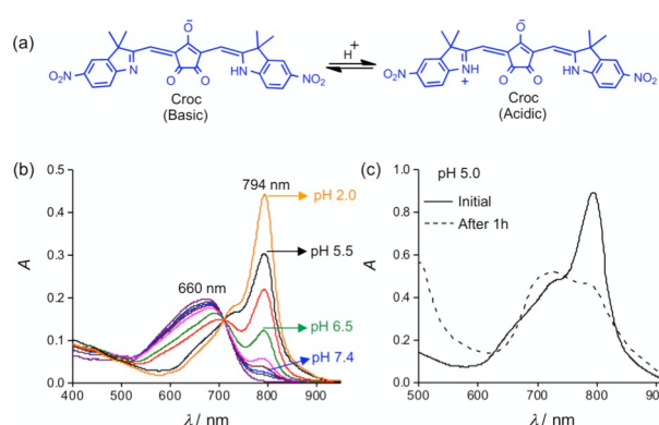
Figure 1. (a) pH sensitive croconaine (Croc). (b) UV/Vis absorption of Croc-SL in buffer at various pH values, [Croc] = 3 \mu\text{M} . (c) UV/Vis absorption plots of Croc-SL in buffer at pH 5.0, spectra were acquired initially (solid line) and after standing for 1 hour (dashed line) at 4°C.
