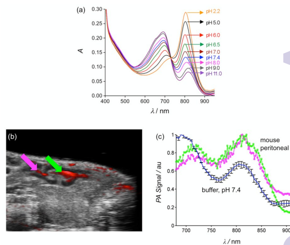
Figure 4. (a) UV/ Vis absorption spectra of CrocRot-IVSL at various pH values, [CrocRot] = 3 \mu\text{M} . (b) Cross-sectional B mode ultrasound image (sagittal plane) of living mouse abdomen (grayscale), co-registered with the photoacoustic response at 740 nm; magenta and green arrows denote two ROIs of CrocRot-IVSL accumulation within peritoneal cavity (c) Photoacoustic spectra of CrocRot-IVSL in buffer pH 7.4 before injection (blue/black trace) and in the two ROIs within the mouse peritoneal cavity (magenta and green).
