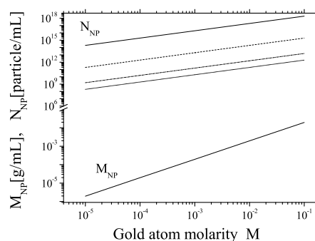
Fig. 1 The mass M_{NP} and the number N_{NP} of gold nanoparticles per unit volume as a function of the gold atom molarity M , for different values of the particle radius r . (full line): 1 nm; (dash line): 10 nm; (dash-dot line): 50 nm; (dotted line): 100 nm.
