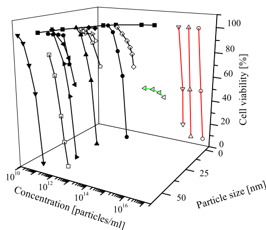
Fig. 5 Viability of HeLa cells incubated with gold nanoparticles of different size and at different concentrations (expressed as nanoparticle per ml). The particles are differently funzionalized. Data taken from Refs: (blacksquare): Ref. 22 ; (bullet): Ref. 23 ; (blacktriangle): Ref. 23 ; (blacktriangledown): Ref. 23 ; (blacklozenge): Ref. 24 ; (blacktriangleleft): Ref. 25 ; (blacktriangleright): Ref. 25 ; (boxdot): Ref. 26 ; (square): Ref. 26 ; (bigcirc): Ref. 27 ; (bigtriangleup): Ref. 27 ; (bigtriangledown): Ref. 27 ; (triangleleft): Ref. 28 ; (triangleright): Ref. 18 ; (lozenge): Ref. 29 .
