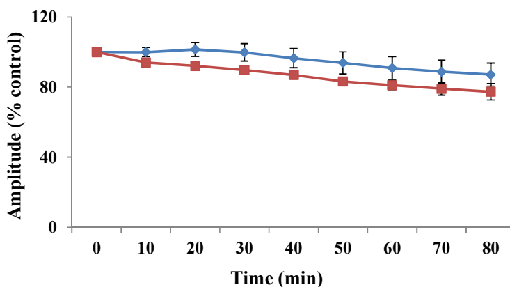
Figure 4. The difference in the change of nCAP amplitude of the sciatic nerve after treatment with 1 mM of (blue) free cisplatin ( p = 0.3 ) and (red) cisplatin@CB[7] ( p = 0.1 ).
