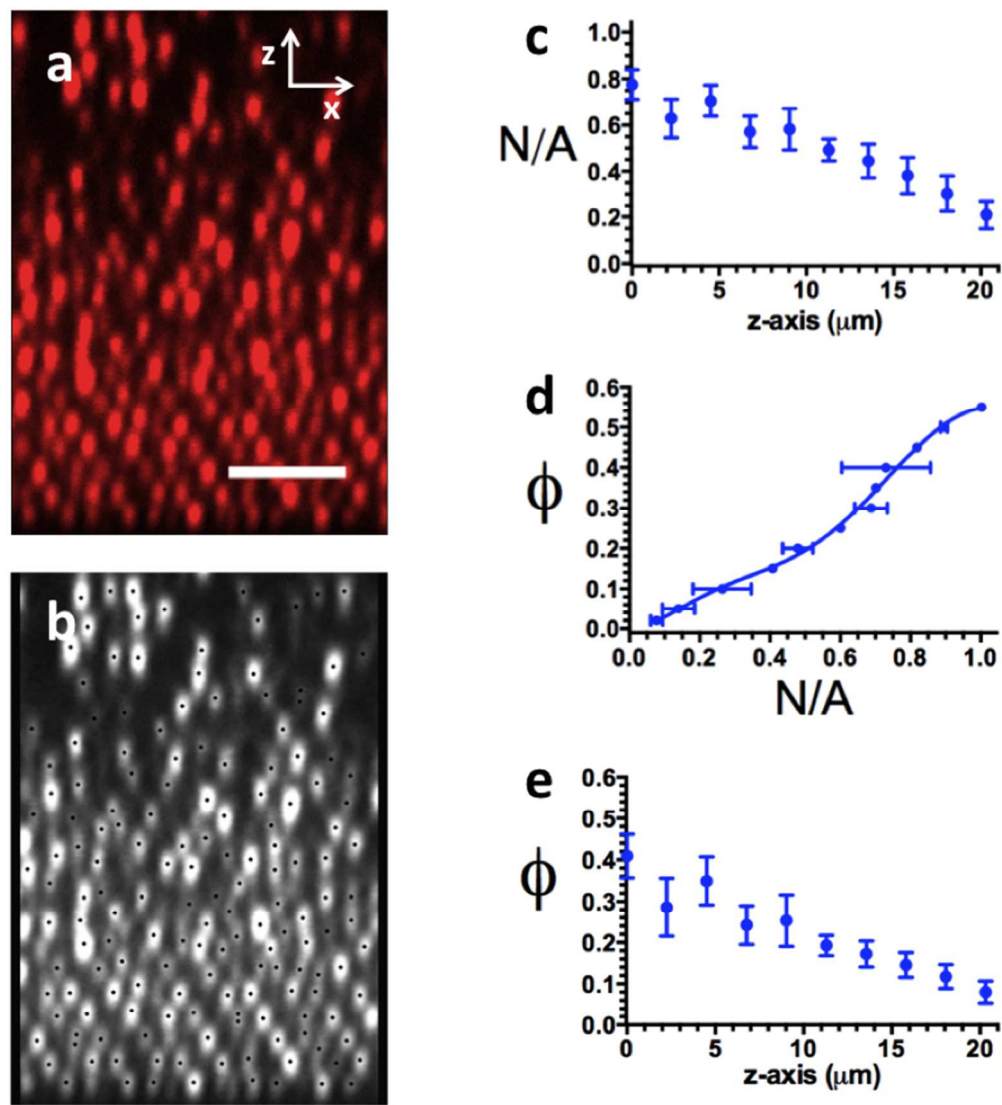
Figure 2. Determination \phi(z) from 2D CLSM images. a) Raw 2D CLSM image and b) particle centroids identified from it by image analysis. c) Particle number density in number of particles/ \mu\text{m}^2 ( N/A ) is plotted vs distance along the discretized z-axis, where z = 0 corresponds to the electrode surface. d) Calibration of N/A to \phi was fit with a polynomial function from which \phi(z) was determined and plotted in (e). Scale bar is 5 \mu\text{m} .
