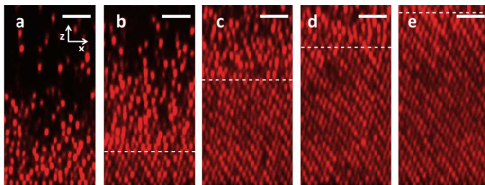
Figure 9. Propagation of crystallinity at Pe = 0.22 a) after 30 minutes of deposition; b) after 1 hour of deposition; c) 2 hours; d) 2.5 hours; e) 3 hours. The time-dependent location of the crystal front ( h_{\text{front}} ) is indicated.
