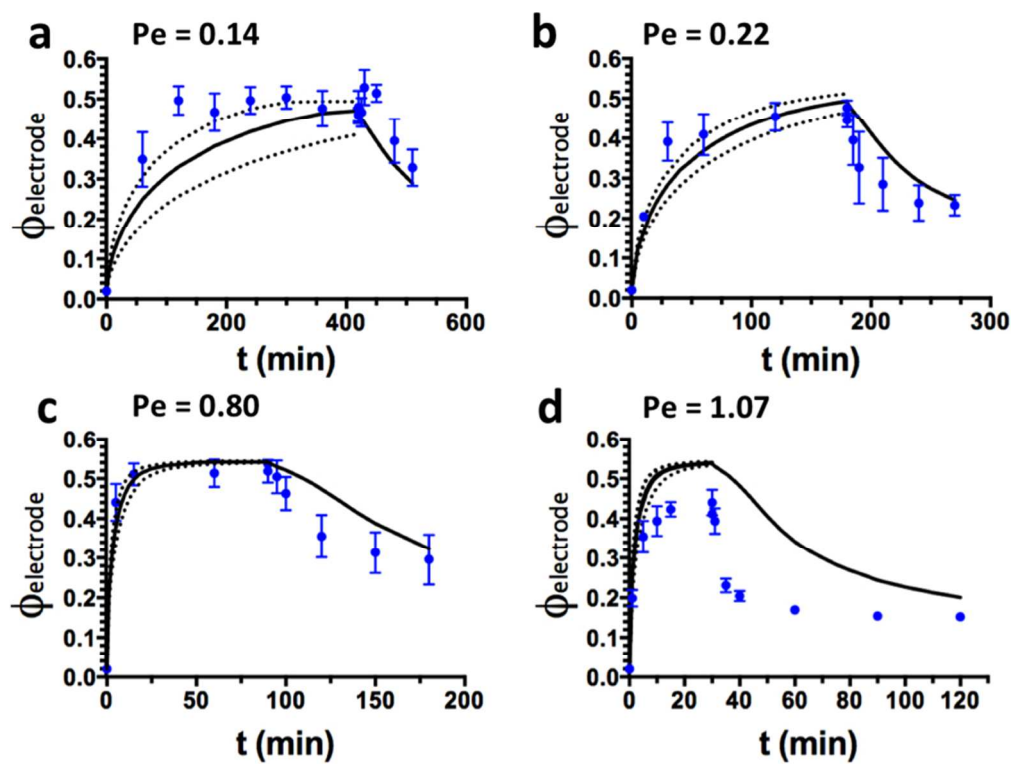
Figure 5. Electrode volume fraction, \phi_{\text{electrode}} , as a function of time for a) Pe = 0.14 b) Pe = 0.22 c) Pe = 0.80 and d) Pe = 1.07 . Data points are measured values and curves are solutions to eqn (1). Dotted curves are model solutions for a standard deviation above and below the measured colloidal velocity in the steady electric field, U_0 .
