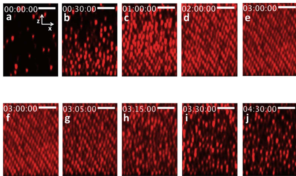
Figure 4. CLSM images of DC electric field-assisted colloidal assembly at Pe = 0.22 (a-e) and subsequent relaxation of this structure upon removal of the field (f-j). a) just prior to application of the steady field; b) 30 minutes after application; c) 1 hour; d) 2 hours ;e) 3 hours. f) relaxation at the moment of field removal; g) 5 minutes after removal of field; h) 15 minutes; i) 30 minutes; j) 90 minutes. Scale bar is 5\ \mu\text{m} .
