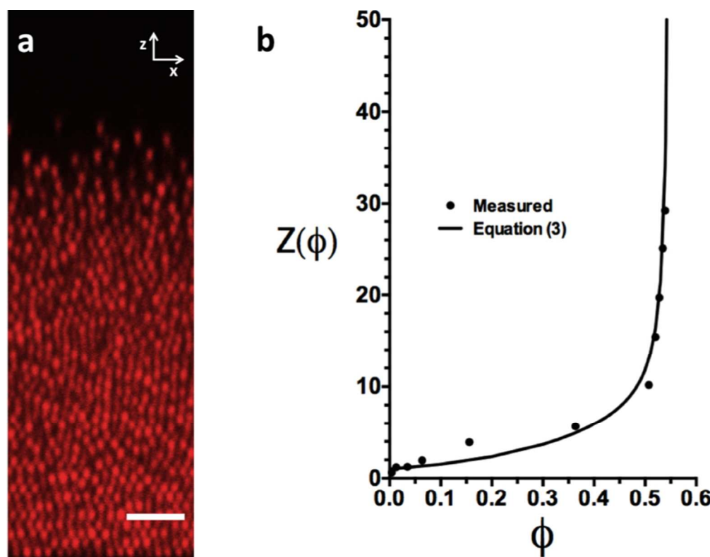
Figure 3. Z(\phi) from steady-state profile of \phi(z) . a) PMMA spheres at \phi_0 = 0.01 were deposited in a steady ( E = 340 V/m) until a steady state in \phi(z,t) was achieved. Scale bar is 5\ \mu\text{m} . Eqn (2) was applied to these data to obtain \Pi(z) , which is plotted as Z(\phi) in b. The curve is the fit to eqn (3) with parameters as given in the text.
