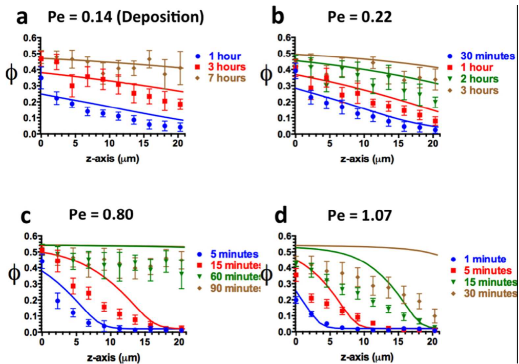
Figure 7. \phi(z,t) during deposition at a) Pe = 0.14 b) Pe = 0.22 c) Pe = 0.80 and d) Pe = 1.07 . The curves are solutions to eqn (1).
