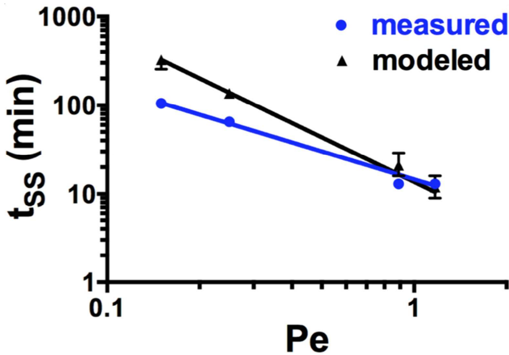
Figure 6. Characteristic times of deposition ( t_{SS} ) as a function of Pe . t_{SS} is the time needed for \phi_{\text{electrode}} to reach 95% of its final value during deposition, as assessed from the results of Fig. 5. Blue data points are characteristic times for measurements, black data points are characteristic times for modeling. The curves are power laws: t_{SS}(Pe) = 13.5 \times Pe^{-1.091} for the measurements and, t_{SS}(Pe) = 16.2 \times Pe^{-1.568} for the model.
