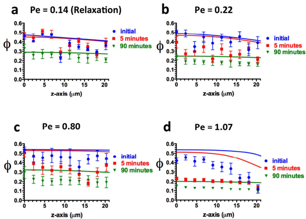
Figure 8. \phi(z,t) during relaxation at a) Pe = 0.14 b) Pe = 0.22 c) Pe = 0.80 and d) Pe = 1.07 . The curves are solutions to eqn (1).
