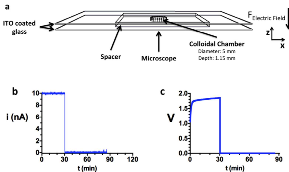
Figure 1. a) Schematic of device used to apply DC electric fields to initially uniform suspensions of colloidal spheres. The device, developed by Shah et al., 3 has an electrode gap of 1.15 mm. b) current vs time and c) voltage vs time plots for a galvanostatic electric field applied from 0-30 minutes and then removed from 30-90 minutes.
