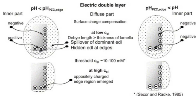
Figure 3 Schematic representation of the electrical double layers (edl) around montmorillonite platelets under different solution conditions, reproduced from Tombacz and Szekeres 30 after Secor & Radke 29 .
