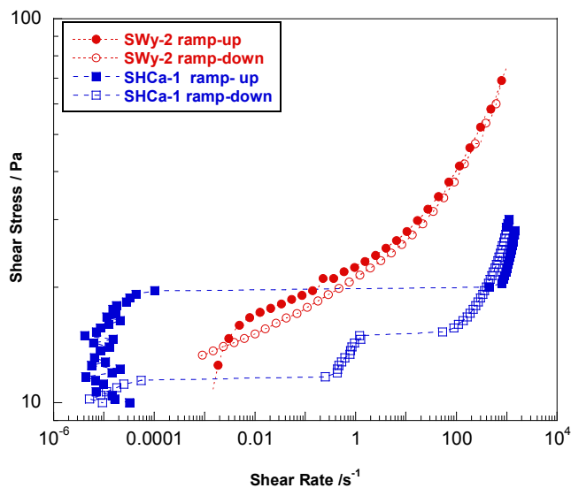
Figure 10 Controlled-stress shear flow curves for 2.8 wt% hectorite SHCa-1 and 3.2 wt% montmorillonite SWy-2 suspensions at c > c^* . Redrawn from data of Ten Brinke et al. and Bailey et al. 89, 110 .
