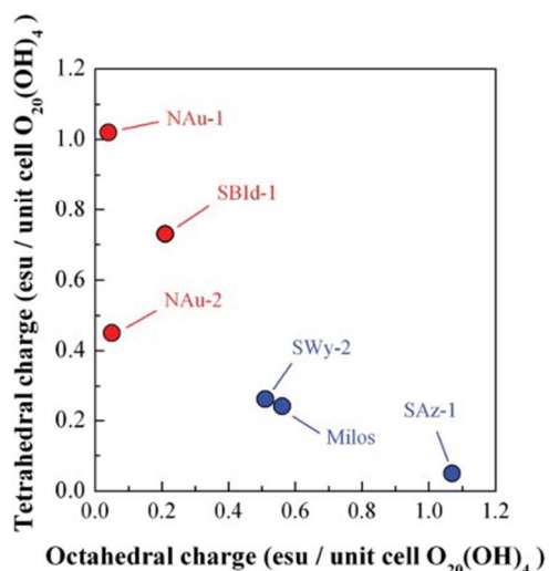
Figure 2. Comparison of the charge location (tetrahedral versus octahedral) for different smectite clays: nontronites: NAu-1 and NAu-2 (Australia); beidellite: SBI-d-1 (Idaho, USA); montmorillonites: SWy-2 (Wyoming, USA), SAz-1 (Arizona, USA), Milos (Greece). Reproduced with permission from Paineau et al. 27 .
