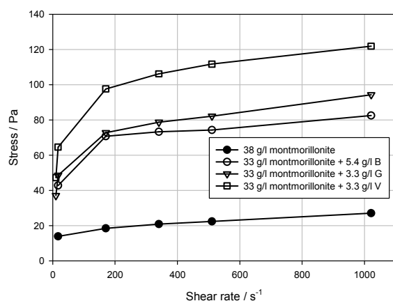
Figure 18 Shear stress shear rate flow curves for suspensions of montmorillonite (bentonite) and montmorillonite–MMH (V) in fresh water, compared with montmorillonite–gibbsite (G) and montmorillonite–boehmite (B) in 15 g/L NaCl. Redrawn from van der Kooij et al. 152
