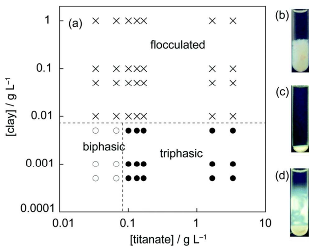
Figure 20 (a) Phase diagram of the titanate-clay binary nanosheet colloids, and typical appearances of the (b) flocculated, (c) isotropic-LC biphasic, and (d) isotropic-LC-LC triphasic samples between crossed polarizers. Symbols embedded in the diagram indicate experimentally examined composition. Reproduced from Nakato et al. 175
