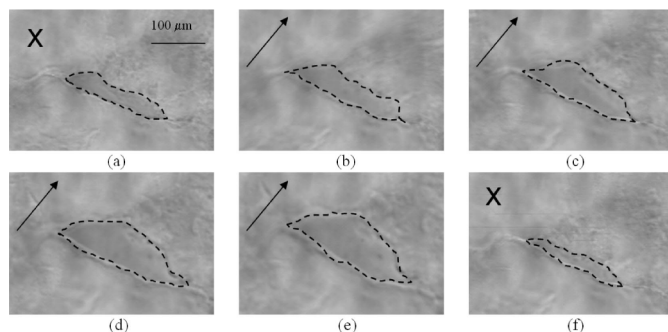
Figure 15 Observations by optical microscopy of a mixture of laponite and maghemite ( \Phi_{\text{mag}} 0.8%, \Phi_{\text{lap}} 0.38%). (a) A sample at rest 2500 h after synthesis of the mixture. (b-e) Sample under the application of a magnetic field gradient; the pictures are taken at intervals of 1.5 s. (f) Sample at rest after the application of a magnetic field gradient. Reproduced with permission from Cousin et al. 144 . Copyright 2008 American Chemical Society.
