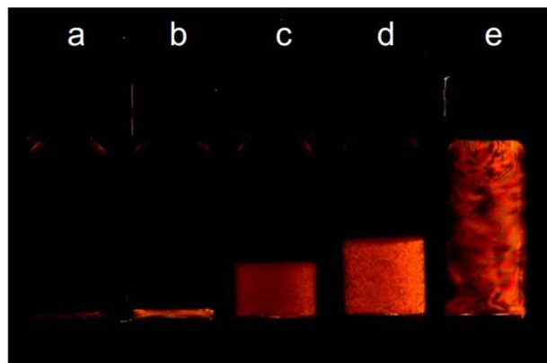
Figure 9. Aqueous suspensions of nontronite clay NAU-2 observed between cross-polarisers, showing increasing Nematic liquid crystal phases volume for clay volume fractions range from 0.5% (a) to 0.72% (d). Sample (e) is a birefringent gel with a volume fraction of 1%. Reproduced with permission from Michot et al. 21 . Copyright (2006) National Academy of Sciences, U.S.A.
