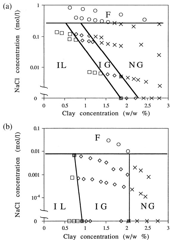
Figure 7 (a) State diagram of the bentonite suspensions versus clay and NaCl concentrations. (o, F) Flocculated; ( \square , IL) isotropic liquid; ( \diamond , IG) isotropic gel; ( \times , NG) nematic gel. (b) Phase diagram of the laponite suspensions versus clay and NaCl concentrations. (o, F) Flocculated; ( \square , IL) isotropic liquid; ( \diamond , IG) isotropic gel; ( \times , NG) nematic gel. Reproduced with permission from Gabriel et al. 18 , Copyright 1996 American Chemical Society.
