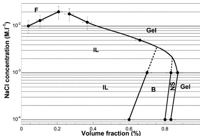
Figure 8 Phase diagram of sodium nontronite suspensions. Upon increasing volume fraction, the suspensions first form an isotropic liquid (IL), then enter a biphasic regime (B) followed by a small region of nematic sol (NS), and finally form birefringent gels. The line between gel and liquid was determined by oscillatory shear measurements. At high salt concentration, the presence of flocs (F) was checked out by visual observation. Reproduced with permission from Michot et al. 21 . Copyright (2006) National Academy of Sciences, U.S.A.
