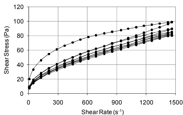
Figure 11 Shear-stress shear-rate flow curves for montmorillonite suspensions illustrating the dependence of thixotropy on shear history. A preconditioned sample was transferred into the measurement geometry and left at rest for 10 minutes. The shear rate was ramped up then down over the range 11.6-1460 s^{-1} repeatedly for a total of 5 cycles. The total ramp time was 48 min in each direction. The first cycle, the upper loop, shows a breakdown of structure in the gelled suspension which is not fully recovered during the ramp-down. Successive up-down flow curves continue to reduce the level of structure in the suspension and shrink the area of the hysteresis loop until the up and down curves are essentially identical, and two successive loops superimpose in the equilibrium flow curve. Under such conditions, the sample has sufficient time to relax to a steady-state condition at each shear rate and all trace of previous stress history has been removed. Reproduced with permission from Tehrani and Popplestone 115 .
