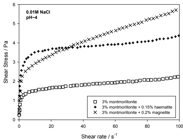
Figure 12 Flow curves for aqueous montmorillonite clay and iron oxide suspensions with different compositions at pH 4 and low salt concentration. (% = wt/wt% concentration) Redrawn from Tombacz et al. 146
