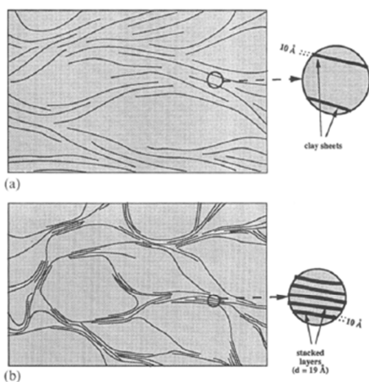
Figure 5. Schematic representation of the structure of smectite gel a) dispersed in fresh water and b) effect on the structure of addition of salt. Reproduced from Morvan et al. 81
