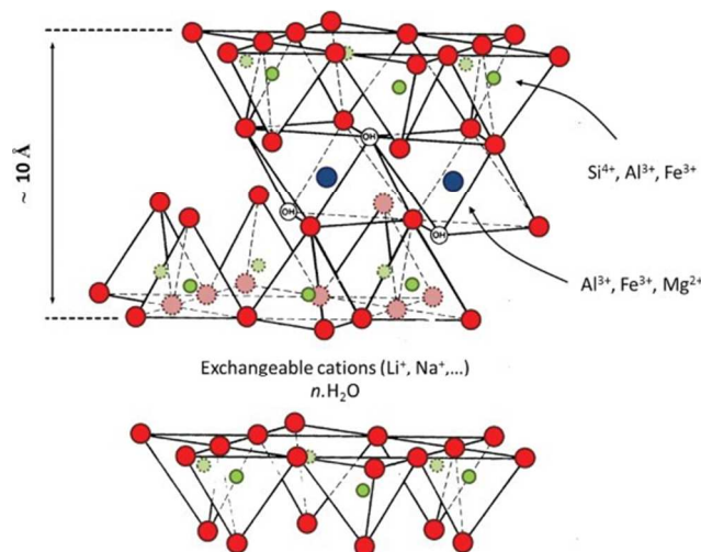
Figure 1 Crystal structure of a dioctahedral smectite nanosheet (Reproduced with permission from Paineau et al. 27 , after Grimm 28 ).
