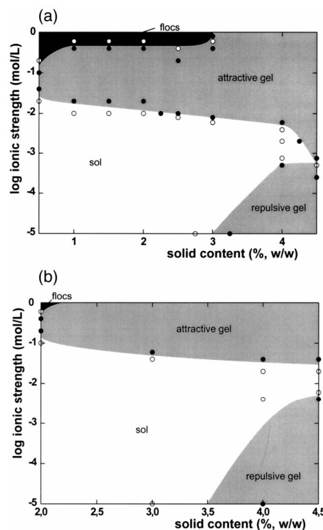
Figure 6. Sol-gel state diagrams for two sodium montmorillonites and NaCl. a) Turkey M50, b) Wyoming M40A. Reproduced from Abend & Lagaly 19 .
