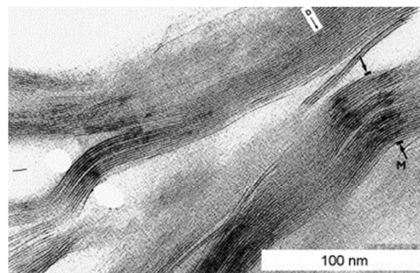
Figure 4 TEM image of a purified natural montmorillonite dispersed in water. Reproduced from Pellenq and Van Damme 70 .
