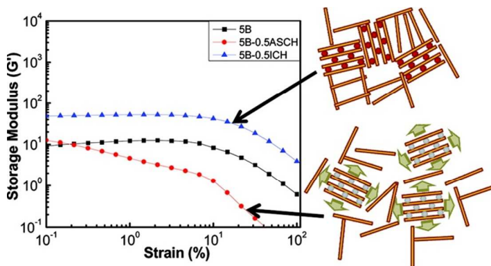
Figure 19 Storage modulus as function of strain for aqueous suspensions of 5 wt% montmorillonite (5B), 5 wt% montmorillonite + 0.5 wt% alumina-silica clay hybrid (5B-0.5ASCH) and 5 wt% montmorillonite + 0.5 wt% iron oxide nanoparticle clay hybrid (5B-0.5ICH). Reproduced by permission from Jung et al. 136 . Copyright 2011 American Society of Chemistry.
