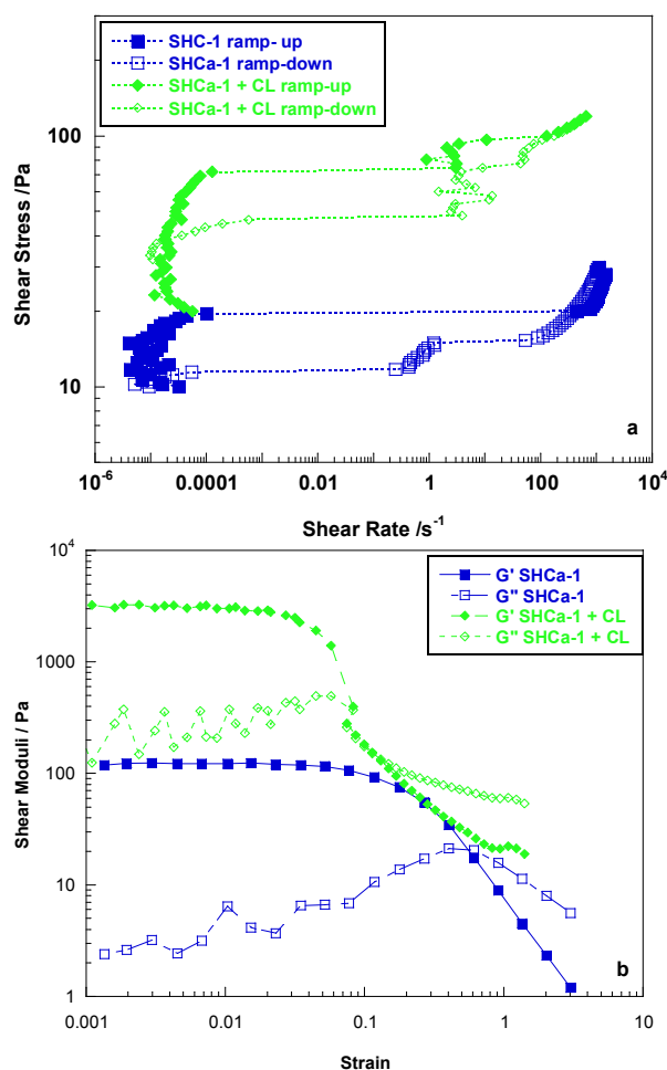
Figure 13 (a) Controlled-stress continuous shear rheology for 2.8 wt% hectorite suspensions ( \square ) and 2.8 wt% hectorite + 0.25 wt% Ludox CL ( \diamond ). Filled symbols: shear stress increasing; open symbols: shear stress decreasing. (b) strain dependence at 1 Hz for storage and loss moduli for 2.8 wt% hectorite suspensions ( \square ) and 2.8 wt% hectorite + 0.25 wt% Ludox CL ( \diamond ). Redrawn from Ten Brinke et al. 110 with permission.
