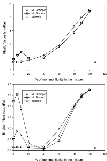
Figure 16 Effect of montmorillonite concentration on plastic viscosity (a) and Bingham yield value (b) of mixed suspensions of Na-saturated polygorskite and montmorillonite at a total clay concentration of 3% w/v and pH 7. Redrawn with permission from Neaman & Singer 153 .
