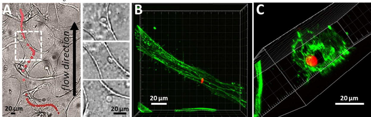
Fig. 7 (A) Trajectory of a colloidal disc ( d = 10 \mu\text{m} , h = 1 \mu\text{m} ) through the microvascular network grown on a multiculture microfluidic device. The black arrow indicates the general direction flow driven by a small hydrostatic pressure difference across the network. The discs assume different orientations during their passage (center panel). The close-ups also show that they do not adhere to the microvessel walls. Confocal micrographs of the longitudinal (B) and the transverse (C) directions of a vessel segment (green) containing a residual particle (red).
