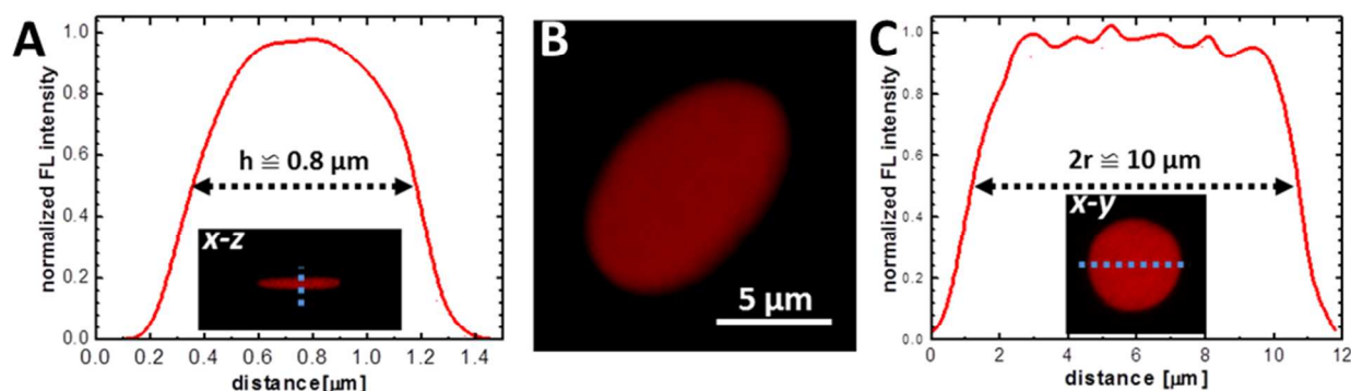
Fig. 5 Laser scanning confocal image of a representative 10 \mu\text{m} disc synthesized using 9.5% \text{O}_2 (B). Normalized fluorescence intensity profiles taken across the x-z (A, blue dotted line) and x-y (C, blue dotted line) planes of the particle. Particle height is estimated to be \sim 0.8 \pm 0.1 \mu\text{m} . Full width at half-maximum (FWHM), as indicated black dotted lines, was used to define the particle boundaries.
