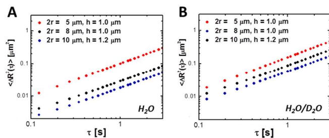
Fig. 6 Mean-square displacement ( \Delta R^2 ) near a wall as a function of lag time, \tau for various colloidal discs in (A) water and (B) a mixture of deuterium oxide and water (9:1 ratio by volume).
