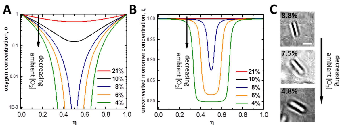
Fig. 3 Steady state profiles of oxygen ( \theta ) and unconverted monomer concentration ( \xi ) as a function of non-dimensionalized channel height ( \eta ). The results shown in A) and B) were obtained by numerically integrating eqn 6 and 7 using the parameter values listed in Table 1 for a range of ambient oxygen concentrations. Decreasing ambient \text{O}_2 concentration leads to a reduction in oxygen penetration depth near the channel walls, where rapid oxygen diffusion prevents particle formation. Cross-linked structures start to grow from the channel center as \theta and \xi fall below a critical threshold value ( \theta_c \sim 10^{-3} , \xi_c = 0.98 ) for gelation. Modulating the chamber [\text{O}_2] allows particle height to approach the sub-micron regime. C) A series of bright-field micrographs showing the change in height of 10 \mu\text{m} diameter discs for a range of chamber [\text{O}_2] (noted in the upper left corner). Above \sim 10\% , no particles can be made, in agreement with model predictions. Scale bar is 5 \mu\text{m} .
