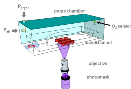
Fig. 1 Experimental setup. Schematic drawing showing the fabrication of an array of colloidal discs ( h \sim 1\ \mu\text{m} , d < 10\ \mu\text{m} ) under reduced oxygen atmosphere. A PEG-based prepolymer is flowed through a tiered PDMS synthesis device and polymerized via controlled pulses of mask-defined UV light through a microscope objective. The gel particles are then advected downstream for collection. The synthesis device is placed in a custom-made purge chamber, which allows the exchange of an air/argon mixture to control the overall ambient oxygen concentration. A RedEye ™ oxygen sensor patch is mounted above the gas outlet to measure the oxygen concentration.
