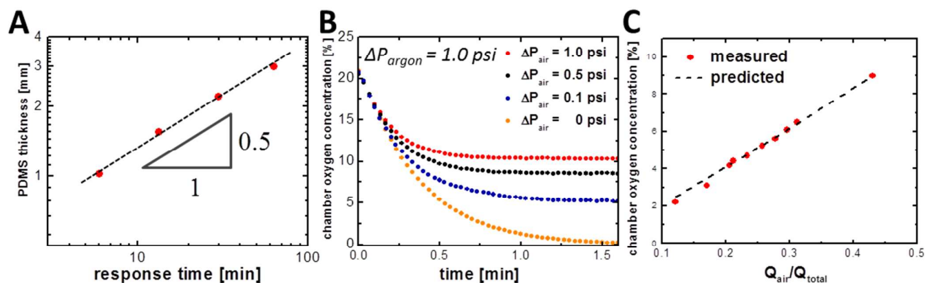
Fig. 2 Timescale comparison. A) Thickness of the PDMS synthesis device determines the threshold response time (defined as the duration of continuous gas purge needed to reach equilibrium). The measured response time obeys a power-law trend, with exponent of 0.5 (a dashed line is drawn to guide the eye), which suggests a simple diffusion-based mechanism, with a characteristic coefficient \sim O(10^{-9}) m 2 /s, typical of oxygen 35 and argon 36 diffusion through porous PDMS. B) The amount of oxygen in the chamber for a range of air feed pressures: 0 psi (orange circles), 0.1 psi (blue circles), 0.5 psi (black circles), 1.0 psi (red circles). Pressure of the argon stream is fixed at 1 psi. Efficient mixing at the gas stream inlets result in short time lags ( < 1.5 min) until a final chamber oxygen concentration plateau is reached. C) Equilibrium oxygen concentration in the purge chamber as a function of volume fraction of air introduced. The empirical measurements (red circles) made using the RedEye TM oxygen sensors are in excellent agreement with a simple model of high Re gas mixing derived from the Blasius correlation (dotted line, eqn 2 in text).
