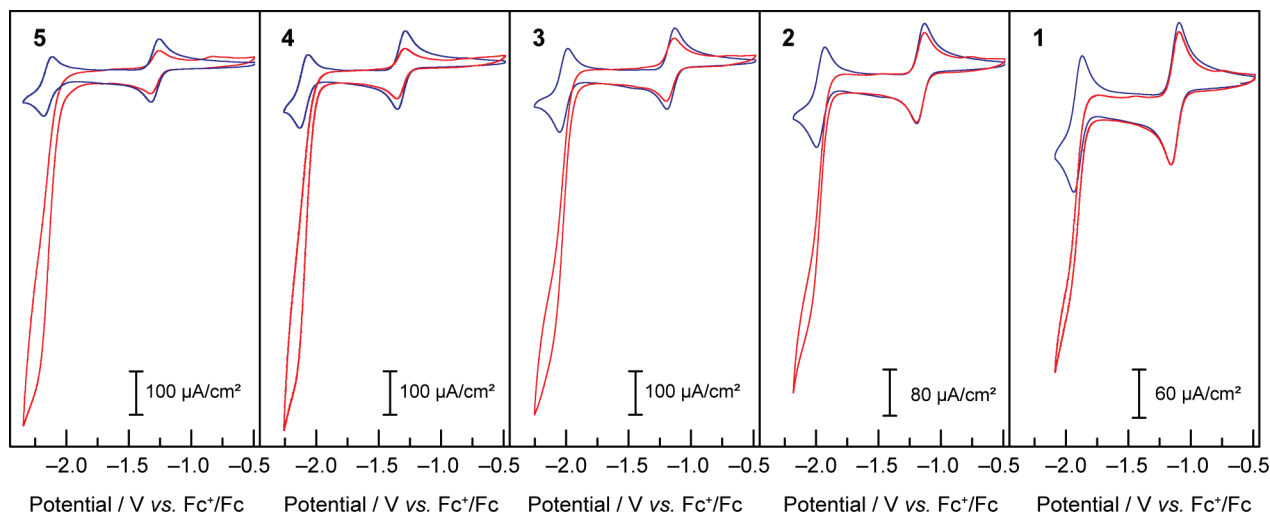
Fig. 6 Cyclic voltammograms under Ar (— blue) and CO 2 (— red) at 50 mV/s of 1 mM solutions of compounds 1-5 in DMF/H 2 O (95:5), TBAPF 6 0.1M
