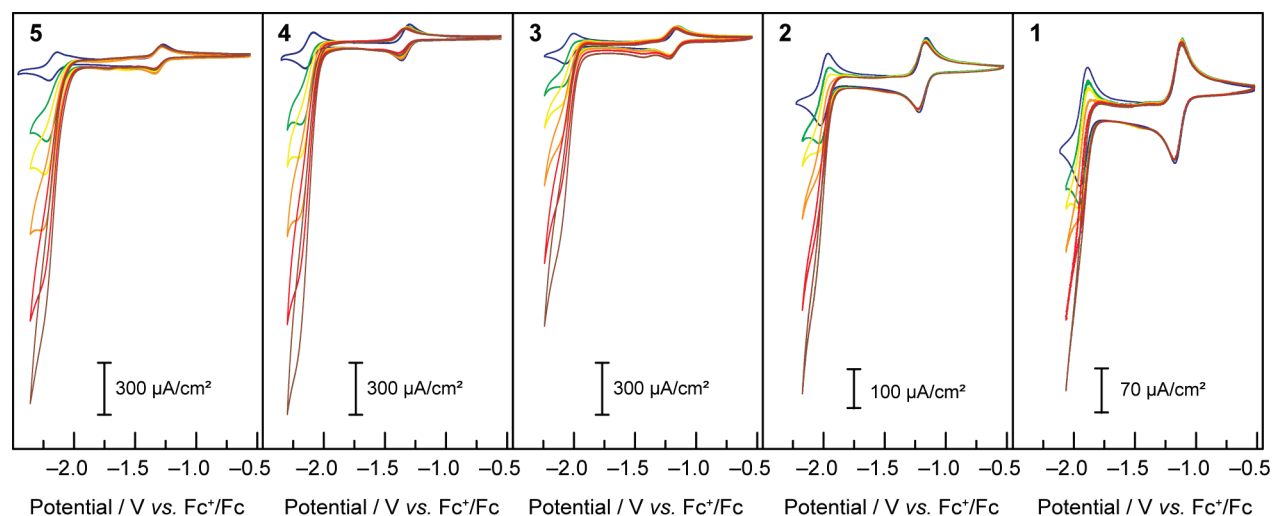
Fig. 2 Cyclic voltammograms under Ar at 50 mV/s of 1 mM solutions of compounds 1-5 in DMF, TBAPF 6 0.1M, on a glassy carbon electrode with 0 (— blue), 5 (— green), 10 (— yellow), 20 (— orange), 40 (— red) and 60 (— brown) mM of acetic acid
