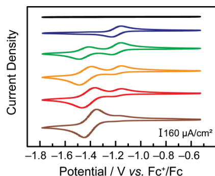
Fig. 3 Cyclic voltammograms under Ar at 100 mV/s in DMF, TBAPF 6 0.1M, on a glassy carbon electrode of a solution of 2 mM tpy (— black) and 2 mM tpy with added 1 mM (— blue), 2 mM (— green), 3 mM (— orange), 4 mM (— red) and 10 mM (— brown) of CoCl 2
