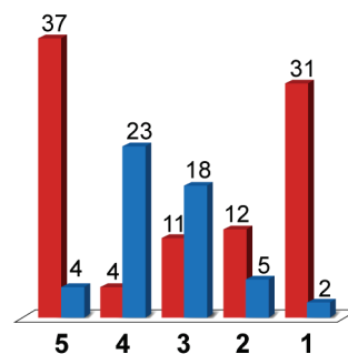
Fig. 7 Faradic yields (in %) for CO (red) and H 2 (blue) during the bulk electrolysis of 1 mM solutions of compounds 1-5 under CO 2 in DMF/H 2 O (95:5), TBAPF 6 0.1M with an applied current of 300 μA during 4h
