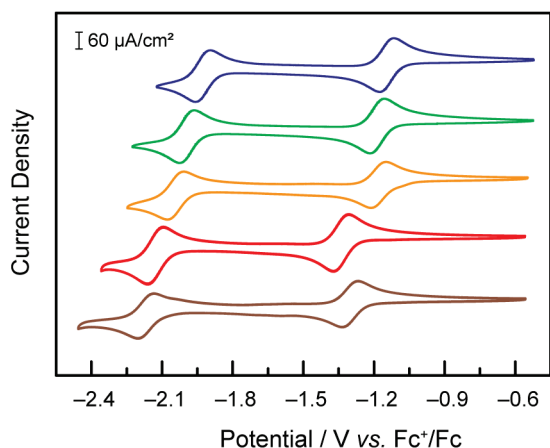
Fig. 1 Cyclic voltammograms under Ar at 50 mV/s of 1 mM solutions of compounds 1 (— blue), 2 (— green), 3 (— orange), 4 (— red) and 5 (— brown) in DMF, TBAPF 6 0.1M, on a glassy carbon electrode
