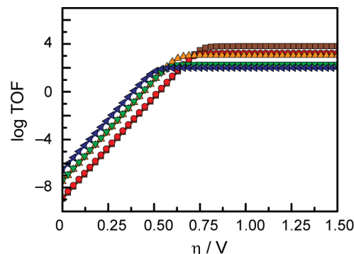
Fig. 5 Catalytic Tafel plot. Turnover frequency for the evolution of hydrogen from 1 M acetic acid in DMF catalysed by 1 (— blue), 2 (— green), 3 (— orange), 4 (— red) and 5 (— brown) as a function of overpotential
