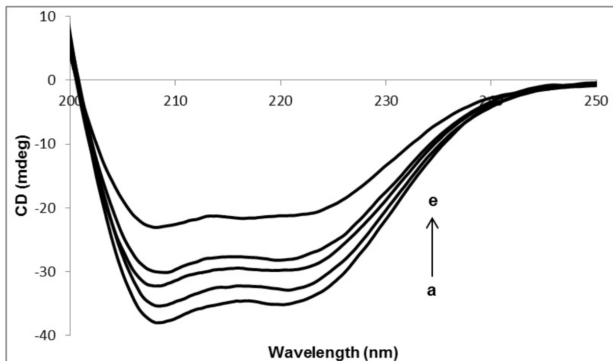
Figure 4. CD spectra of HSA in the presence of various concentrations of PG. [HSA] = 3 \times 10^{-6} M. ( r_i = ([PG]/[HSA]) = 0.0, 0.33, 1.0, 1.66 and 2.66 ).
