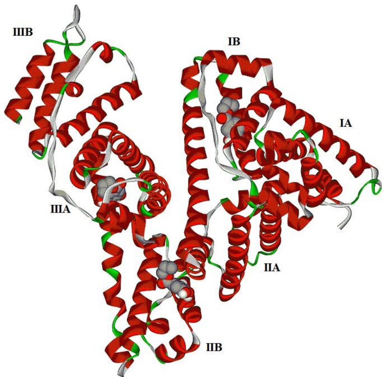
Figure 5. Docking interaction of PG and HSA. PG molecules are shown as CPK and protein is represented as solid ribbon.
