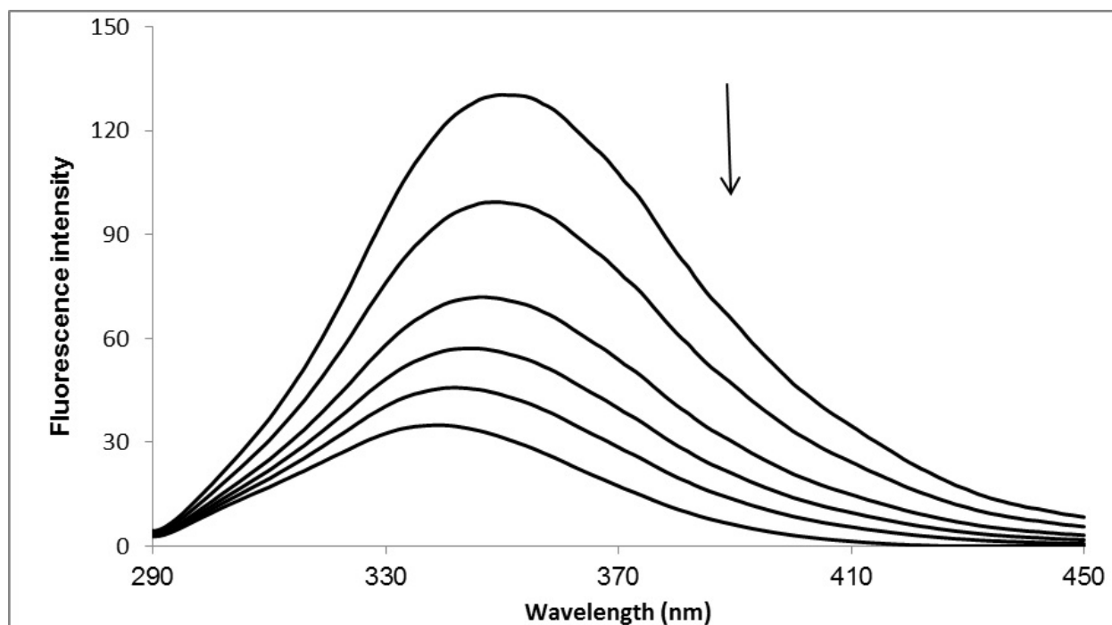
Figure 2. Fluorescence spectra of HSA in the absence or the presence of PG, [HSA] = 3 \times 10^{-5} M and [PG] = 0, 2, 4, 6, 8, 10 \times 10^{-4} M.
