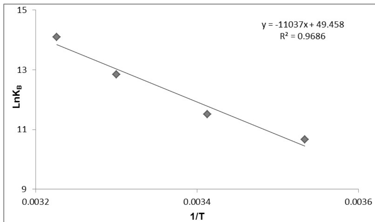
Figure 3. The van't Hoff plot for the interaction of HSA and PG, [\text{HSA}] = 3 \times 10^{-5} \text{ M} ; [\text{PG}] = 0, 2, 4, 6, 8, 10 \times 10^{-4} \text{ M} .
