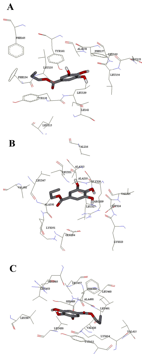
Figure 6. The computational interaction model of A) HSA- subdomains IB; B) HSA- subdomains IIB; C) HSA- subdomains IIIA. The amino acid residues of HSA are represented using lines and PG structure is represented as stick model.
