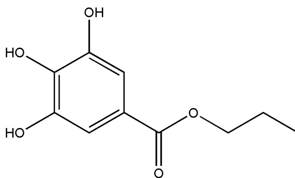
Figure 1. Chemical structure of propyl gallate.
