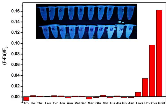
Fig. 4 Fluorescence emission intensity of the N-GQDs-Hg (II) upon addition of different kinds of amino acids. [\text{Hg}^{2+}] = 20 \mu\text{M} , [\text{amino acids}] = 10 \mu\text{M} . Inset shows the fluorescent color of the N-GQDs-Hg (II) complex after adding different kinds of amino acids under UV light ( \lambda_{\text{ex}} = 365 \text{ nm} ).
