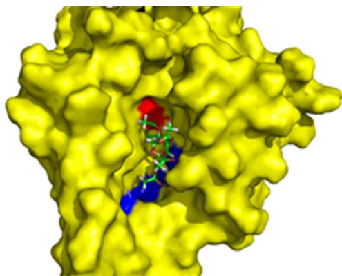
Fig. 3. Top view of the cavity of lipase from P. stutzeri with 1β molecule, with the lids on the sides. In blue, large pocket; small
