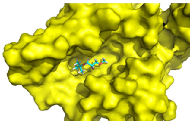
Fig. 5. Top view of the cavity of lipase from P. stutzeri with S6 in the enzyme active center. The solvent has a t -butyl group that avoids the approach of the catalytic residue Ser-109 and therefore can not allow the nucleophilic attack of the alcoholysis reaction.
