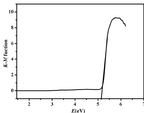
Fig. 1 Kubelka–Munk-transformed diffuse reflectance spectra of ZIF-8.
