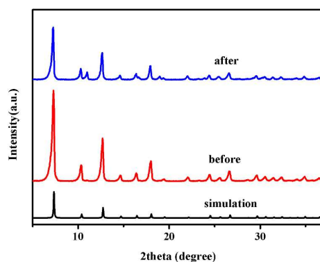
Fig. 7 PXRD patterns of ZIF-8 before and after photocatalytic reaction and the simulated XRD pattern for the ZIF-8 structure created from CIF in reference 52.
