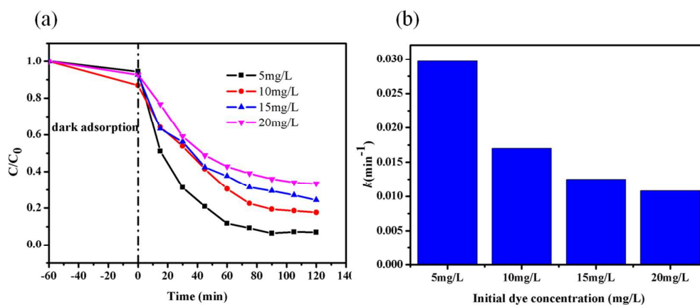
Fig. 4 (a) Effect of initial dye concentration on the degradation of MB. (b) Comparison of the apparent rate constants of the degradation of MB with different initial concentrations.
