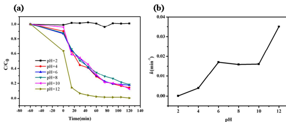
Fig. 5 (a) Effect of initial pH on the degradation of MB. Experimental conditions: ZIF-8, 0.5 g/L; MB, 10 mg/L and UV irradiation. (b) The corresponding pseudo-first-order rate constants for system with pH = 2.0 - 12.0.
