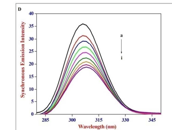
Figure 9. Synchronous emission spectrum of (A) HSA at \Delta\lambda=60 nm, (B) BSA at \Delta\lambda=60 nm, (C) HSA at \Delta\lambda=15 nm and (D) BSA at \Delta\lambda=15 nm at various AZA concentrations.
