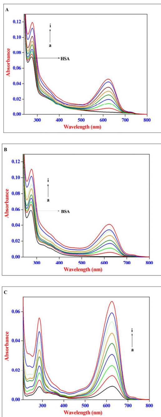
Figure 2. Absorption spectra of (A) HSA ( 1.0 \times 10^{-6} \text{ mol dm}^{-3} ), (B) BSA ( 1.0 \times 10^{-6} \text{ mol dm}^{-3} ) in the absence and presence of AZA. (C) AZA alone. Conditions: [AZA]: (a) 0, (b) 2.00 \times 10^{-7} , (c) 4.00 \times 10^{-7} , (d) 6.00 \times 10^{-7} , (e) 8.00 \times 10^{-7} , (f) 10.00 \times 10^{-7} , (g) 12.00 \times 10^{-7} , (h) 14.00 \times 10^{-7} and (i) 16.00 \times 10^{-7} \text{ mol dm}^{-3} . c[\text{HSA}] = c[\text{BSA}] = 1.00 \times 10^{-6} \text{ mol dm}^{-3} .
