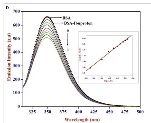
Figure 7. Emission spectra of (A) HSA-Phenylbutazone, (B) BSA-Phenylbutazone, (C) HSA-Ibuprofen and (D) BSA-Ibuprofen [1:1] at various AZA concentrations. [AZA]: (a) 0, (b) 2.00 \times 10^{-7} , (c) 4.00 \times 10^{-7} , (d) 6.00 \times 10^{-7} , (e) 8.00 \times 10^{-7} , (f) 10.00 \times 10^{-7} , (g) 12.00 \times 10^{-7} , (h) 14.00 \times 10^{-7} and (i) 16.00 \times 10^{-7} mol dm -3 . Inset shows the respective double logarithmic plot.
