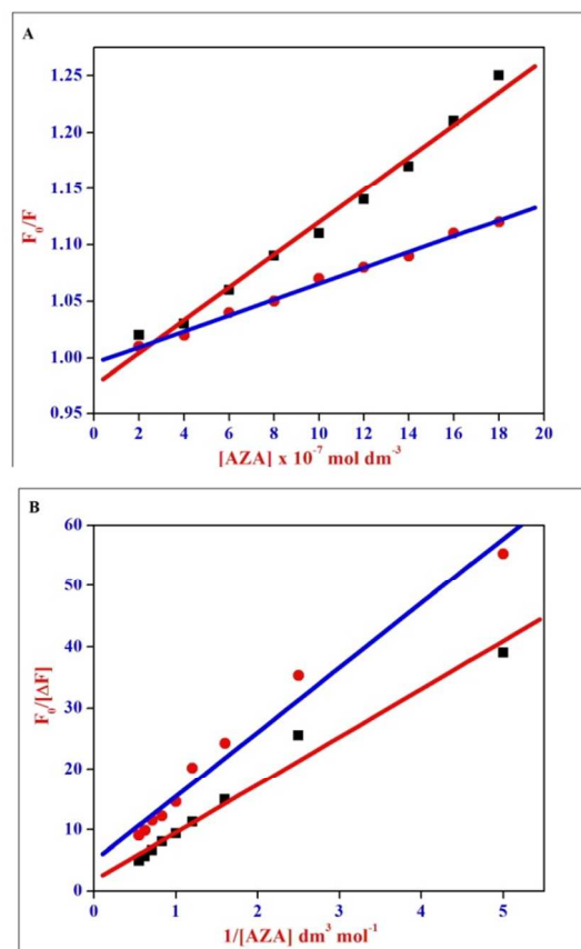
Figure 4. (A) Stern-Volmer and (B) Modified Stern-Volmer plot for HSA-AZA (●) and BSA-AZA (■) complexes.
