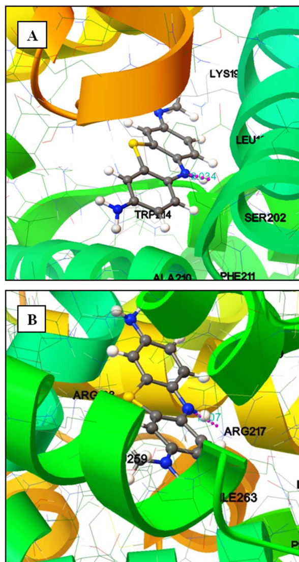
Figure 12. (A) Molecular docking of HSA-AZA complex. (B) Molecular docking of BSA-AZA complex. Hydrogen bond is shown in pink dotted line.
