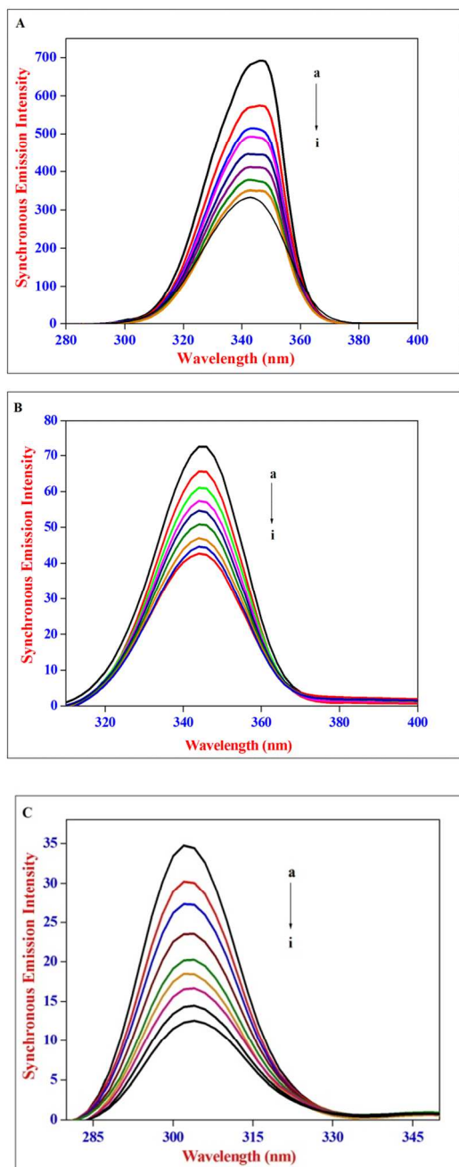
Figure 9. Synchronous emission spectrum of (A) HSA at \Delta\lambda=60 nm, (B) BSA at \Delta\lambda=60 nm, (C) HSA at \Delta\lambda=15 nm and (D) BSA at \Delta\lambda=15 nm at various AZA concentrations.
