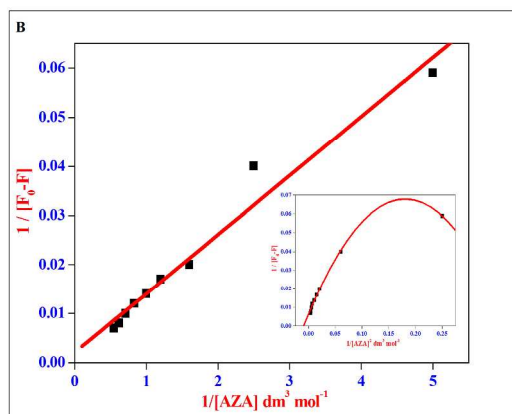
Figure 5. Benesi-Hildebrand plot of 1/[F_0-F] vs 1/[AZA] for binding of AZA with (A) HSA and (B) BSA. Inset shows the modified Benesi-Hildebrand plot of 1/[F_0-F] vs 1/[AZA]^2 for HSA/BSA-AZA systems.
