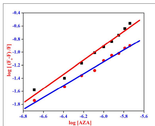
Figure 6. Double logarithmic plot for HSA-AZA (●) and BSA-AZA complexes (■).
