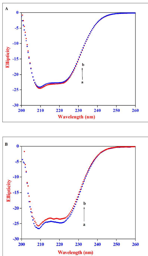
Figure 10. CD spectra of (A) HSA and (B) BSA in the absence and presence of AZA. Conditions: [HSA] = [BSA] = 2.0 \times 10^{-6} mol dm ^{-3} ; [AZA]: (a) 0 \times 10^{-6} mol dm ^{-3} and (b) 2.0 \times 10^{-6} mol dm ^{-3} .
