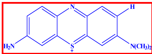
Scheme. 1. Structure of Azure A
