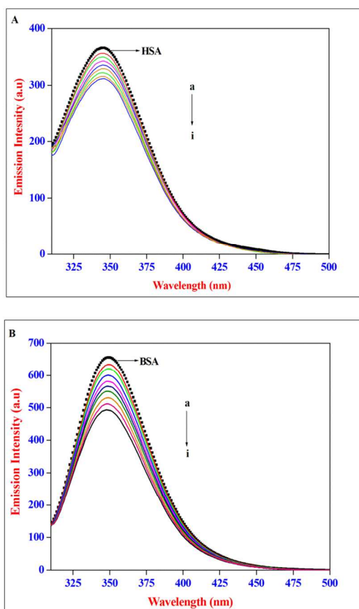
Figure 1. Emission spectra of (A) HSA ( 1.00 \times 10^{-6} mol \text{dm}^{-3} ) and (B) BSA ( 1.00 \times 10^{-6} mol \text{dm}^{-3} ) at various AZA concentrations. [AZA]: (a) 0, (b) 2.00 \times 10^{-7} , (c) 4.00 \times 10^{-7} , (d) 6.00 \times 10^{-7} , (e) 8.00 \times 10^{-7} , (f) 10.00 \times 10^{-7} , (g) 12.00 \times 10^{-7} , (h) 14.00 \times 10^{-7} and (i) 16.00 \times 10^{-7} mol \text{dm}^{-3} .
