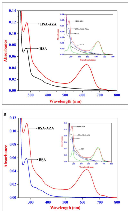
Figure 8. Absorption spectra of (A) HSA alone and HSA-AZA complex; (B) BSA alone and BSA-AZA complex. Conditions: c[\text{HSA}] = c[\text{BSA}] = 1.0 \times 10^{-6} \text{ mol dm}^{-3} ; c[\text{AZA}] = 1.0 \times 10^{-6} \text{ mol dm}^{-3} . Inset shows the difference absorption spectra of HSA/BSA:AZA [1:1] complex and AZA.
