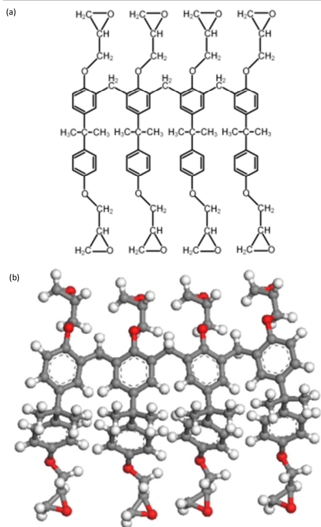
Fig. 1 Epoxy monomer of SU-8 photoresist: (a) Chemical structure. (b) Molecular model.
