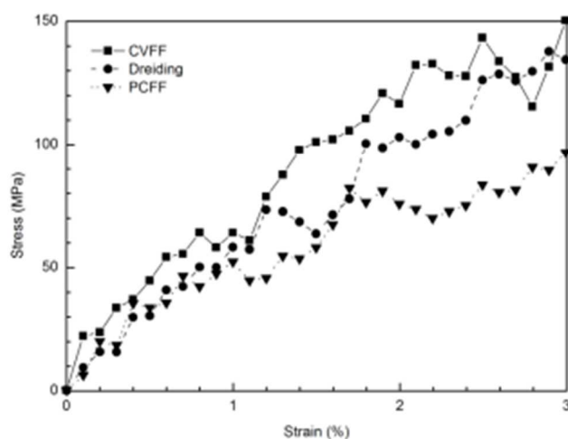
Fig. 6 Stress-strain curves obtained at tensile deformation of cross-linked SU-8 photoresist at three forcefields.
