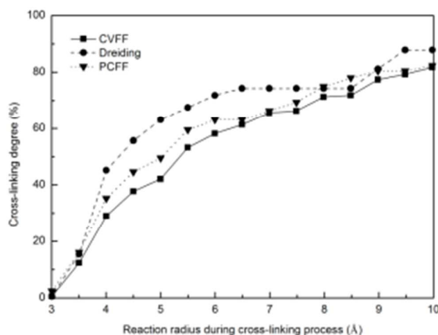
Fig. 5 Cross-linking degree of SU-8 photoresist as a function of reaction radius under different potentials.
