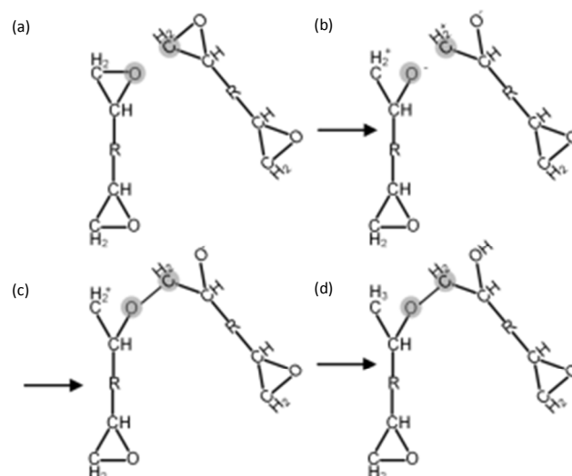
Fig. 3 Procedures of cross-linking process: (a) Reactive atoms located inside the reaction radius are recognized (marked with filled circles). (b) Epoxide groups comprising recognized reactive atoms are opened by deleting bonds. (c) The recognized reactive atoms are connected with a new bond to form cross-linking. (d) The unreacted atoms at the open epoxide groups are saturated with hydrogen atoms. Atoms located between the two epoxide groups are denoted as "R" for better clarity.
