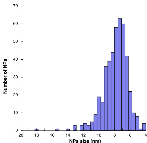
Fig. 3 Size histogram for \text{Pd}^0 NPs obtained by hydrogenation of compound 3 .
