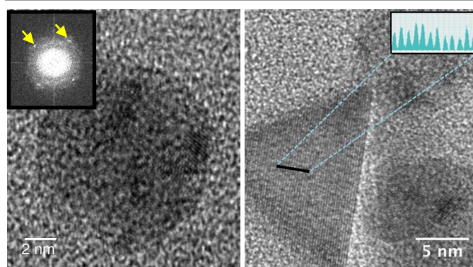
Fig. 4: HR-TEM micrograph of a \text{Pd}^0 nanoparticle obtained from 3 .
