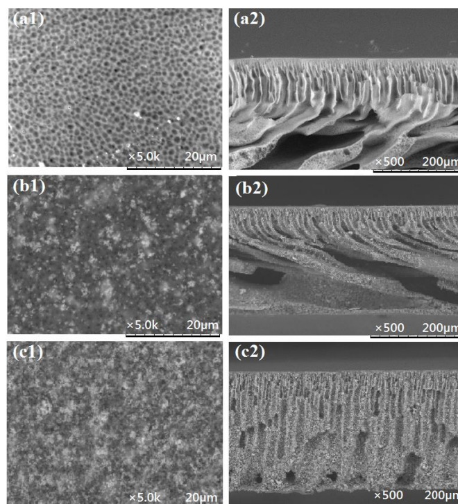
Fig. 5. SEM images of top surface (magnification of 5000 \times ) and cross section (magnification of 500 \times ) of PES membranes prepared from different nanoparticles loadings, (a) PES, (b) PES/HMO-1 and (c) PES/HMO-2 membrane
