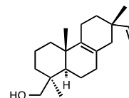
60, isopimara-8,15-diene-19-ol
