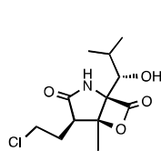
20, antiprotealide
