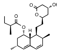
75, mevinolin
