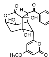
71, enterocin
