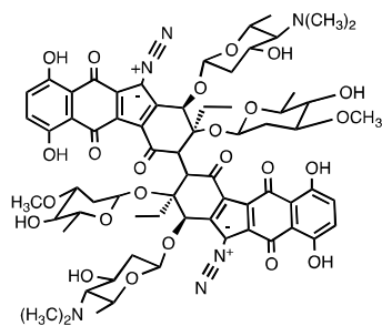
1, lomaiviticin A
