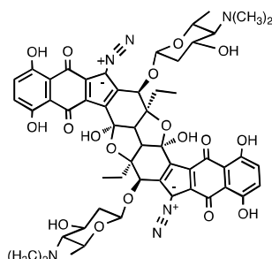
2, lomaiviticin B
