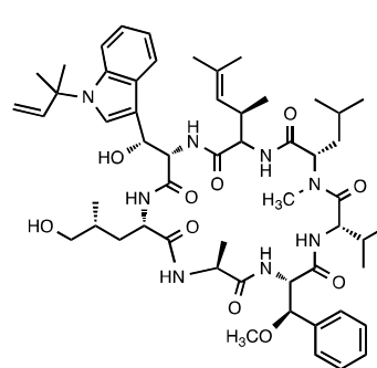
51, cyclomarin D
