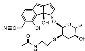
29, cyanosporaside F
