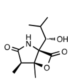
7, omuralide
