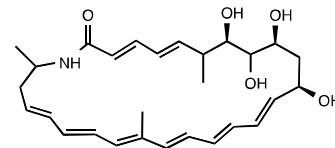
58, salinilactam
