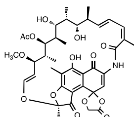
40, rifamycin O
