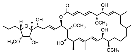
32, arenicolide C
