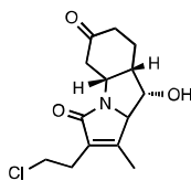
9, salinosporamide C
