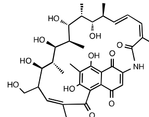
41, rifamycin W
