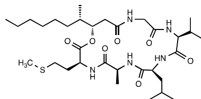
35, arenamide C
