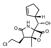
21, salinosporamide X7
