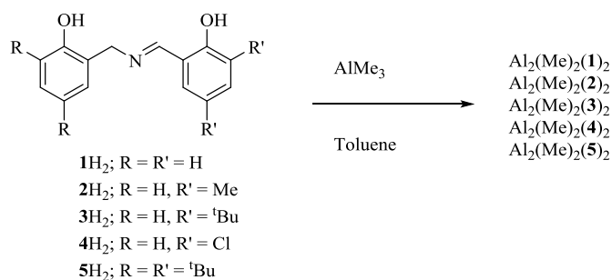
Scheme 2. Synthesis of aluminium(III) imine bis(phenolate) complexes \text{Al}_2(\text{Me})_2(\text{X})_2
