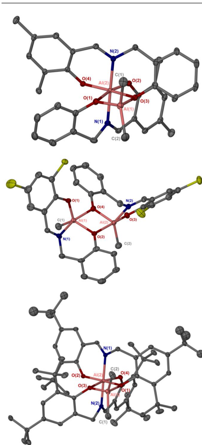
Figure 1. Solid-state structure of \text{Al}_2(\text{Me})_2(2)_2 (top), \text{Al}_2(\text{Me})_2(4)_2 (middle) and \text{Al}_2(\text{Me})_2(5)_2 (bottom) as determined by single-crystal X-ray diffraction. Ellipsoids are shown at the 30% probability level. All disorder and hydrogen atoms have been removed for clarity. See supporting information for bond lengths and angles.
