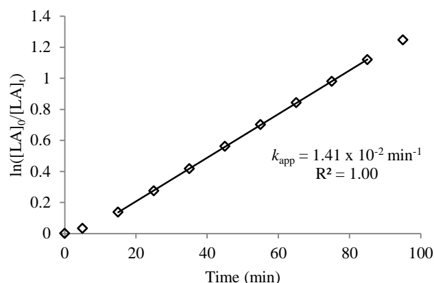
Figure 5. Semi-ln plot for the ROP of L-lactide by \text{Al}_2(\text{Me})_2(\mathbf{1})_2 showing pseudo-first order kinetics. [\text{LA}] = 0.8 \text{ mol dm}^{-3} , [\text{LA}]:[\text{I}]:[\text{BnOH}] = 100:1:1 , 353 K, toluene- d_8
