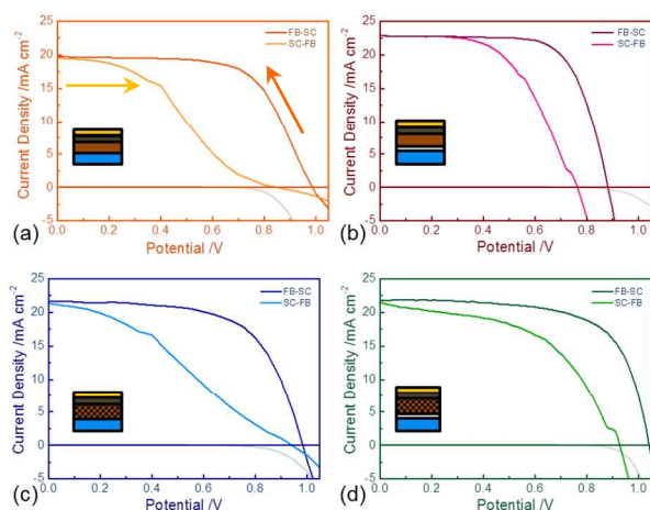
FIGURE 2 Forward bias to short-circuit (FB-SC) and SC-FB J-V curves of perovskite solar cells with different structures measured under simulated AM1.5, 100 mW cm -2 solar irradiance of the best performing solar cells for each type. Devices are scanned at 0.38V/s after holding the devices at 1.4V forward bias under illumination for 5 seconds. (a) Planar structure without a titania compact layer (b) planar structure with a titania compact layer. (c) Mesoporous structure on an Al 2 O 3 scaffold without a titania compact layer (d) mesoporous structure on an Al 2 O 3 scaffold with a titania compact layer. Corresponding dark currents (FB-SC) are plotted underneath the x-axis. The arrows indicate the scan directions. The inserted diagrams indicate cross-sections of each device configuration.
