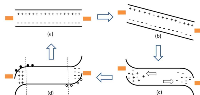
FIGURE 5 Schematic illustration of the migration of ionic species, giving a beneficial temporary photovoltaic performance after subjecting the cells to forward bias. For simplicity this diagram assumes symmetric metallic contacts and makes no judgement upon any interactions between the perovskite and the metal contacts. In (a) there is no field across the device and mobile ionic species are uniformly distributed. Instantaneously following the application of an external bias, there will be an electric field drop uniformly across the film, since the ions have no time to migrate. After a certain time period, in (c) the mobile ionic species have migrated in the appropriate direction and screened the electric field to regions closest to the interface. After removing the external bias and exposing the device to light, in (d) the ions have not had time to re-disperse and photogenerated free carriers will associate with the net negative and positive ionic species in the regions near the contacts. This will have the same effect as impurity doping and result in n-type doping near the anode (left) and p-type doping near the cathode (right). After a certain period of time (back to (a)) the ions will redistribute throughout the film and the interfacial doping will dissipate.
