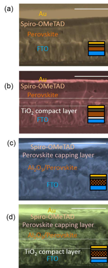
FIGURE 1 Device structure and SEM images of CH 3 NH 3 PbI 3-x Cl x perovskite solar cells (a) Planar structure without a titania compact layer. (b) Planar structure with a titania compact layer. (c) Mesoporous structure on an Al 2 O 3 scaffold without a titania compact layer. (d) Mesoporous structure on an Al 2 O 3 scaffold with a titania compact layer. The diagrams indicate cross-sections of each device. The scales indicate 1 μm.
