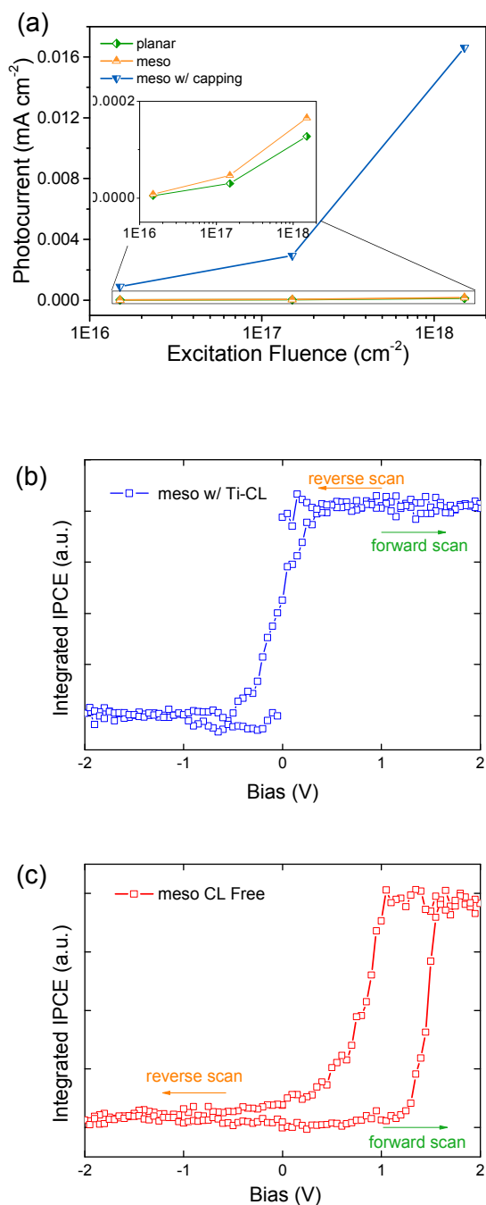
FIGURE 4 (a) photocurrent vs excitation fluence on planar, meso-structured, meso-structured with capping layer devices. Inset: enlarged photocurrent of planar and meso-structured devices. IPCE loops based on FTSP measurement. The inserted diagrams indicate cross-sections of each device configuration.
