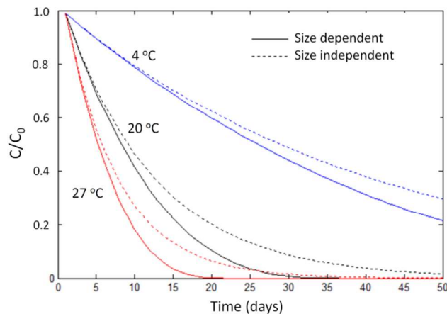
Fig. 1. A simple box model of the dissolution of a monodisperse solution of unsulfidized silver ENPs predicts relatively little error results from an assumption that "per day" mass-based reaction rates remain constant as the particle shrinks when compared to the effect of temperature (assuming an Arrhenius temperature coefficient of 1.08).
