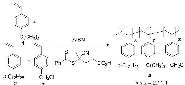
Scheme 1. Synthesis of chloromethylated poly(4-alkylstyrene) terpolymers suitable for conversion into a heptane phase-selectively soluble supports.
