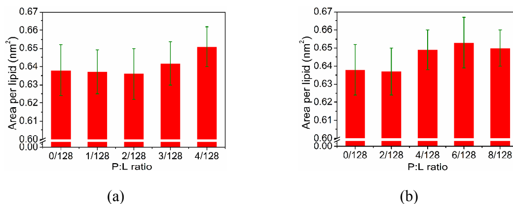
Fig. 4 Area per lipid of DPPC bilayer in the presence of varying number of ARG8 peptides. (a) All peptides were adsorbed onto one leaflet of bilayer. (b) Peptides were evenly distributed on
