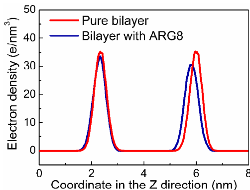
Fig. 5 Electron density profiles for phosphorus atoms on lipid heads. The profiles were obtained from the last 100 ns MD simulation data for system A8T.
