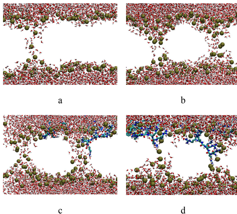
Fig. 7 On the left of each figure we show the starting configuration of an equilibrium membrane pore generated by constrained simulations (as described). To the right we show the final configuration after 200 ns of unconstrained simulations. (a) The membrane pore was generated by lipid flip-flop without peptide adsorbed on the membrane surface. The pore closed quickly after 5 ns. (b) The membrane pore was generated by peptide translocation without peptide adsorbed on the membrane surface. The peptide was then deleted and after 200 ns of MD simulations, the pore remained open. (c) The membrane pore was generated by peptide translocation with four peptides adsorbed on the membrane surface. The pore forming peptide was deleted and after 200 ns MD simulations, the pore remained open and one ARG8 peptide started to insert into the pore. (d) The membrane pore was generated by lipid flip-flop with four peptides adsorbed on the membrane surface. One arginine side chain inserted itself into the pore and kept the pore open after 200 ns of MD simulations.
