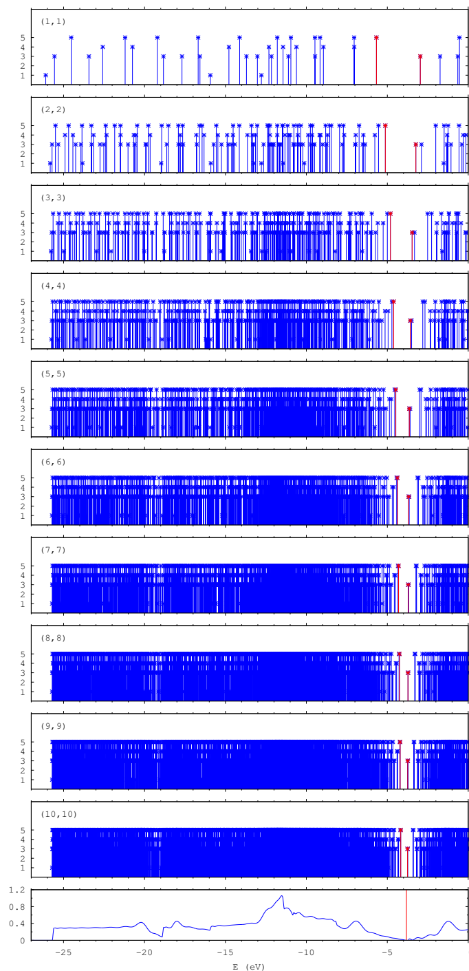
FIG. 7: Electronic levels of (n, n) fullerenes (along the x axis, in eV). For each level the corresponding degeneracy is reported along the y axis. HOMO and LUMO levels are in red. For sake of reference, density of states for graphene is shown in the bottom box (in states per eV per cell; Fermi level in red).
