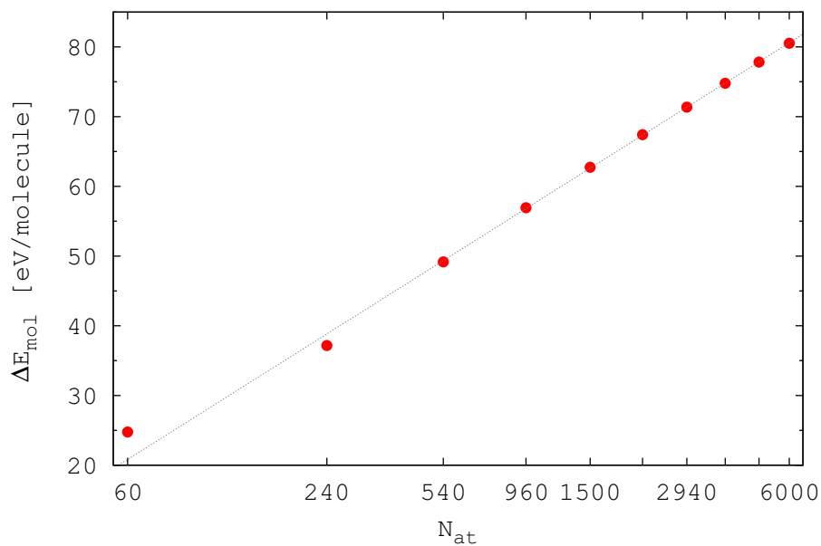
FIG. 9: Excess energy per molecule \Delta E_{mol} of (n,n) fullerenes, in eV/molecule, as a function of the number of atoms N_{at} . Points correspond to values obtained with the ab initio calculations. The curve is obtained through best-fit with respect to Eq. (10). Data for (1,1) and (2,2) are excluded from the fit (see text for details). The x axis is in logarithmic scale.
