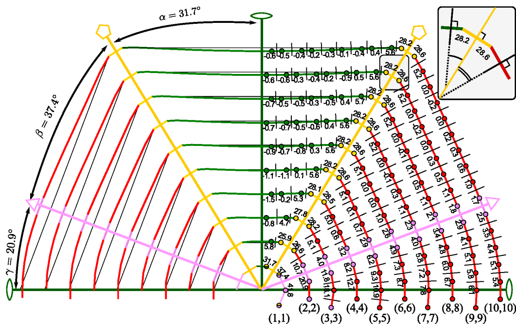
FIG. 4: Sections of (n,n) fullerenes, showing the paths described in Figure 3. All angles are in degrees. Two-, five- and three- fold rotation axes and the corresponding angles \alpha , \beta and \gamma are constant along the whole fullerene series. Right side: components of \alpha , \beta and \gamma along the path, corresponding to angles between the normals of two consecutive segments of the path (see inset on top). Left side: path profiles compared to the profiles of the ideal graphene sheet (black lines).
