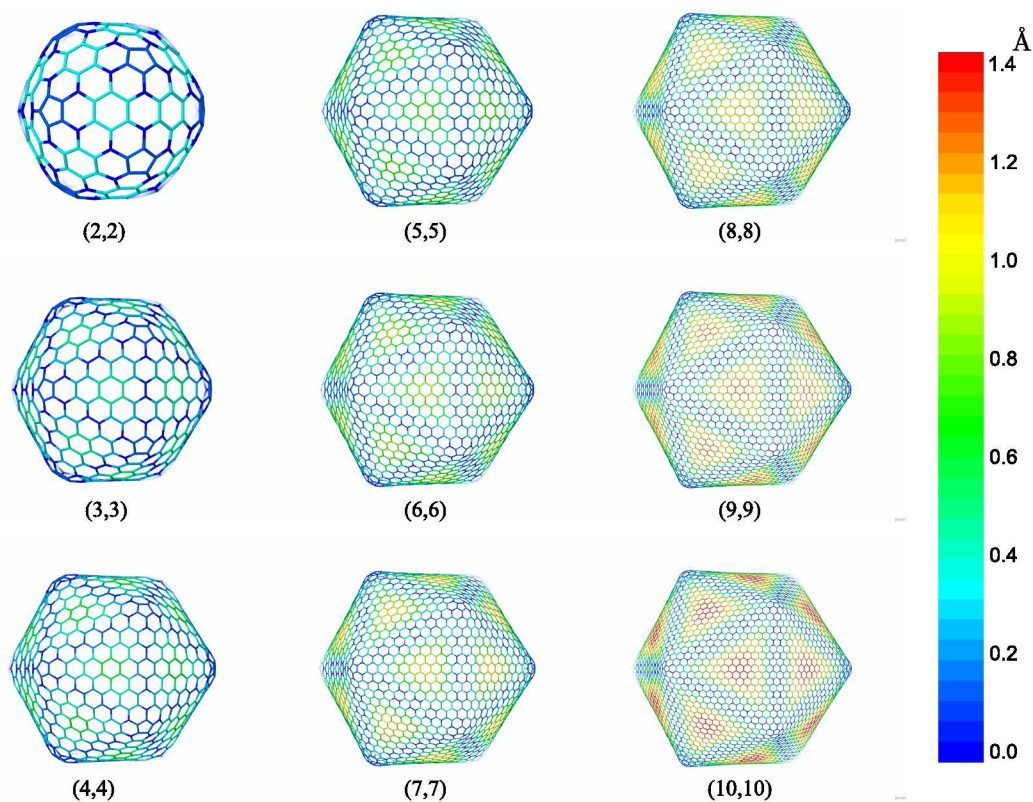
FIG. 5: Three-dimensional structures of (n,n) fullerenes ( n = 1 not shown). For each face, atomic positions have been compared to the case of an ideally flat graphene triangle; relative displacements are rendered by means of a color scale (values in Å). The graphene triangle is taken so that its z coordinate corresponds to the radius of the inscribed sphere to the ideal polyhedral fullerene, and its central hexagon is in-plane aligned with the central hexagon of the fullerene face.
