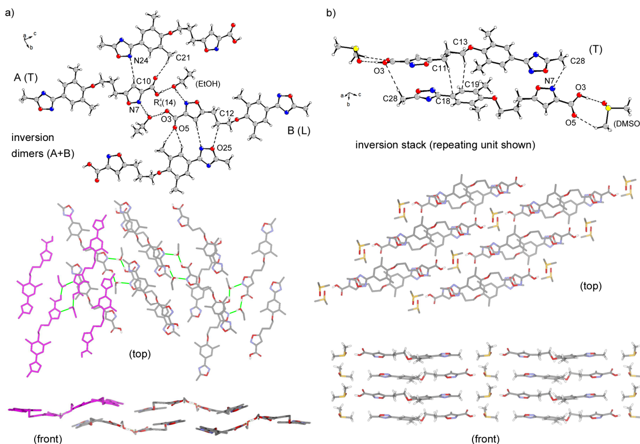
Figure 3. Inversion dimer (a) and inversion stack (b) of the solvate structures of derivative 2 with crystal packing shown for: a) 2 -EtOH and b) 2 -DMSO. Dashed black or solid green lines highlight the selected intermolecular interactions. Hydrogen atoms have been omitted for clarity when applicable.
