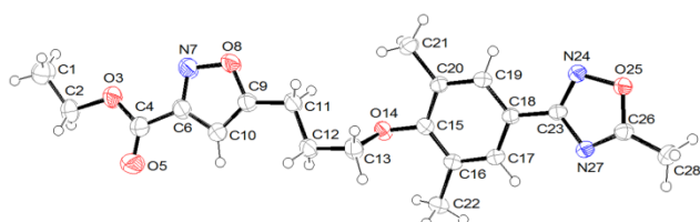
Figure 1. A representative Ortep figure of WIN 61893 analogue (derivative 1 , structure 1-form II ) with 50% ellipsoid probability and a numbering scheme used for all structures.
