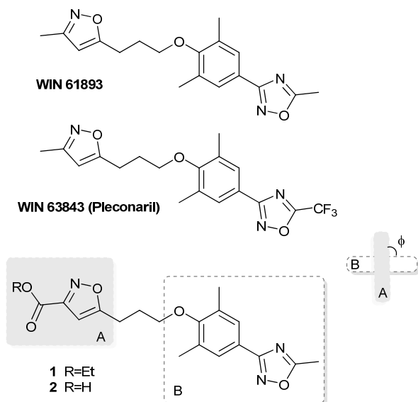
Scheme 1. Chemical structures of WIN 61893, WIN 63843 (Pleconaril) and derivatives 1 and 2 .
