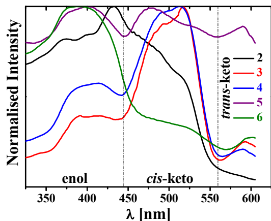
Fig. 9 Normalised solid-state excitation spectra of 2–6 at 298 K ( \lambda_{\text{em}} = 620 nm).
