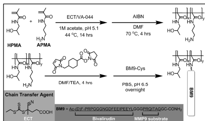
Scheme. 1 Synthetic scheme of HPMA-BM9 copolymers.
