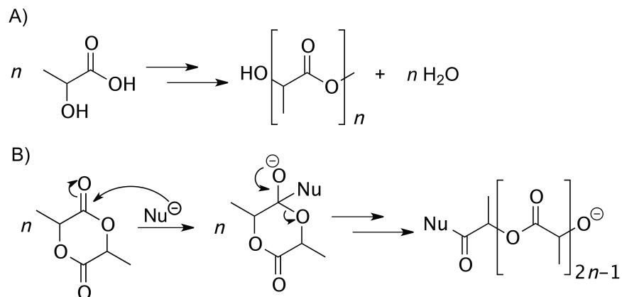
Figure 7. (A) Polymerization of lactic acid; (B) ring-opening polymerization of lactide.
