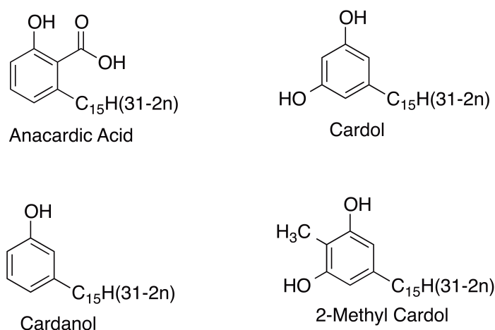
Figure 2. Major components of cashew nut shell liquid, where n = 0, 1, 2, or 3.
