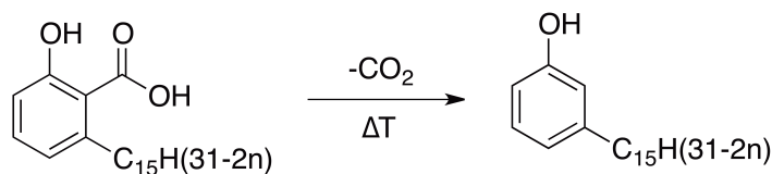
Figure 3. Conversion of anacardic acid to cardanol, where n = 0, 1, 2, or 3.
