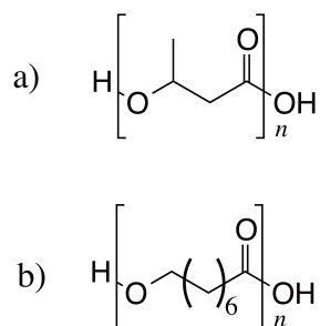
Figure 8. Chemical structure of (a) poly-3-hydroxybutyrate (P3HB), and (b) polyhydroxyoctanoate (PHO).
