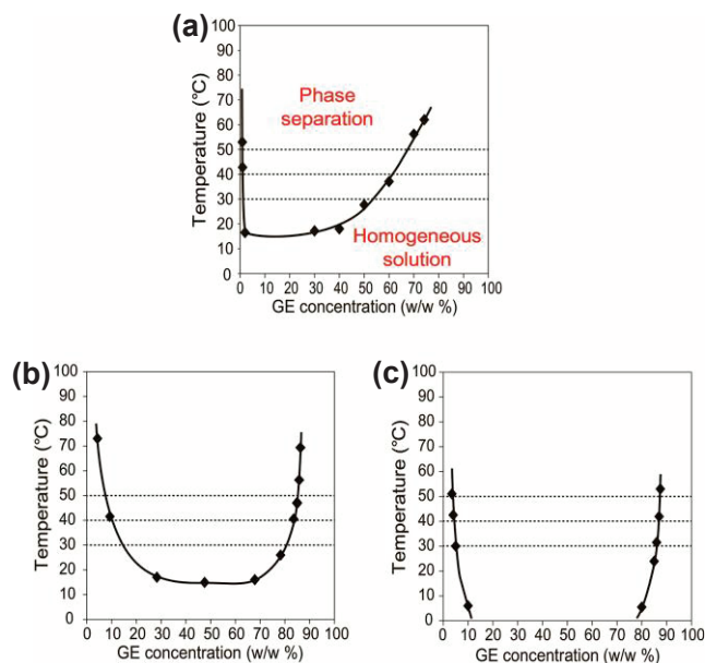
Fig. 3 Phase diagrams of GE-water mixtures; (a) DEH/water, (b) DPP/water, and (c) PB/water.
