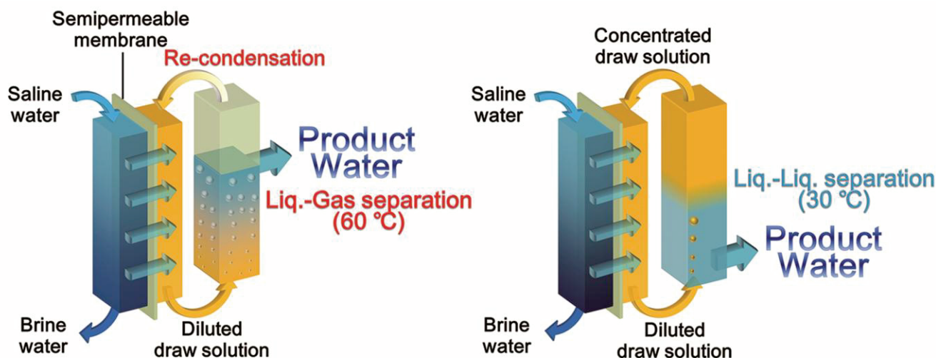
Fig. 1 Schematic illustration of the FO desalination systems based on a liquid-gas phase separation (left) and a liquid-liquid phase separation (right).
