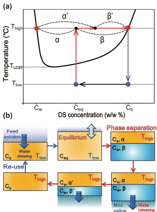
Fig. 7 Illustration of a FO desalination process by a phase diagram and a schematic diagram describing relative concentrations and amounts of each phase. DS: draw solute; T_{LCST} : LCST temperature; T_{high} and T_{low} : operation temperatures (high T and low T); C_s : the DS concentration in the draw solute-rich phase after phase separation at T_{high} ; C_w : the DS concentration in the water-rich phase after phase separation at T_{high} ; C_{eq} : the DS concentration of draw solution with an equivalent osmotic pressure to the feed solution.
