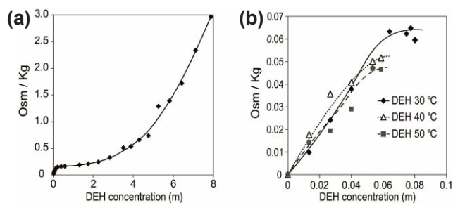
Fig. 5 Osmolality of DEH/water mixture at various concentrations (a) at low T measured by freezing point depression and (b) at high T measured by vapor pressure depression.
