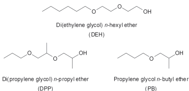
Fig. 2 Chemical structures of glycol ethers evaluated in this study.
