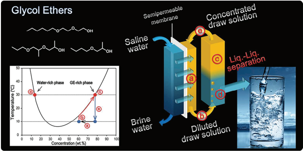
Lower critical solution temperature (LCST) phase transition of glycol ethers by mild temperature gradient induces drastic conversion of osmotic pressure to enable energy-efficient forward osmosis (FO) desalination. 80x39mm (300 x 300 DPI)
