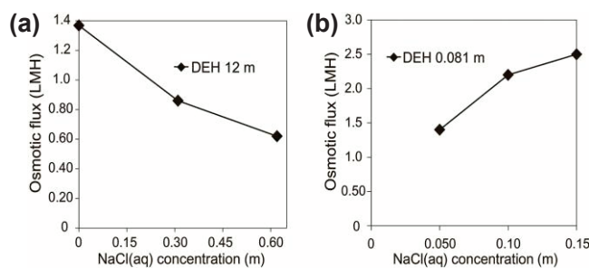
Fig. 6 Osmotic flux between the DEH aqueous solution and NaCl solutions at (a) 10 and (b) 30 °C. (a) The flow from the NaCl solution to a 12 m DEH solution. (b) The flow from the 0.081 m DEH solution ( i.e. , water-rich phase) to the NaCl solution.
