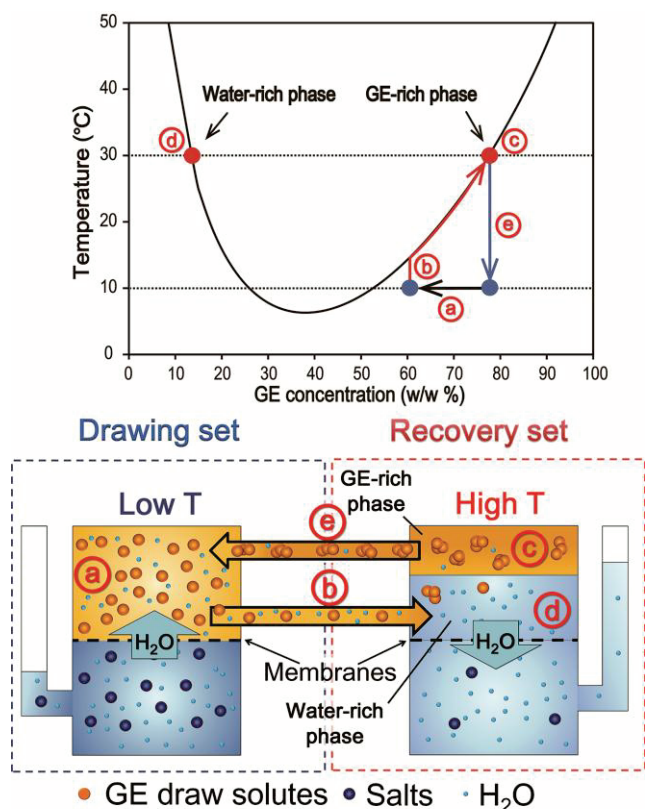
Fig. 4 A schematic diagram of a FO desalination system based on the GE/water phase diagram.
