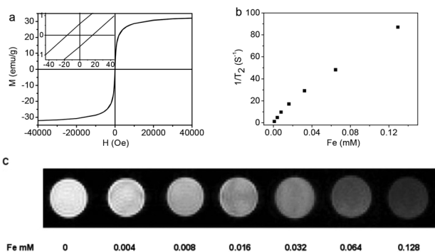
Fig. 5 (a) The hysteresis loop of \text{Fe}_3\text{O}_4 @C-CDs NPs measured at room temperature. The left inset shows the respective expanded plots for fields between -40 and 40 Oe; (b) T_2^* relaxation rates as a function of iron concentration (mM) for \text{Fe}_3\text{O}_4 @C-CDs NPs; (c) T_2^* -weighted MR images of \text{Fe}_3\text{O}_4 @C-CDs NPs at different concentrations, corresponding to different amount of Fe.
