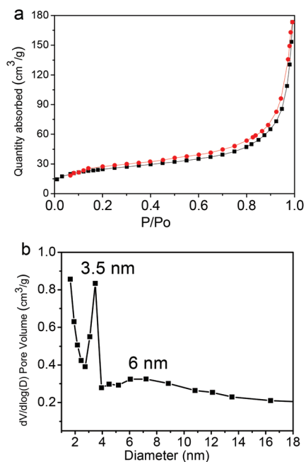
Fig. 8 (a) \text{N}_2 adsorption/desorption isotherms and (b) the pore size distribution of the \text{Fe}_3\text{O}_4 @C-CDs hybrid NPs.
