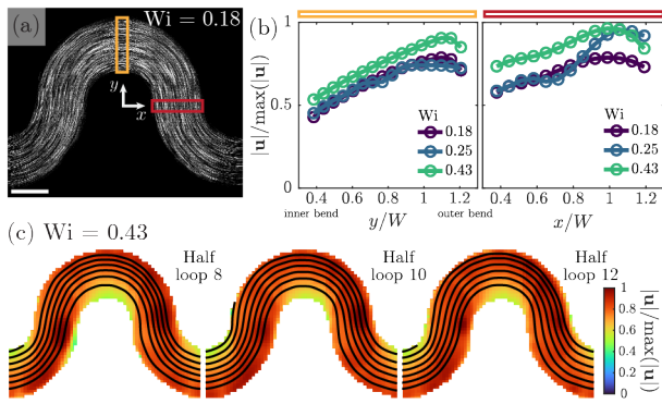
Fig. 3 Base steady laminar flow exhibits strong shear thinning and slip at surfaces. (a) Pathline image of flow in the R_i = 300 \mu\text{m} device at Wi = 0.18 < Wi_c , generated using a moving average of fluorescence intensity over 60 frames. Scale bar is 500 \mu\text{m} . (b) Time-averaged (over 86\lambda ) velocity profiles, normalized by the maximum velocity, at the apex (yellow rectangle) and end (red rectangle) of a half-loop. All velocity profiles exhibit highly asymmetric plug flow and indicate the presence of a substantial slip velocity at surfaces. The PIV grid resolution used is 0.05W . (c) Streamline visualization and color maps of the normalized velocity magnitudes at selected half-loop locations further reflect strong plug flow and asymmetry in the base laminar flow state.
