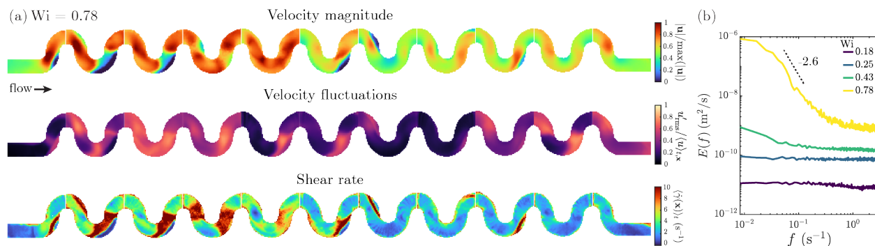
Fig. 4 Unsteady 3D flow arising from an elastic instability. (a) Instantaneous color maps of the flow field measured at the channel mid-height in the unsteady flow state showing the (top) normalized velocity magnitude |\mathbf{u}|/\max(|\mathbf{u}|) , (middle) root-mean-square (rms) velocity magnitude fluctuations u'_{\text{rms}}/\langle u \rangle_{r,x} , and (bottom) shear rate \dot{\gamma}(x) in the R_i = 300 \mu\text{m} channel at Wi = 0.78 > Wi_c . The top and bottom rows show near-instantaneous flow fields that are time-averaged over a duration of 1\lambda to reduce noise. The middle row shows rms velocity fluctuations over a duration of 86\lambda , highlighting the spatial heterogeneity and temporal persistence of flow fluctuations. All color maps comprise stitched fields-of-view obtained sequentially during flow imaging, giving rise to the visible discontinuities between adjacent half-loops. (b) Power spectral densities of the magnitude of velocity fluctuations indicate that above the onset of the elastic instability, more energy is dissipated in fluctuations across a broad range of frequencies, with no characteristic time scale.
