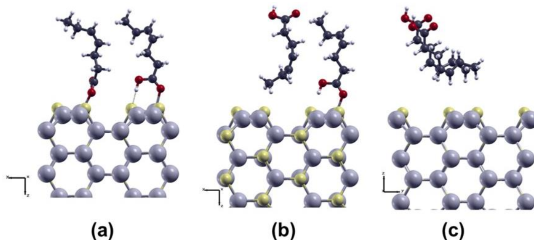
Figure 7. Depiction of the final adsorption geometries for a dimer pairing of the cis isomer ligand with a) both COOH groups pointed toward the surface, b) one COOH and one CH 3 group alternating, and c) both CH 3 groups pointed towards the surface. Cd atoms are illustrated here as gray spheres, S atoms as yellow spheres, O atoms as red spheres, C atoms as black spheres, and H atoms as white spheres.
