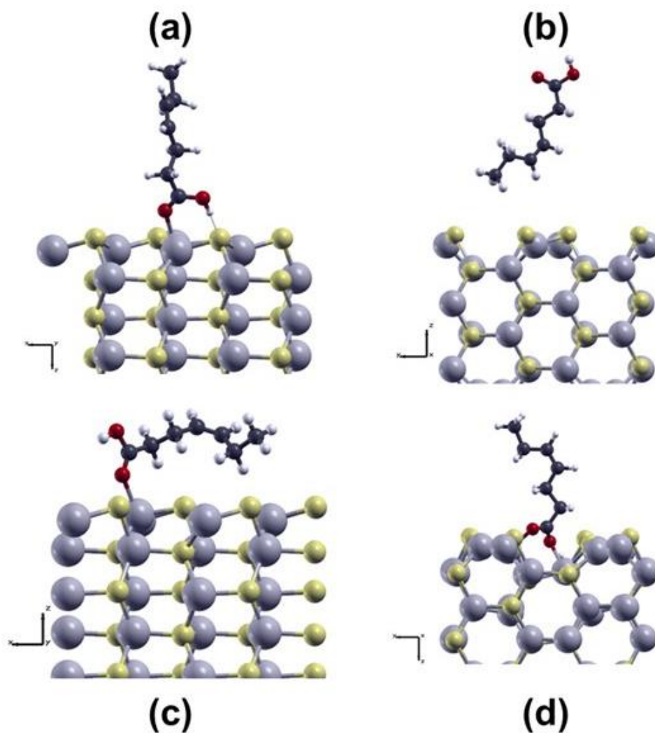
Figure 6. Depiction of the final adsorption geometries for a single cis isomer of 4-heptenoic acid with the a) COOH or b) CH 3 group pointed towards the CdS surface, the c) flat configuration, and
