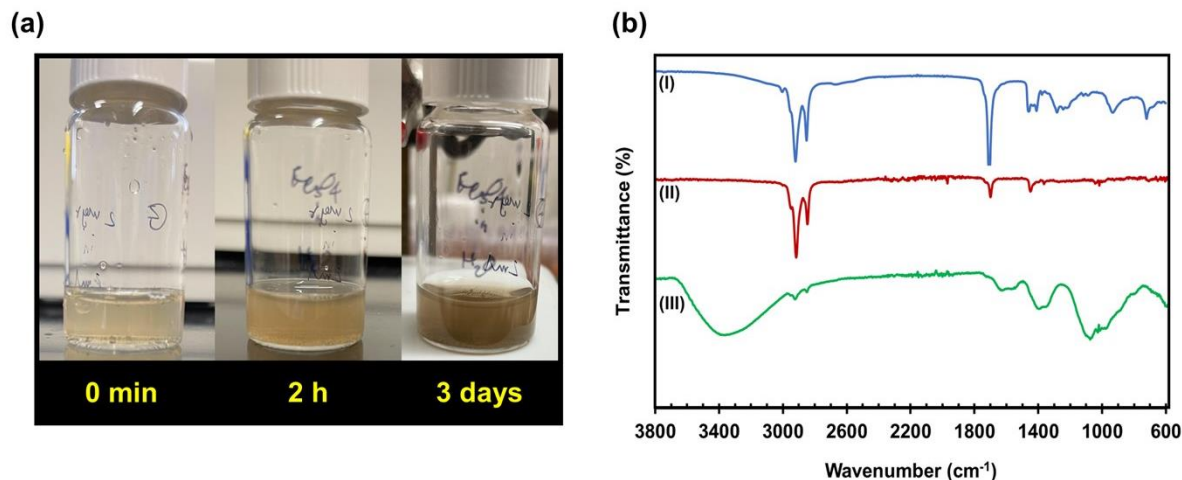
Figure 5. (a) Photographs of oleic-acid (OA)-coated magnetite nanoparticles (NPs) transferred into pH 8 water as a function of time. (b) FT-IR spectra of pure OA ligands (I), OA-coated magnetite NPs in hexane (II), and OA-coated magnetite NPs after transfer into water (III).
