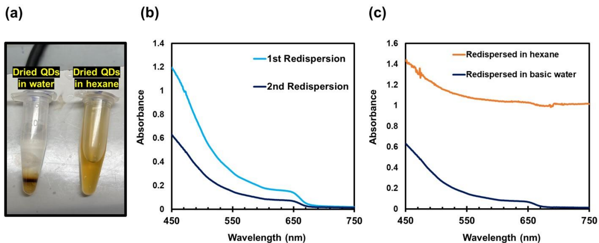
Figure 4. (a) Photograph of dried pellets of oleid-acid-capped quantum dots (QDs) redispersed in water (left) and hexane (right). (b) Absorption spectra of the water-soluble QDs after a first and second redispersion in basic water. (c) Absorption spectra of the water-soluble QDs after a second redispersion in basic water and in hexane, after first being redispersed in basic water.
