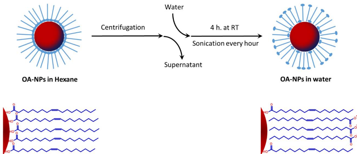
Figure 1. Illustration of nanoparticle transfer from hexane to water through the rearrangement of oleic acid capping molecules.
