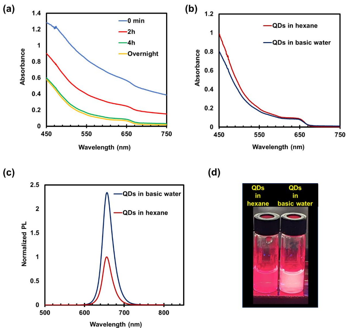
Figure 2. (a) Absorption spectra of oleic-acid (OA)-capped quantum dots (QDs) after redispersion into aqueous media (pH 8) as a function of time. (b) The comparison of QD absorbance in hexane versus after complete redispersion into basic water (pH 8). (c) Emission spectra of OA-capped QDs in hexane and after transfer into basic water. (d) Photographs of QDs under UV light illumination (365 nm) in hexane (left) and in pH 8 water (right).
