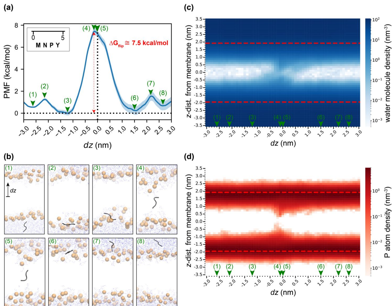
Figure 2. Analysis of flipping for the truncated N-terminal loop (N-loop). (a) Potential of mean force (PMF) as a function of the z -component of the distance between the COM of the N-loop and the center of the membrane, dz . The amino-acid sequence of the N-loop is in the top-left inset. The midplane of the membrane is at dz = 0 nm. The blue shaded area indicates the standard deviation computed by bootstrapping. (b) Simulation snapshots of N-loop flipping. Each snapshot corresponds to a representative configuration for the value of dz marked by a green arrowhead on the PMF curve in (a). The N-loop is gray, phosphorus atoms of lipid head groups are orange, water molecules are blue dots, and lipid tails are not shown to aid visualization. (c) Heatmap of water molecule number densities as a function of dz . Each point in the heatmap shows the density of water molecules with the specified z -component of the distance from the membrane midplane averaged over time and over all x - y positions. Densities are computed using configurations from the umbrella sampling trajectories with the value of dz ( i.e. , the distance of the N-loop from the membrane midplane). The red dashed lines indicate the distances from the center of the membrane that correspond to the maximum average densities of phosphorus atoms from (d). (d) Heatmap
