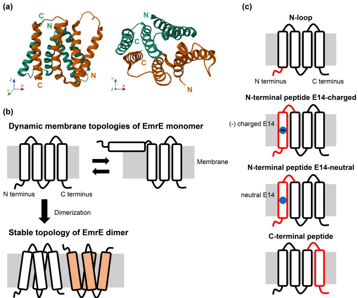
Figure 1. Structure, topology, and sequence of EmrE and truncated segments studied in this work. (a) Structure of the EmrE dimer viewed from within the x - y plane of the membrane (left) or down the z -axis from above the membrane (right). The two monomers are colored green (chain A) and orange (chain B). The N- and C-termini for each monomer are labeled with “N” and “C”, respectively. (b) Schematic of dynamic membrane topologies of the EmrE monomer 32 , in which the N-terminal (but not C-terminal) transmembrane helix crosses (flips) across the membrane (top). Flipping is no longer observed experimentally after the monomers assemble into a dimer (bottom). (c) Schematics of the truncated segments (colored in red) from the EmrE monomer that are used for the simulations in this work. The blue dot indicates the approximate position relative to the membrane of the E14 residue. Corresponding amino-acid sequences are shown in Figures 2-4.
