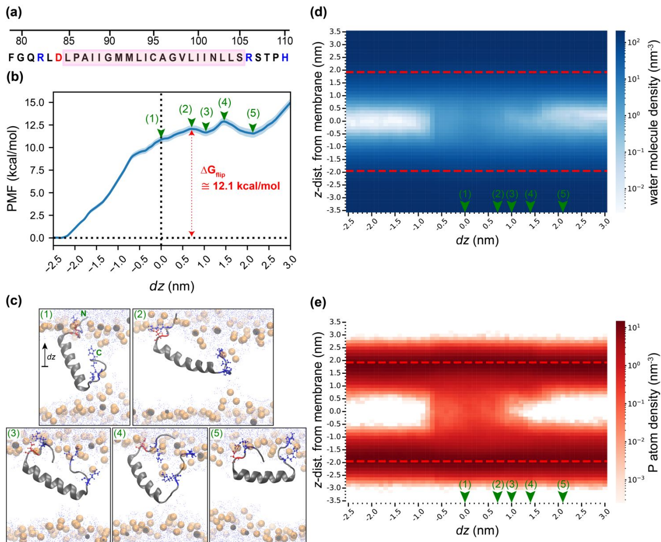
Figure 4. Analysis of flipping for the truncated C-terminal peptide (C-pep). (a) Amino-acid sequence of C-pep. The index of each amino acid with respect to the whole EmrE monomer sequence is shown above the residue. The transmembrane helical (TMH) domain is highlighted with the pink box. Residues colored in blue and red are positively and negatively charged residues, respectively. (b) Potential of mean force (PMF) as a function of the z -component of the distance between the COM of the C-terminal loop and the center of the membrane, dz . The midplane of the membrane is at dz = 0 nm. The blue shaded area indicates the standard deviation computed by bootstrapping. (c) Simulation snapshots of C-pep flipping. Each snapshot corresponds to a representative configuration for the value of dz marked by a green arrowhead on the PMF
