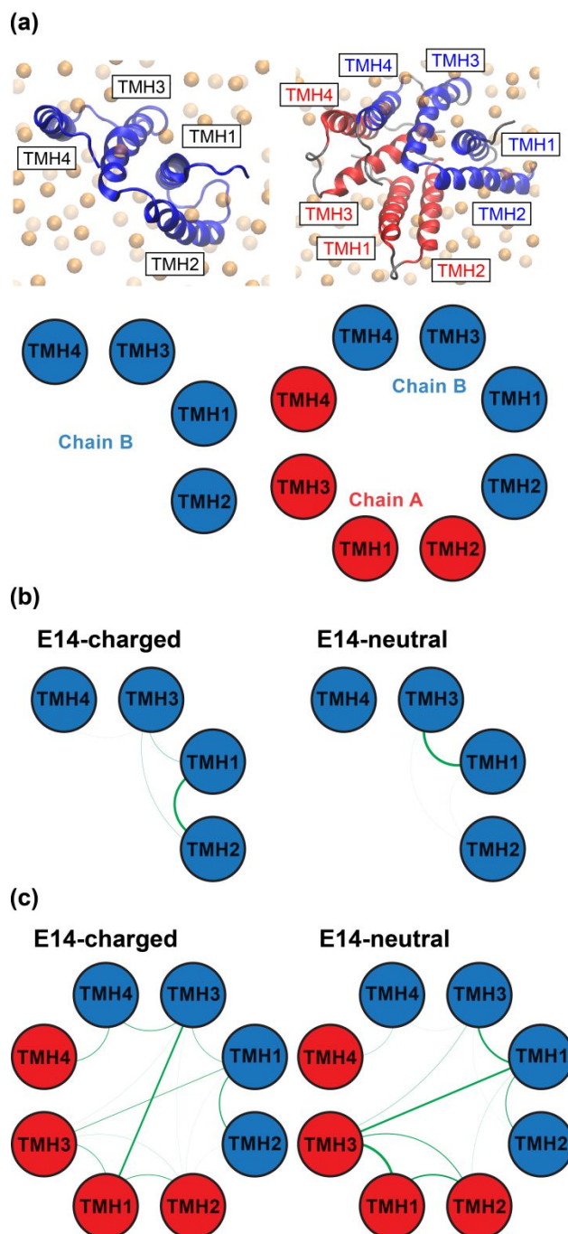
Figure 7. Interhelical hydrogen bonding patterns in EmrE. (a) Structures of the EmrE monomer (left) and dimer (right) viewed from above the membrane. Chain A is in red, chain B is in blue, and phosphorus atoms are in orange. Topological maps of TMHs corresponding to each structure are shown below with helices numbered by the order in which they appear in the primary sequence. (b) Topological maps of interhelical hydrogen bonds for the EmrE monomer with E14 deprotonated (E14-charged, at left) or protonated (E14-neutral, at right). Green lines connecting the TMHs represent hydrogen bonds and the line thickness quantifies their persistence based on the time-averaged number of the bonds during a 500 ns simulation
