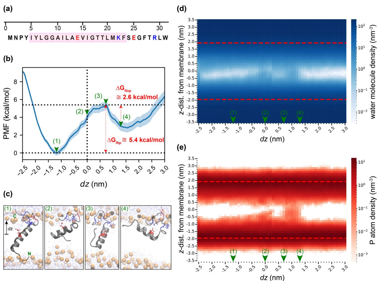
Figure 3. Analysis of flipping for the truncated N-peptide-E14-charged (N-pep-charge). (a) Amino-acid sequence of N-pep-charge. The index of each amino acid with respect to the whole EmrE monomer sequence is shown above the residue. The transmembrane helix (TMH) of the peptide is highlighted with the pink box. Residues colored in blue and red are positively and negatively charged, respectively. E14 is
