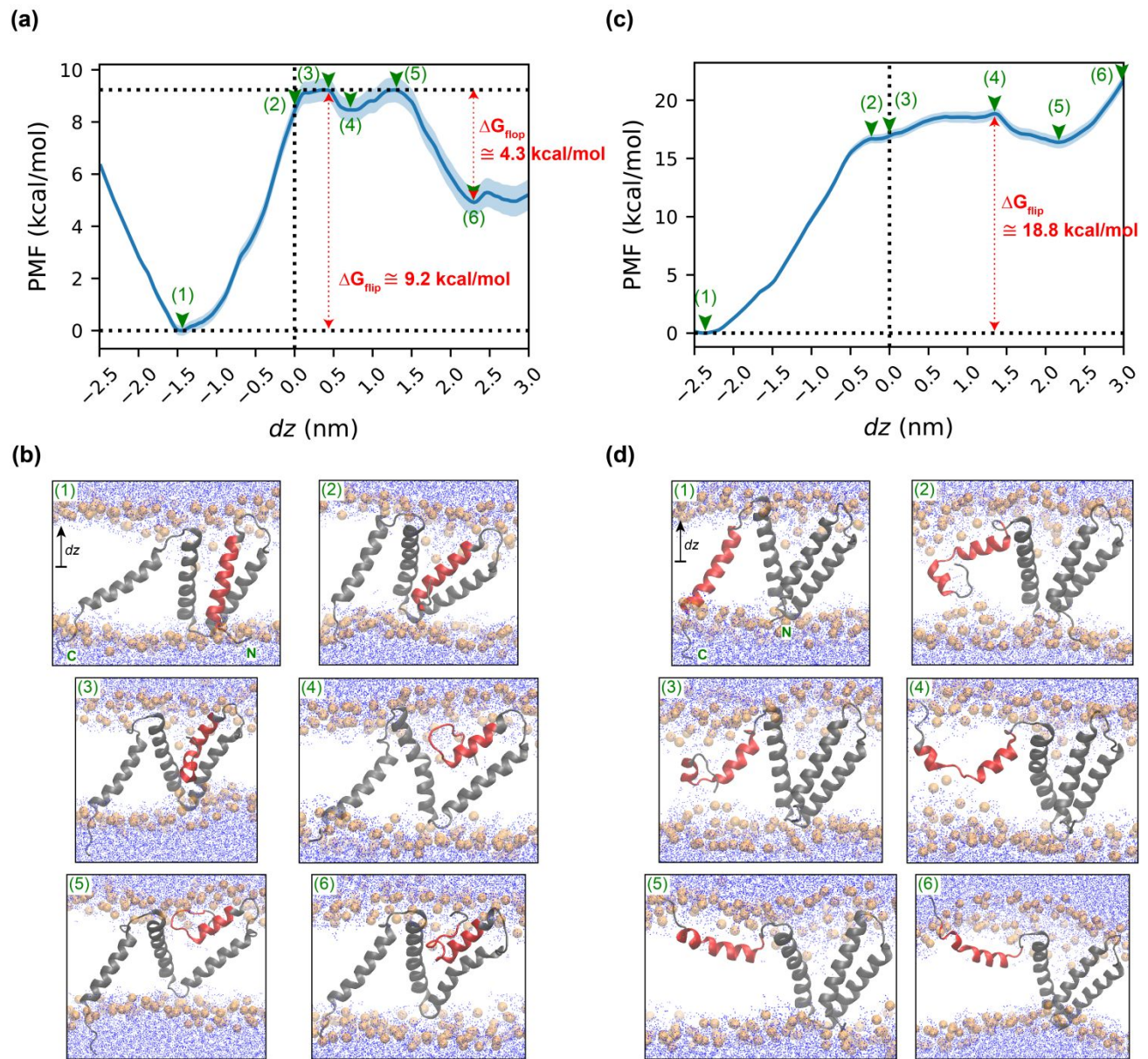
Figure 5. Analysis of flipping for the N- and C-terminal loops of EmrE monomer. (a) Potential of mean force (PMF) as a function of the z -component of the distance between the COM of the N-terminal loop and the center of the membrane, dz . The midplane of the membrane is at dz = 0 nm. The blue shaded area indicates the standard deviation computed by bootstrapping. (b) Simulation snapshots of EmrE N-terminal TMH1 flipping. Each snapshot corresponds to a representative configuration for the value of dz marked by a green arrowhead on the PMF curve in (a). The EmrE monomer is gray, TMH1 is red, phosphorus atoms of lipid
