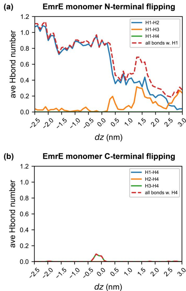
Figure 6. Interhelical hydrogen bonding patterns of flipping for the N- and C-terminal loops of EmrE monomer. (a) Time-averaged number of hydrogen bonds between TMH1 and other helices for the N-terminal loop flipping as a function of dz . The legend “H1-H2” indicates H-bonds between TMH1 and TMH2 and other legends follow the same definition. The red dashed line indicates all interhelical H-bonds of TMH1. (b) Time-averaged number of hydrogen bonds between TMH4 and other helices for the C-terminal loop flipping as a function of dz . The legend “H1-H4” indicates H-bonds between TMH1 and TMH4 and other legends follow the same definition. Red dashed line indicates all interhelical H-bonds of TMH4.
