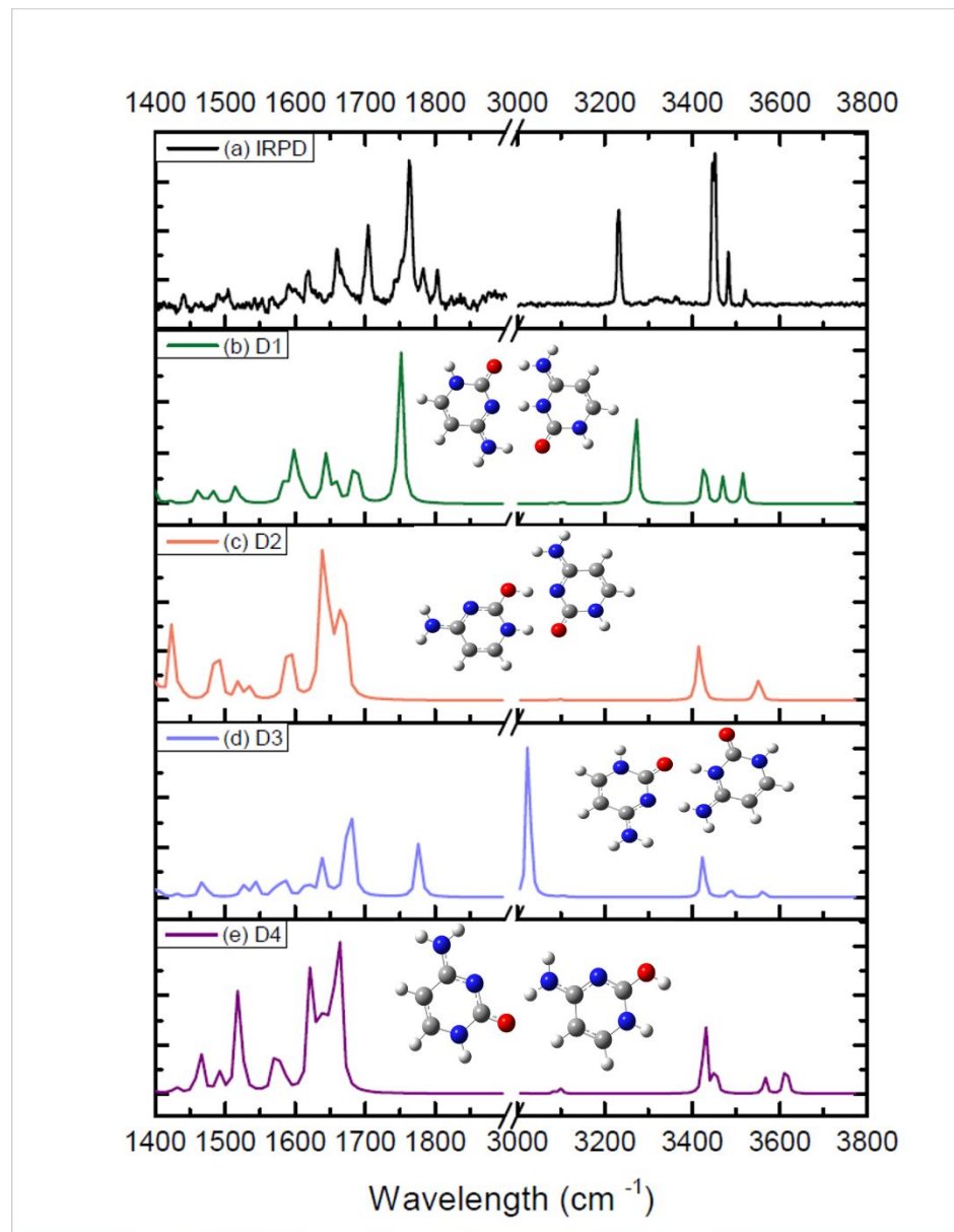
Figure 3: Comparison of the measured IRPD spectrum (a) with the calculated vibrational spectra of the most stable protonated cytosine dimer structures (b-e) in the 3-micron ( 3000\text{--}3800\text{ cm}^{-1} ) and 6-micron ( 1400\text{--}2000\text{ cm}^{-1} ) regions. Panels (b-e) correspond to the D1 (b), D2 (c), D3 (d), and D4 (e) structures.
