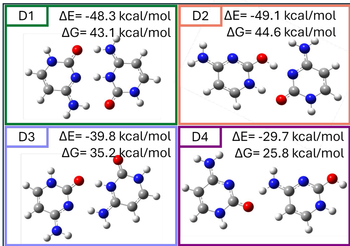
Figure 4: Optimized geometries of the most stable hemiprotonated cytosine dimer structures (D1–D4) calculated at the MP2/cc-pVTZ level, their interaction energies ( \Delta E ) and binding free energies ( \Delta G ) with a positive sign indicating stabilization, are presented above each structure. Color code: grey = carbon, red = oxygen, blue = nitrogen, white = hydrogen.
