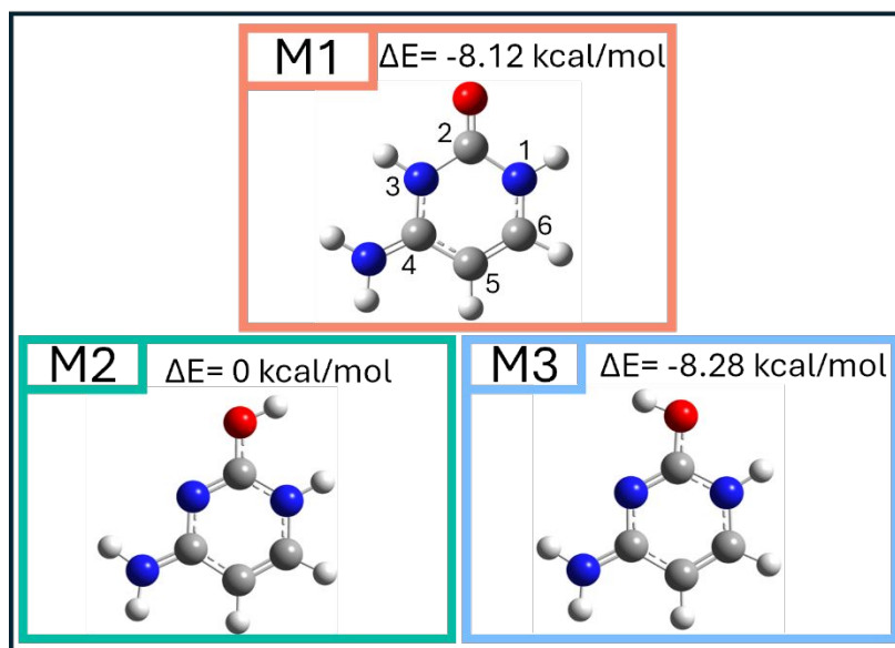
Figure 1: Most stable protonated cytosine monomer structures (M1, M2, M3) and their relative energies ( \Delta E ) optimized in the gas phase at the MP2/cc-pVTZ level. Atomic color code representation: grey- carbon, red- oxygen, blue -nitrogen, and white- hydrogen.
