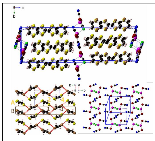
Fig. 1 (top) Packing diagram of \alpha -(BEDT-TTF) 2 Hg(SeCN) 2 Cl. (bottom left) \alpha -type packing motif of the BEDT-TTF layer. The sulphur atoms in the crystallographically unique BEDT-TTF molecules are shown as yellow and brown spheres, respectively. Intermolecular S-S interactions less than 3.6 Å are indicated with red lines. The brown rectangle indicates the 1D spin chain. (bottom right) The dimerized Hg(SCN) 2 Cl - anion forms a 2D structure. Colour scheme: carbon (black), sulphur (yellow/brown), hydrogen (salmon), mercury (magenta), nitrogen (blue), selenium (maroon), and chlorine (green).
