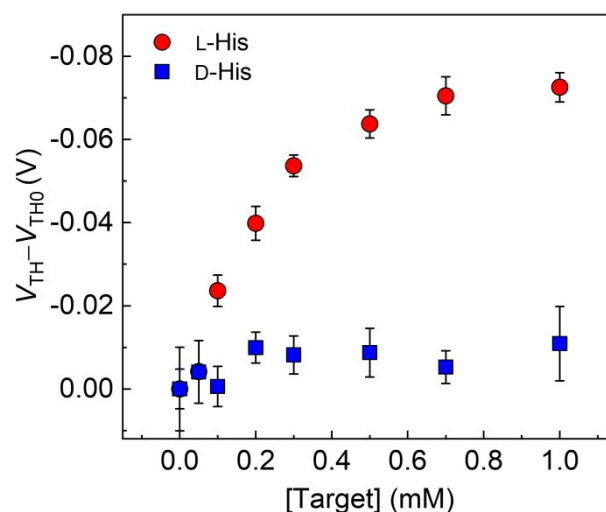
Fig. 3 Responses of the MIP-OFET to L- (red circles) and D-His (blue squares) in a phosphate buffer solution (100 mM) at pH 6.0 at 25 °C. The terms V_{\text{TH0}} and V_{\text{TH}} mean threshold voltages before and after adding targets ( n = 3 ). The titration isotherms were obtained by collecting V_{\text{TH}} at V_{\text{GS}} = -2 V.
