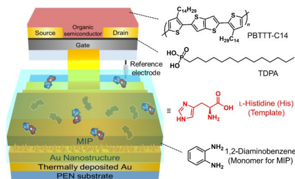
Fig. 1 Schematic illustration of an extended-gate-type OFET functionalized with MIP for chiral recognition and %ee determination of L-His and chemical structures of the sensor components. 1,2-Diaminobenzene was used as the functional monomer for MIP fabrication.
