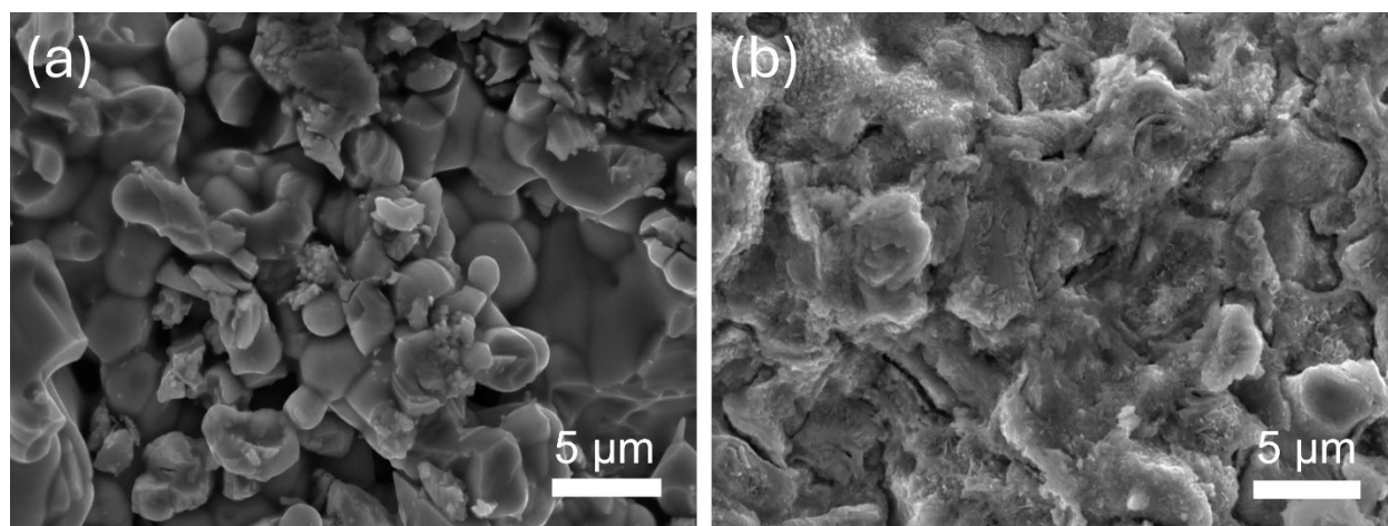
Fig. 2 SEM images at the center of cross section of the polycrystal \text{Sr}_{12}\text{Y}_2\text{Cu}_{24}\text{O}_{41} (a) before and (b) after 10 h water treatment.
