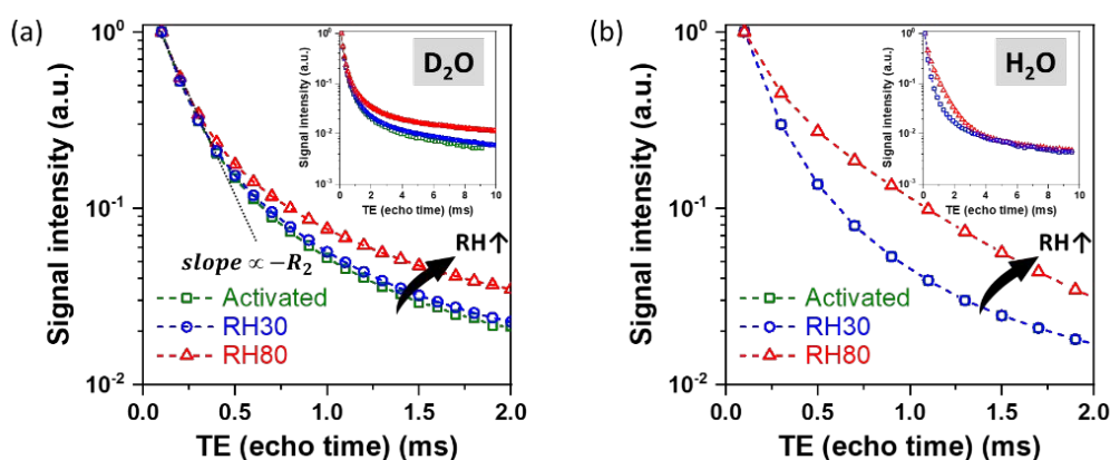
Fig. 7 ^1\text{H} NMR relaxation decay curves obtained at 9.4 T of activated and water ( \text{D}_2\text{O}/\text{H}_2\text{O} + \text{N}_2 ) adsorbed materials at 25 ^\circ\text{C} with RH30, and RH80 for R_2 = (1/T_2) relaxations. Considering potential deuterium exchange in polymer, the data presented in \text{D}_2\text{O} is used after reactivating \text{D}_2\text{O} adsorbed sample in (a). Measurements with Activated and RH30 in (b) are overlapped in the graph.
