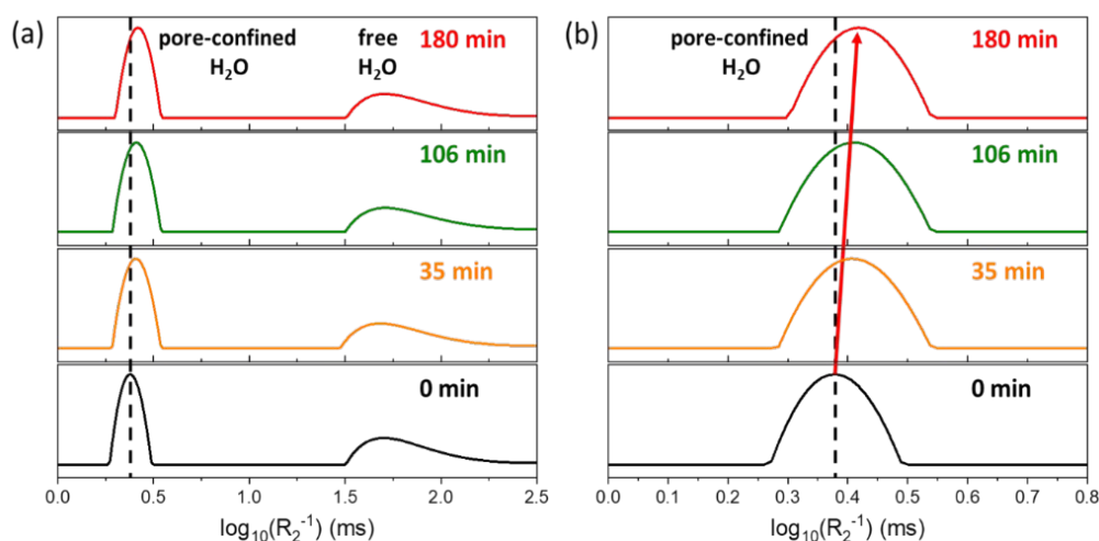
Fig. 6 Changes in transverse relaxation rates ( R_2^{-1} = T_2 ) of water saturated within material, measured at a resonant ^1\text{H} frequency of 13.11 MHz. (a) R_2 distribution interpreted as pore-confined H 2 O (faster R_2 , i.e. shorter T_2 ) and free H 2 O (slower R_2 , i.e. longer T_2 ); (b) magnified view of (a), highlighting the changing R_2 distribution of pore-confined H 2 O. Dashed black and solid red lines are a guide to the eye.
