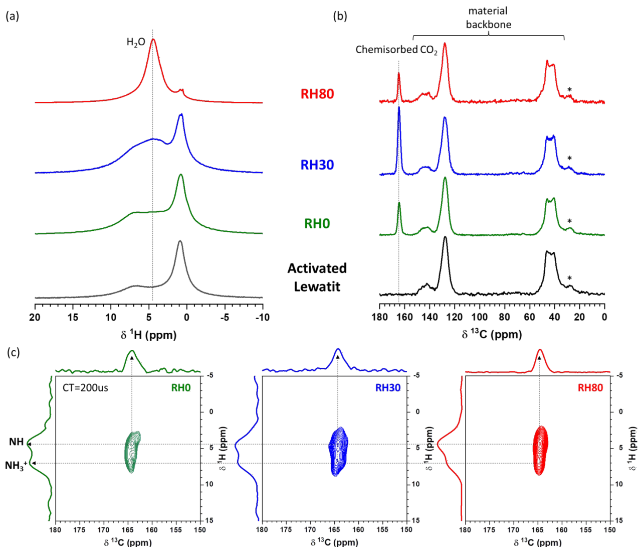
Fig. 4 Solid-state MAS NMR spectra of Lewatit® VP OC 1065 dosed with co-adsorption ( \text{N}_2 , \text{CO}_2 , and \text{H}_2\text{O} ) at low p\text{CO}_2 with variable RHs (RH0, RH30, and RH80). (a) ^1\text{H} DEPTH NMR; (b) ^{13}\text{C} CPMAS NMR with 200 \mu\text{s} of contact time; (c) ^{13}\text{C} - ^1\text{H} FSLG-HETCOR 2D spectra with 200 \mu\text{s} of contact time. Activated Lewatit refers to a state where sample pretreatment (high vacuum) lead to no adsorbed species. In ^{13}\text{C} CPMAS NMR spectra, * indicates spinning sideband and signals at 40–50 ppm, 120–130 ppm, and 140 to 150 ppm arise from the backbone in Lewatit® VP OC 1065, where not affected by \text{CO}_2 adsorption.
