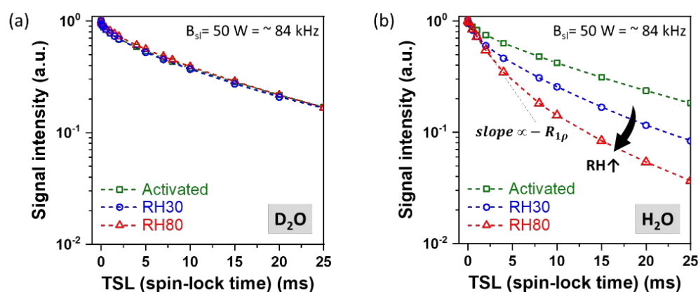
Fig. 8 ^1H NMR relaxation decay curves obtained at 9.4 T of activated and water ( D_2O/H_2O + N_2 ) adsorbed materials at 25 °C with RH30, and RH80 for R_{1\rho}(=1/T_{1\rho}) relaxations. Considering potential deuterium exchange in polymer, the data presented in D_2O is used after reactivating D_2O adsorbed sample in (a).
