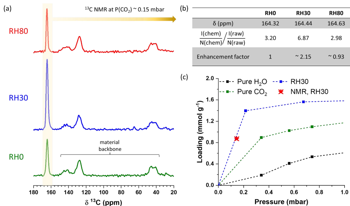
Fig. 5 Quantitative \text{CO}_2 adsorption at various relative humidities. (a) Solid-state ^{13}\text{C} NMR obtained by direct excitation under MAS on samples exposed to a mixture gas \text{N}_2 + \text{CO}_2 + \text{H}_2\text{O} at 25 °C with RH0 (bottom, green), RH30 (middle, blue), and RH80 (top, red). (b) Tabulated values of quantified \text{CO}_2 adsorption corresponding to the NMR spectra shown in (a). In table, I(\text{chem}) or I(\text{raw}) represents the integral area associated with chemisorbed species or sorbent itself in the spectra, and N(\text{chem}) or N(\text{raw}) denotes the number of carbons associated with chemisorbed species or sorbent itself. (c) Comparison of the adsorbed \text{CO}_2 obtained from NMR ( \text{N}_2 + \text{CO}_2 + \text{H}_2\text{O} ) with the isotherm experiments \text{CO}_2 , RH30 ( \text{CO}_2 + \text{H}_2\text{O} ), and water at 25 °C. Isotherm experiments were described previously and reproduced from Ref.22 with permission from the Royal Society
