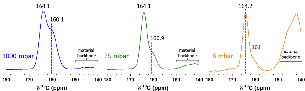
Fig. 1 13 C solid-state CPMAS (contact time 2 ms) NMR of CO 2 adsorbed at various pressures (1000 mbar in blue, 35 mbar in green or 8 mbar in orange) within Lewatit® VP OC 1065. Signals observed between 140 to 150 ppm originate from the backbone in Lewatit® VP OC 1065, where not affected by CO 2 adsorption.
