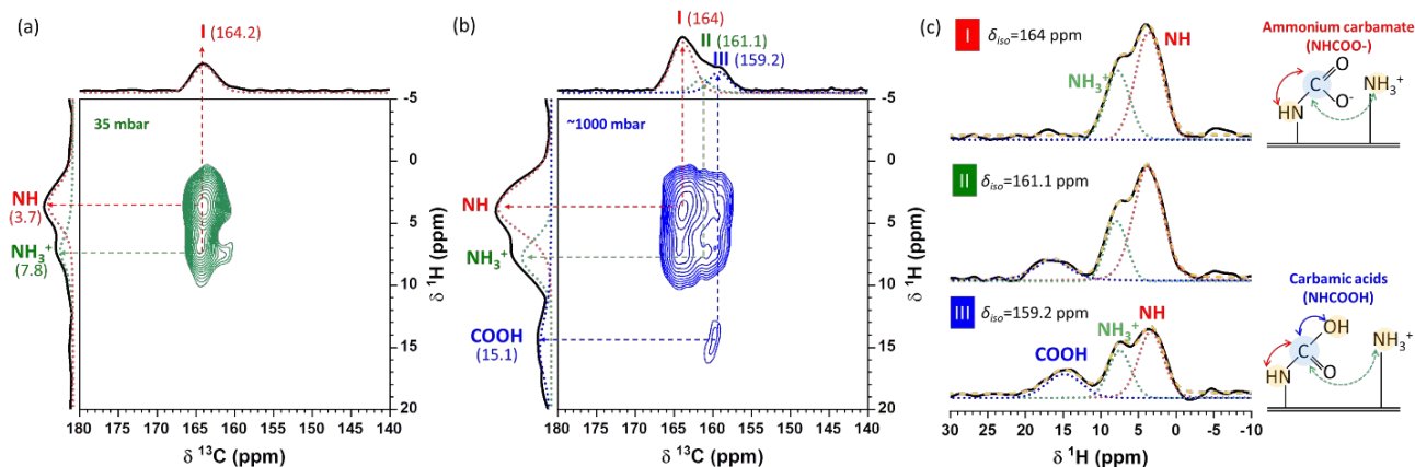
Fig. 2 2D ^1\text{H} - ^{13}\text{C} FSLG-HETCOR spectra recorded with a contact time of 50 \mu\text{s} for Lewatit ® VP OC 1065 loaded with (a) 35 mbar or (b) approx. 1 bar of ^{13}\text{CO}_2 . The chosen contact time of 50 \mu\text{s} highlights protonated carbon sites. (c) Individual ^1\text{H} projection for each ^{13}\text{C} environment (I, II, and III in (b)) observed in the 2D spectrum in (b) at approximately 1 bar of ^{13}\text{CO}_2 are deconvoluted with colored dashed lines: NH (red), \text{NH}_3^+ (green), and COOH (blue).
