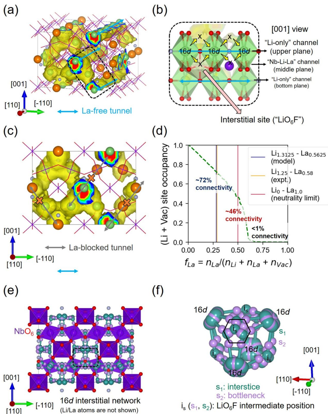
Figure 5. (a) 3D-perspective Li trajectory density within the LLNOF-L1 structure based on 1000-K AIMD calculation. La-free tunnels are indicated as light-blue double-head arrows. NbO 6 units are
