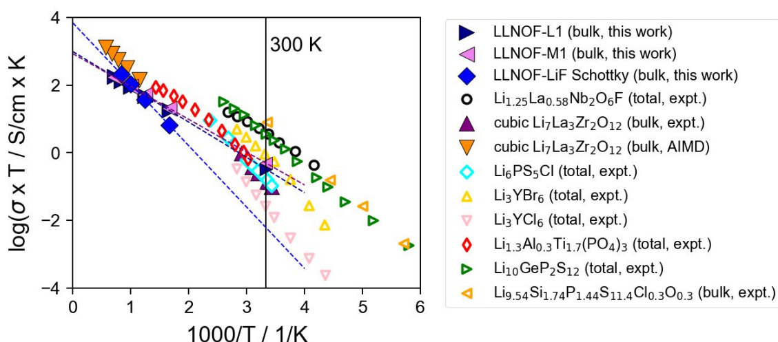
Figure 4. Comparison of the \text{Li}^+ ion conductivity of selected all-solid-state battery electrolytes: pyrochlore-type LLNOF-L1 ( \text{Li}_{1.3125}\text{La}_{0.5625}\text{Nb}_2\text{O}_6\text{F} , Figure 2b), pyrochlore-type LLNOF-M1 ( \text{Li}_{1.3125}\text{La}_{0.5625}\text{Nb}_2\text{O}_6\text{F} , Figure 2c), experimentally reported LLNOF ( \text{Li}_{1.25}\text{La}_{0.58}\text{Nb}_2\text{O}_6\text{F} ) 12 , and cubic \text{Li}_7\text{La}_3\text{Zr}_2\text{O}_{12} solid electrolyte from previous experimental and AIMD-based works 7, 34 , argyrodite \text{Li}_6\text{PS}_5\text{Cl} experimental total conductivity 35 , halide \text{Li}_3\text{YBr}_6 and \text{Li}_3\text{YCl}_6 36 , Nasicon-type \text{Li}_{1.3}\text{Al}_{0.3}\text{Ti}_{1.7}(\text{PO}_4)_3 experimental total conductivity 37 , \text{Li}_{10}\text{GeP}_2\text{S}_{12} experimental total conductivity 38 , and \text{Li}_{9.54}\text{Si}_{1.74}\text{P}_{1.44}\text{S}_{11.4}\text{Cl}_{0.3}\text{O}_{0.3} experimental bulk conductivity 39 .
