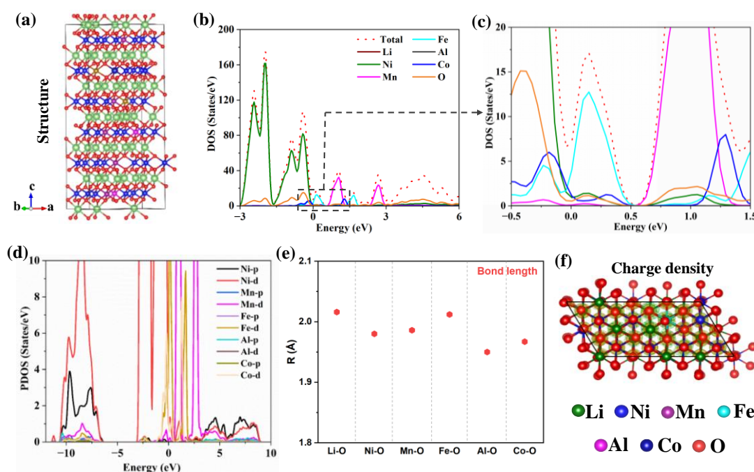
Figure 2: (a) Optimized atomic structure of NMFAC cathode. (b-d) Calculated density of states and partial density of states for NMFAC. (e, f) Bond length and charge density distribution for NMFAC.
