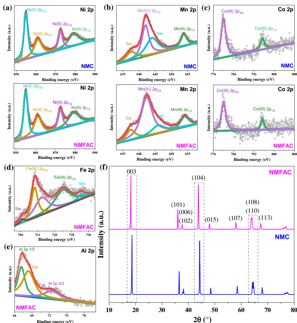
Figure 3: XPS spectra for (a) Ni 2p, (b) Mn 2p, (c) Co 2p, (d) Fe 2p, and (e) Al 2p for NMC and NMFAC. (f) XRD patterns for NMC and NMFAC.
