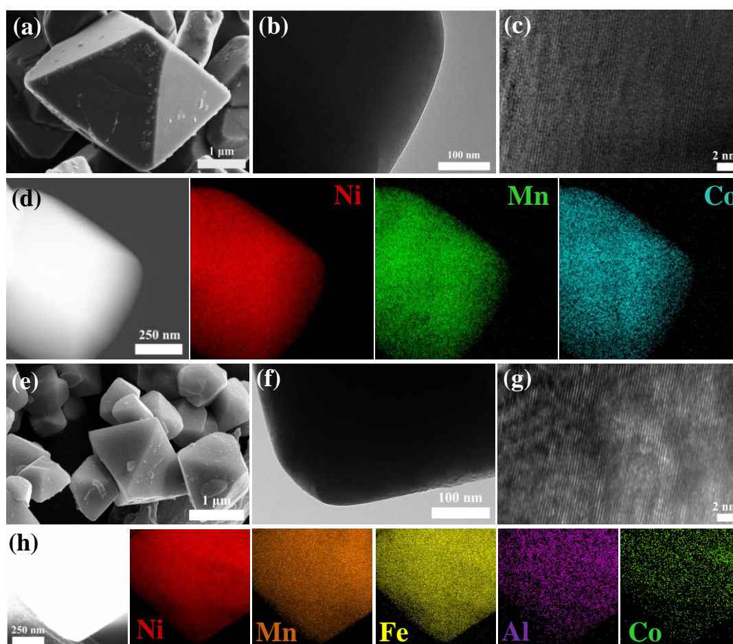
Figure 4: SEM, TEM and EDS analysis of (a-d) NMC and (e-h) NMFAC.
