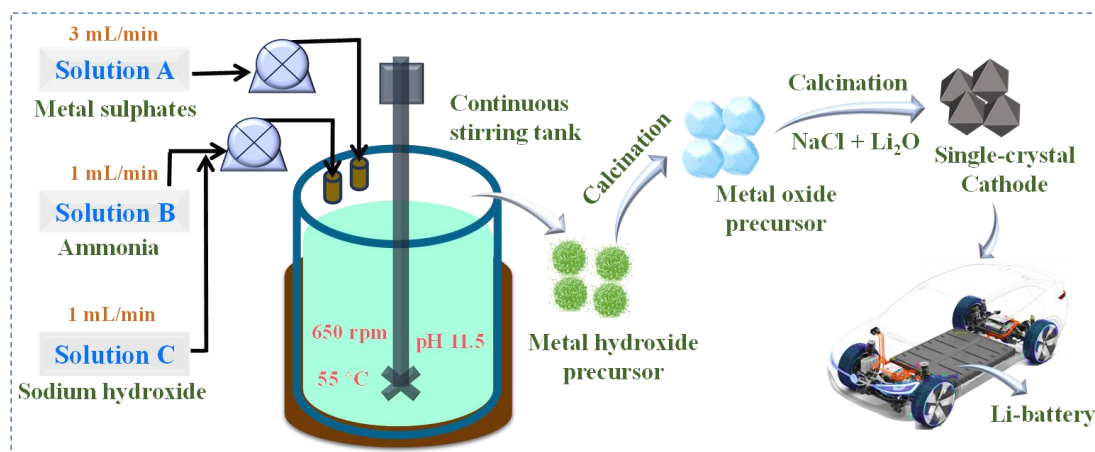
Figure 1: Schematic illustration of the synthesis process for NMC and NMFAC.
