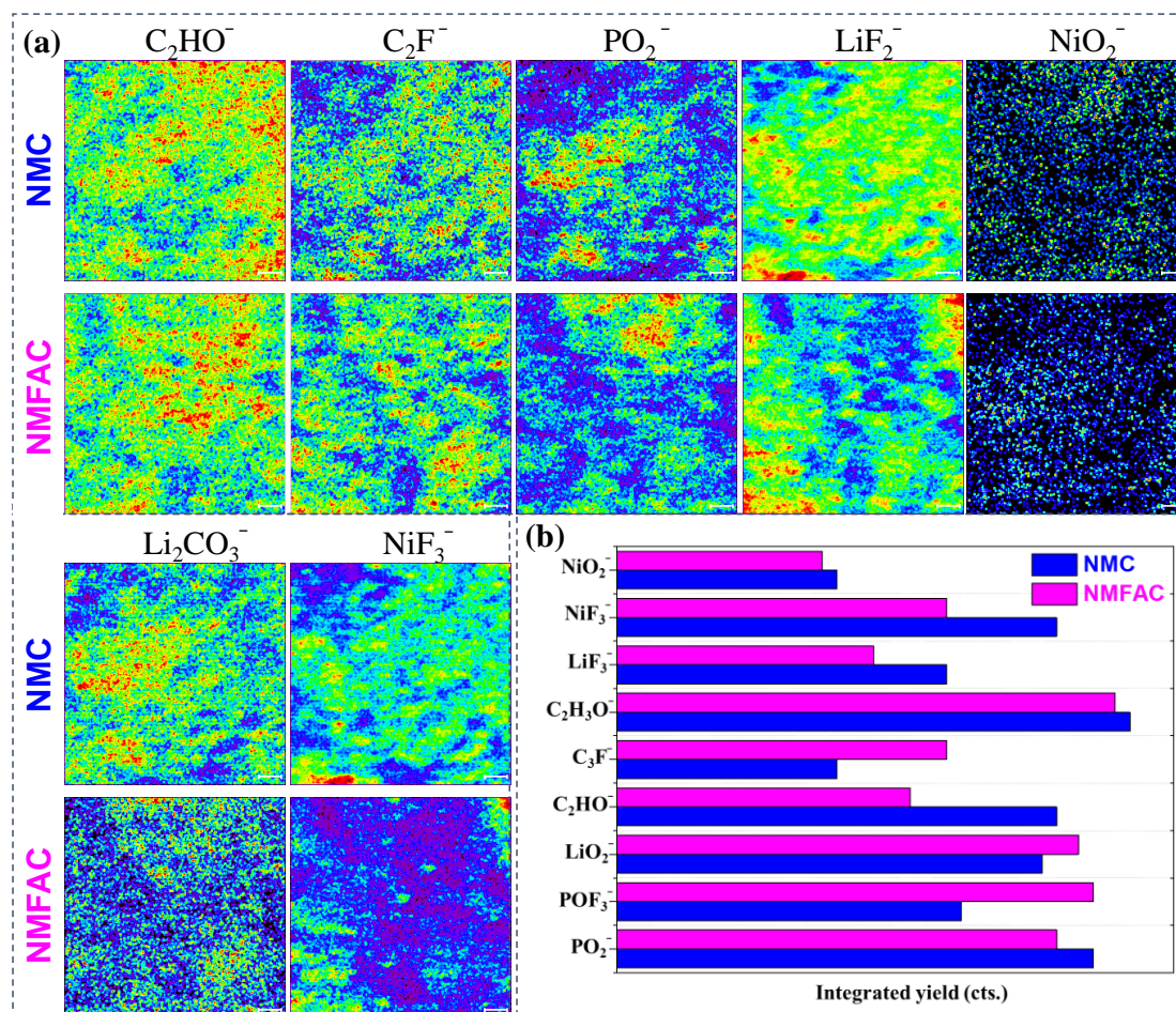
Figure 6: (a) TOF-SIMS chemical imaging and (b) integrated yields of the secondary-ion fragments of cathodes after 600 cycles.
