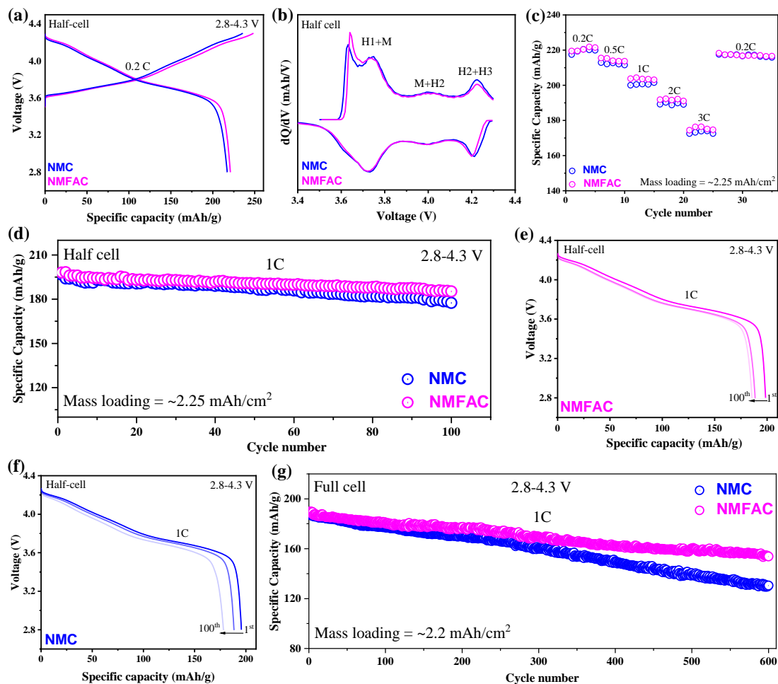
Figure 5: (a) Charge-discharge capacity and (b) dQ/dV curves at 0.2C. (c) Rate performance with different current rate for NMC and NMFAC. (d) Cycle performance, (e, f) charge-discharge curves for coin half-cells with NMC and NMFAC cathodes. (g) Cycle performance for full-cells with NMC and NMFAC cathodes.
