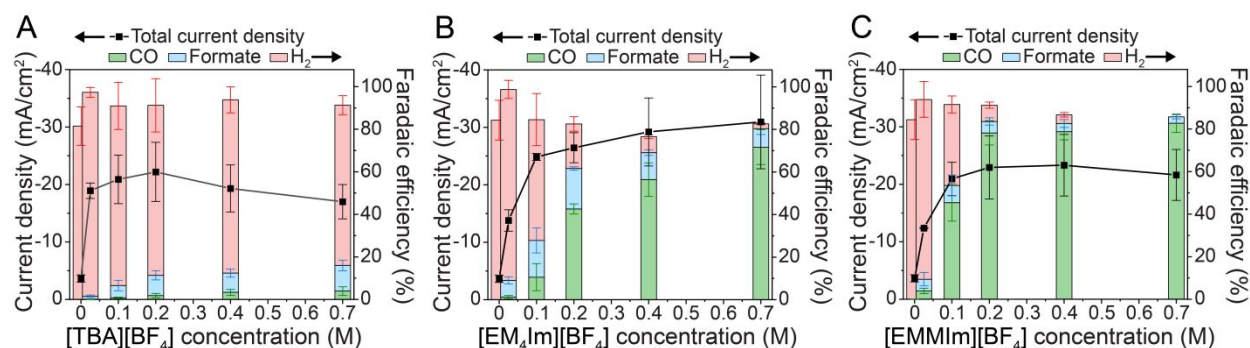
Figure 2. Total current density and product selectivity of electrochemical CO 2 reduction in (A) [TBA][BF 4 ], (B) [EM 4 Im][BF 4 ], and (C) [EMMIm][BF 4 ] electrolytes at different concentrations with 0.05 M [Et 3 NH]Cl as the proton donor. For each trial, the potential was held at -2.5 V vs Ag/Ag + for 65 min under stirring (600 rpm) and CO 2 purging. Direct reduction of [Et 3 NH] + to H 2 is the dominant reaction pathway in [TBA][BF 4 ] electrolytes. In contrast, both [EM 4 Im][BF 4 ] and [EMMIm][BF 4 ] electrolytes facilitate CO 2 reduction at concentrations higher than 0.1 M. [EM 4 Im][BF 4 ] electrolytes exhibit higher steady-state total current density and thus overall CO 2 conversion rate by producing both formate and CO, while [EMMIm][BF 4 ] electrolytes yield lower steady-state total current density but higher selectivity towards CO.
