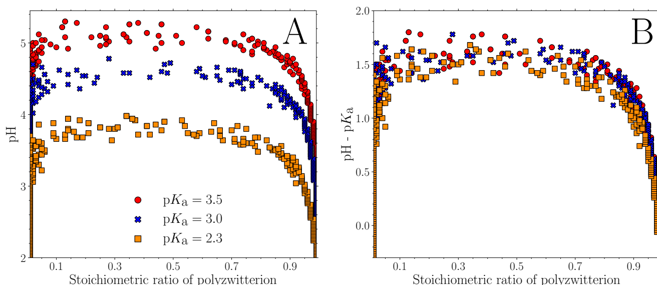
Fig. 12 Phase diagrams for various pK_a values of the pH-active charged group on the zwitterion. A) as pK_a increases, the pZCs are able to sustain complexation into the higher pH range. B) visual inspection suggests that the difference between the curves correlate closely to the differences between the pK_a values. When the curves are aligned according to the difference between pH and their pK_a , no complexation is observed beyond 2 pH units above the pK_a of the negative moiety on the zwitterion for this particular system.
