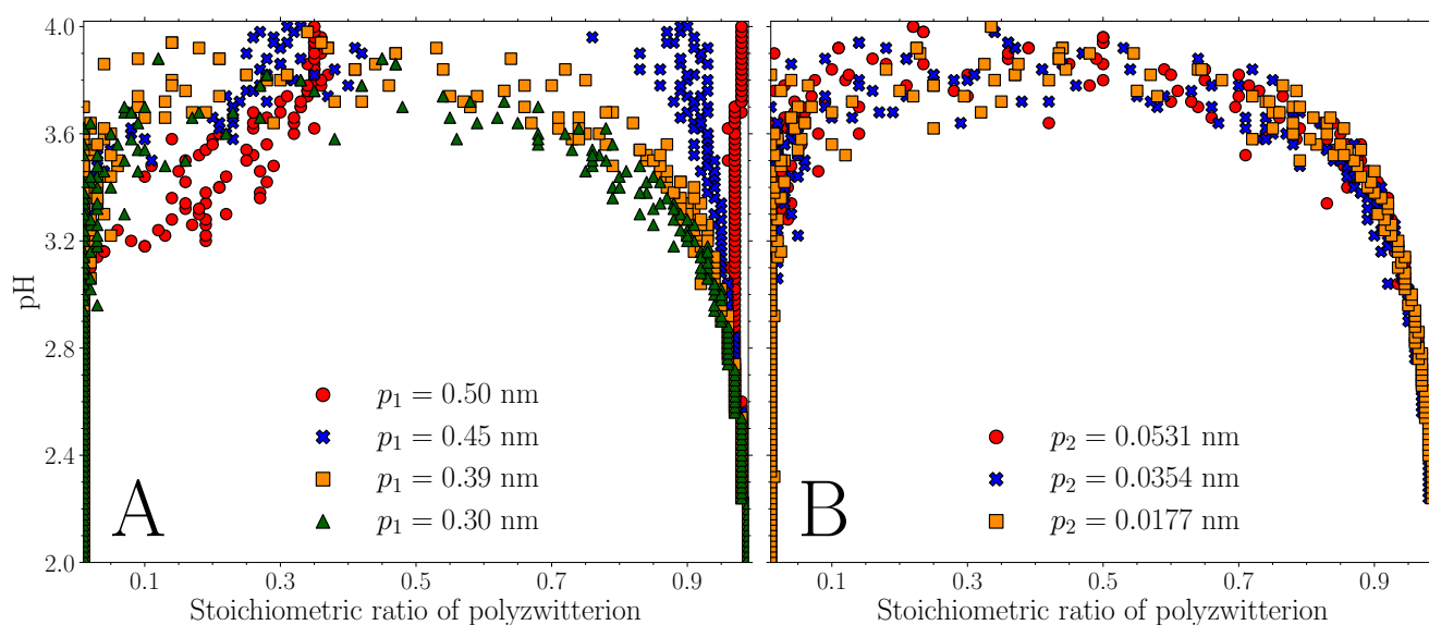
Fig. 13 Phase diagrams for various monomer dipole lengths. A) the dipole length of the zwitterionic monomer is modified while that of the polydipole is fixed. Earlier discussion about long dipole lengths of the zwitterionic monomers allowing the formation of robust polyzwitterion-polyzwitterion complexes seems to be confirmed. If the dipole length is long enough, when the primary mode of electrostatic interactions switches from charge-dipole to dipole-dipole, the latter will be sufficiently strong so as to sustain complexation even as the pH is 2 units about the pK_a value. B) the dipole length of the polydipole is modified \pm 50\% while the polyzwitterion dipole length is constant. The polydipole dipole length does not result in considerable difference in the window of complexation.
