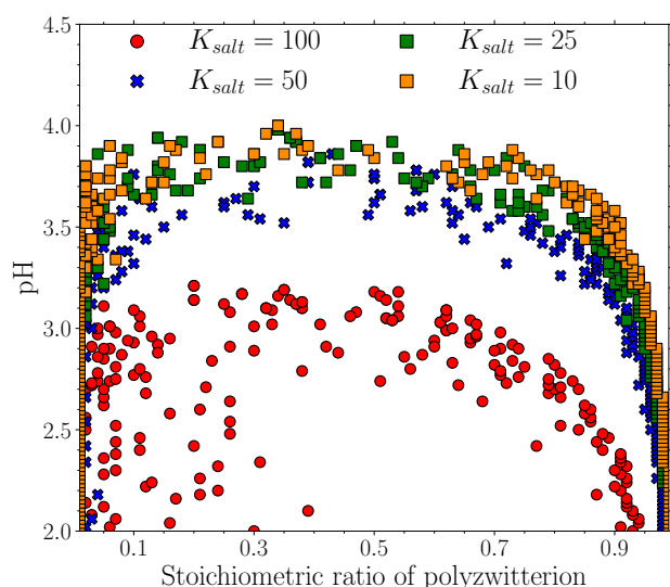
Fig. 11 Phase diagrams for various K_{salt} values of the permanently charged group on the zwitterion. A) as K_{salt} increases, the permanently charged group is more likely to have a small negative salt ion condensed onto it thus suppressing the polyzwitterion's ability to be involved in charge-dipole electrostatic interactions that sustain pZC formation. B) complexation becomes less probable with decreasing stoichiometric ratio and increasing pH.
