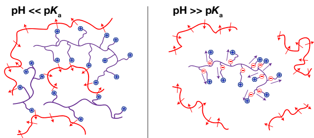
Fig. 1 Illustration of our model system. Our system consists of polyzwitterions (purple curves), protonated polyanions (i.e., polydipoles; red curves), positive and negative monovalent salt ions (not shown), and solvent (not shown). The charged groups of the polyzwitterion are depicted as blue positive symbols and red negative symbols tethered to the backbone. The negative moiety is the pH-active group on each zwitterionic monomer while the positive moiety is a permanent charge, subjected only to small salt ion condensation reactions. Left : at a pH sufficiently lower than the pK_a of the negative moiety on the zwitterion, the negative charges of the polyzwitterion are neutralized and complexation between polyzwitterions and dipolar polyanions occurs, forming polyzwitterionic complexes (pZCs). Right : once the pH is raised to be sufficiently higher than the pK_a of the negative moiety on the zwitterion, the negative charges on the polyzwitterion are ionized. Thus, the polyzwitterion monomers adopt a dipolar state and, concurrently, the pZC dissociates. It is important to note that the orientation of the charged groups along the side chain is not taken into consideration in our theory. Adapted from Margossian, K. O. et al., Nat. Commun. 13:2250, 2022. Licensed under CC BY 4.0.
