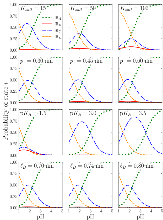
Fig. 4 Zwitterion state probability distributions with respect to key parameters. Moving downward row-wise, the effect of: K_{salt} , p_1 , pK_a , and temperature. The parameters for each set of probability distributions are enumerated as follows, unless noted otherwise: T = 298 K, p_1 = 0.39 nm, K_{salt} = 25 , and pK_a = 2.3 . Temperature is related to \ell_B and at 298 K, \ell_B = 0.72 nm. The temperatures which correspond to \ell_B = 0.70 , 0.74 , and 0.80 nm are 273, 323, and 373 K, respectively.
