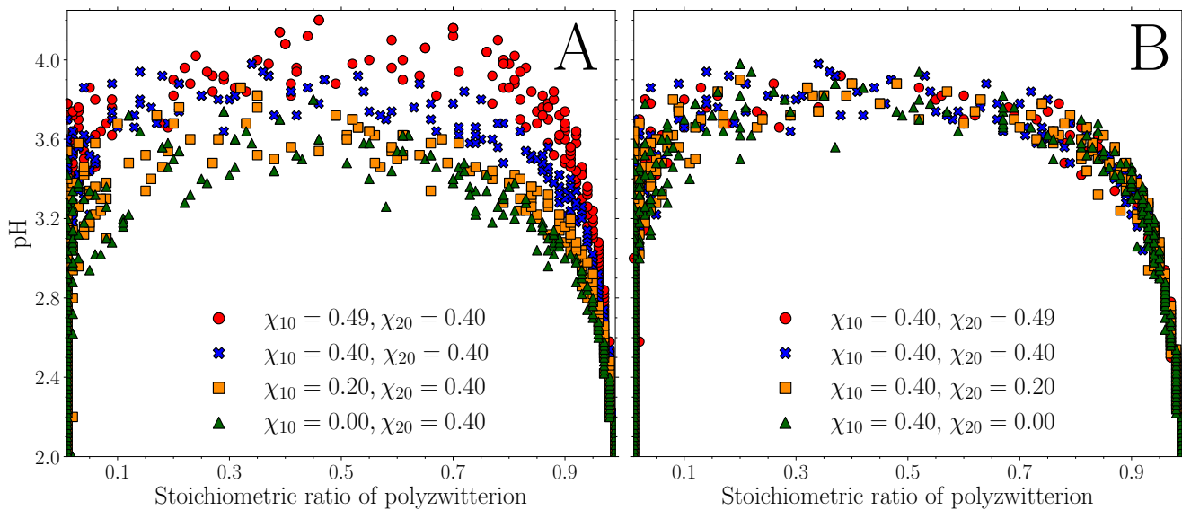
Fig. 10 Phase diagrams for unequally hydrophobic polymers. A) the hydrophobicity of the polyzwitterion is varied while the hydrophobicity of the polydipole is constant. B) the hydrophobicity of the polydipole is varied while that of the polyzwitterion is constant. Similar to the study of the chain lengths, the hydrophobicity of the polydipole does not significantly contribute to the overall phase behavior of the pZC.
