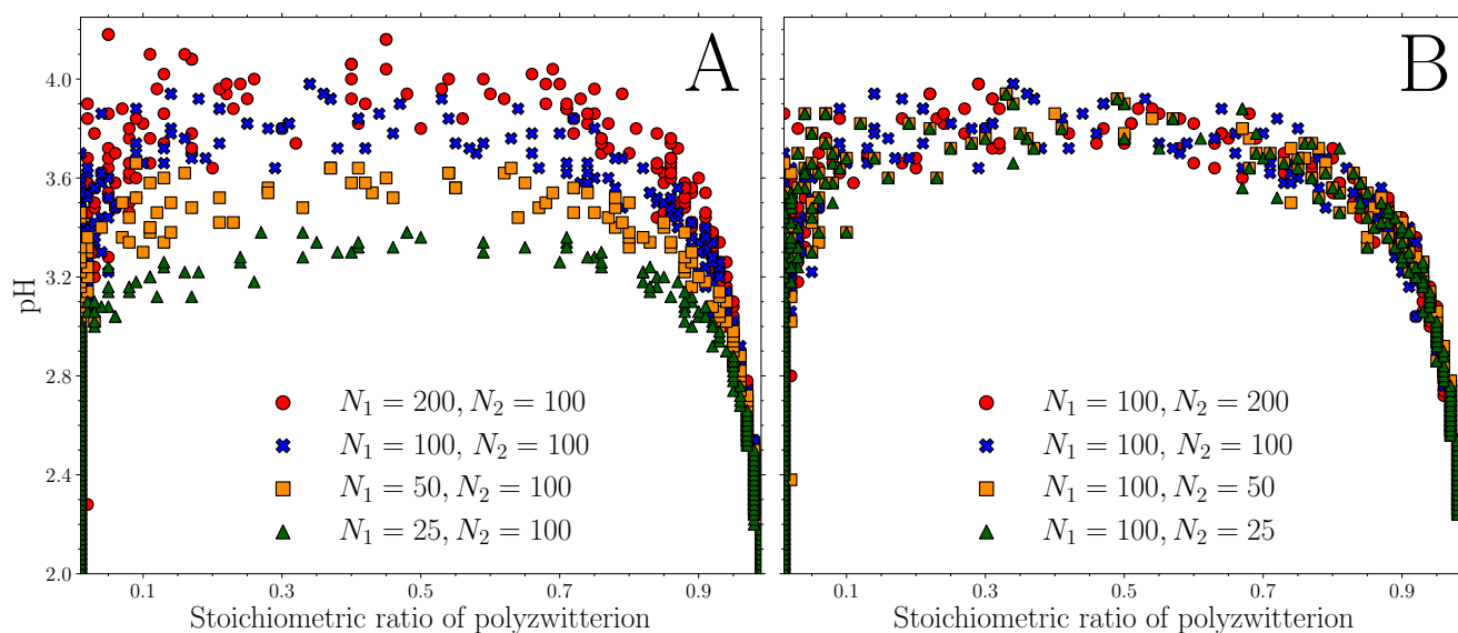
Fig. 8 Phase diagrams for asymmetrical polymer chain lengths. A) varying the chain length of the polyzwitterion while the polydipole chain length is fixed. B) varying the chain length of the polydipole while that of the polyzwitterion is held constant.
