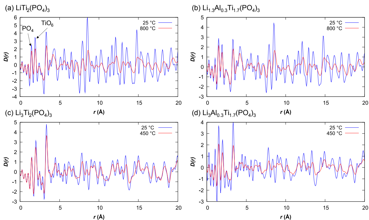
Figure 4 – Experimental X-ray PDFs ( Q_{\text{max}} = 18 \text{ \AA}^{-1} ) at selected temperatures of (a) \text{LiTi}_2(\text{PO}_4)_3 ; (b) \text{Li}_{1.3}\text{Al}_{0.3}\text{Ti}_{1.7}(\text{PO}_4)_3 ; (c) \text{Li}_3\text{Ti}_2(\text{PO}_4)_3 and (d) \text{Li}_3\text{Al}_{0.3}\text{Ti}_{1.7}(\text{PO}_4)_3 .
