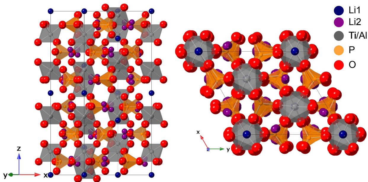
Figure 1 – Crystal structure of \text{Li}_{1+x}\text{Al}_x\text{Ti}_{2-x}(\text{PO}_4)_3
