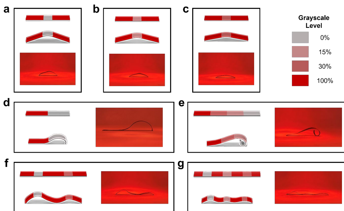
Fig. 5 The programmability of the SPSA under global heating by the nIR light for 2 s. (a-c) Bending curvatures as grayscale levels of the UV photomask for preparing the bending joint gradually increase from (a) 0%, (b) 15%, to (c) 30%. (d-g) Examples of more complex shape changes and programmability through UV photomasks with spatially programmed grayscales, including (d) laying down hook, (e) smoother laying down hook, (f) M shape, and (g) trefoil arch shape. The LCE layers were facing downward for all configurations.
