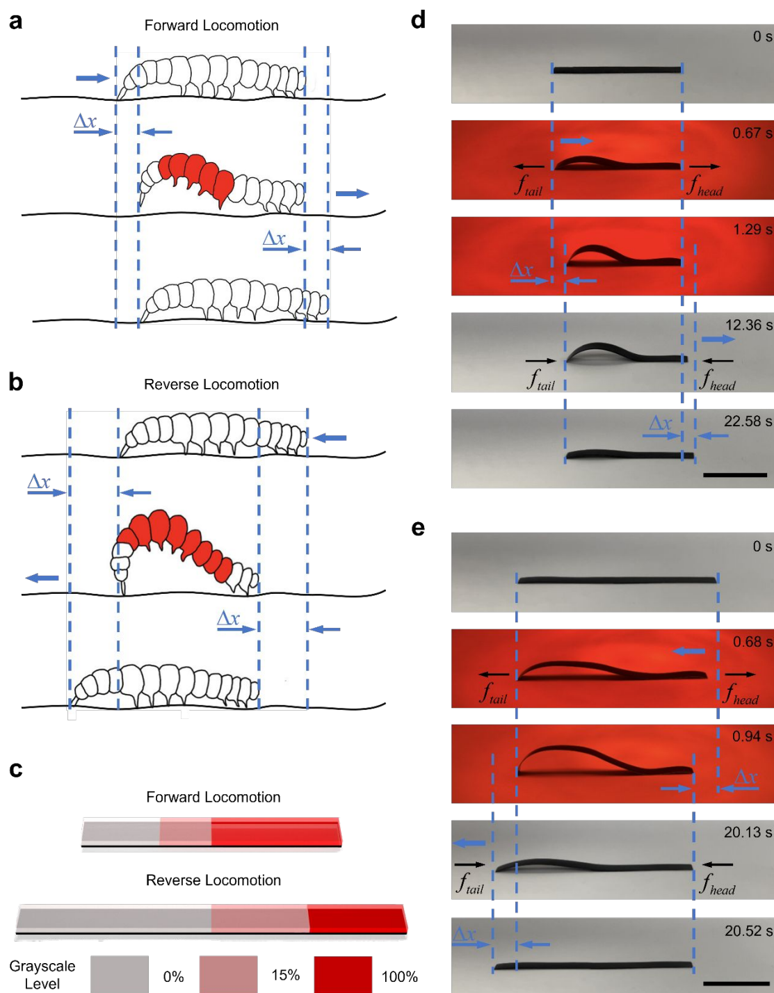
Fig. 6 Caterpillar-inspired soft crawling robots demonstrating locomotion under global heating using an nIR light. (a–b) Schematics showing the forward and backward locomotion modes of the caterpillar. (c) Two patterns of the soft crawling robot enabling forward and backward locomotion. Snapshots of (d) forward and (e) backward locomotion modes of the soft crawling robots, actuated by intermittently turning on and off the nIR lamp. Scale bars: 20 mm.
