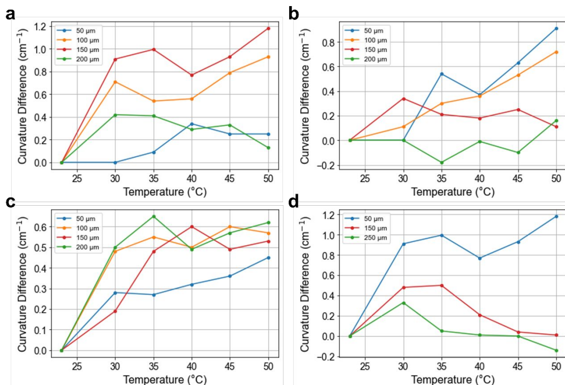
Fig. 2 Curvature differences between SPSAs with the UV-exposed and non-UV-exposed BP-PDMS. (a-c) Curvature differences as a function of temperature for a gPDMS layer thickness of 50 \mu\text{m} and BP-PDMS layer thicknesses ranging from 50 to 200 \mu\text{m} , with LCE layer thicknesses of (a) 150 \mu\text{m} , (b) 300 \mu\text{m} , and (c) 450 \mu\text{m} . (d) Curvature differences as a function of temperature for BP-PDMS and LCE layer thicknesses of 150 \mu\text{m} , and gPDMS layer thicknesses ranging from 50 to 250 \mu\text{m} .
