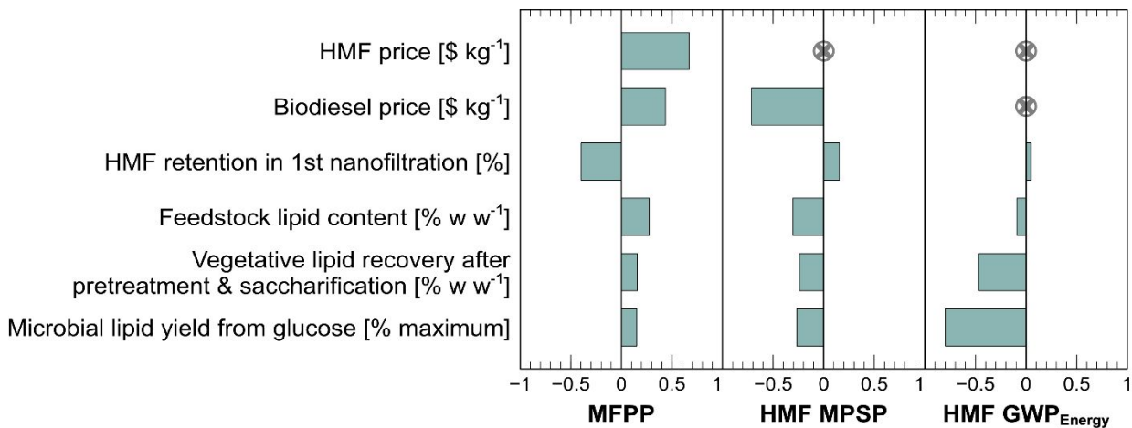
Figure 3. Spearman's \rho values between parameters and MFPP, HMF MPSP, and energy-allocated HMF GWP 100 .
