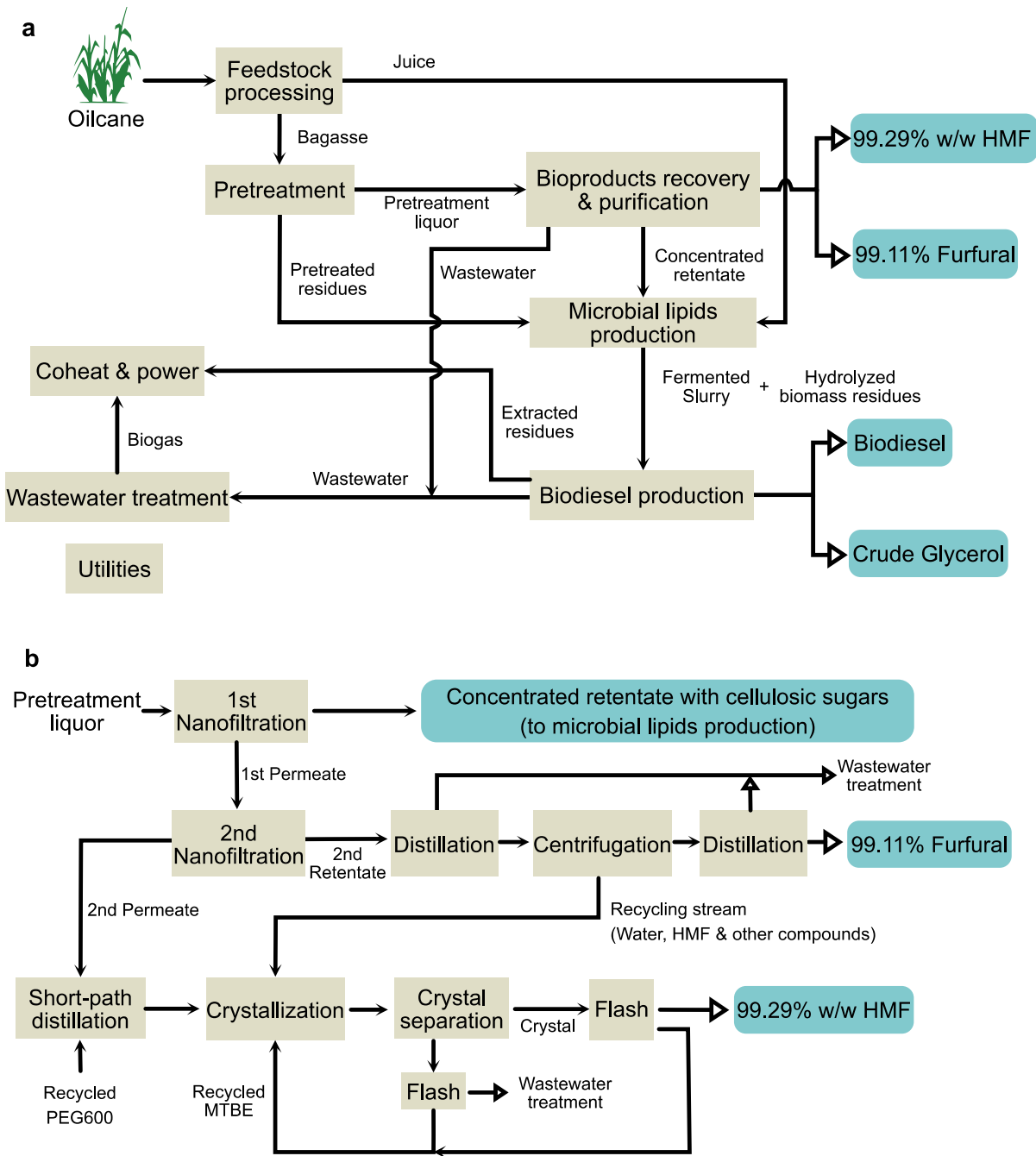
Figure 1: Simplified flow diagram of the proposed biorefinery for (a) coproduction of HMF, furfural, biodiesel, and crude glycerol from oilcane, and (b) bio-based products recovery and purification section of the proposed biorefinery. Acronyms in the figure denote polyethylene glycol 600 (PEG600), and methyl tert-butyl ether (MTBE).
