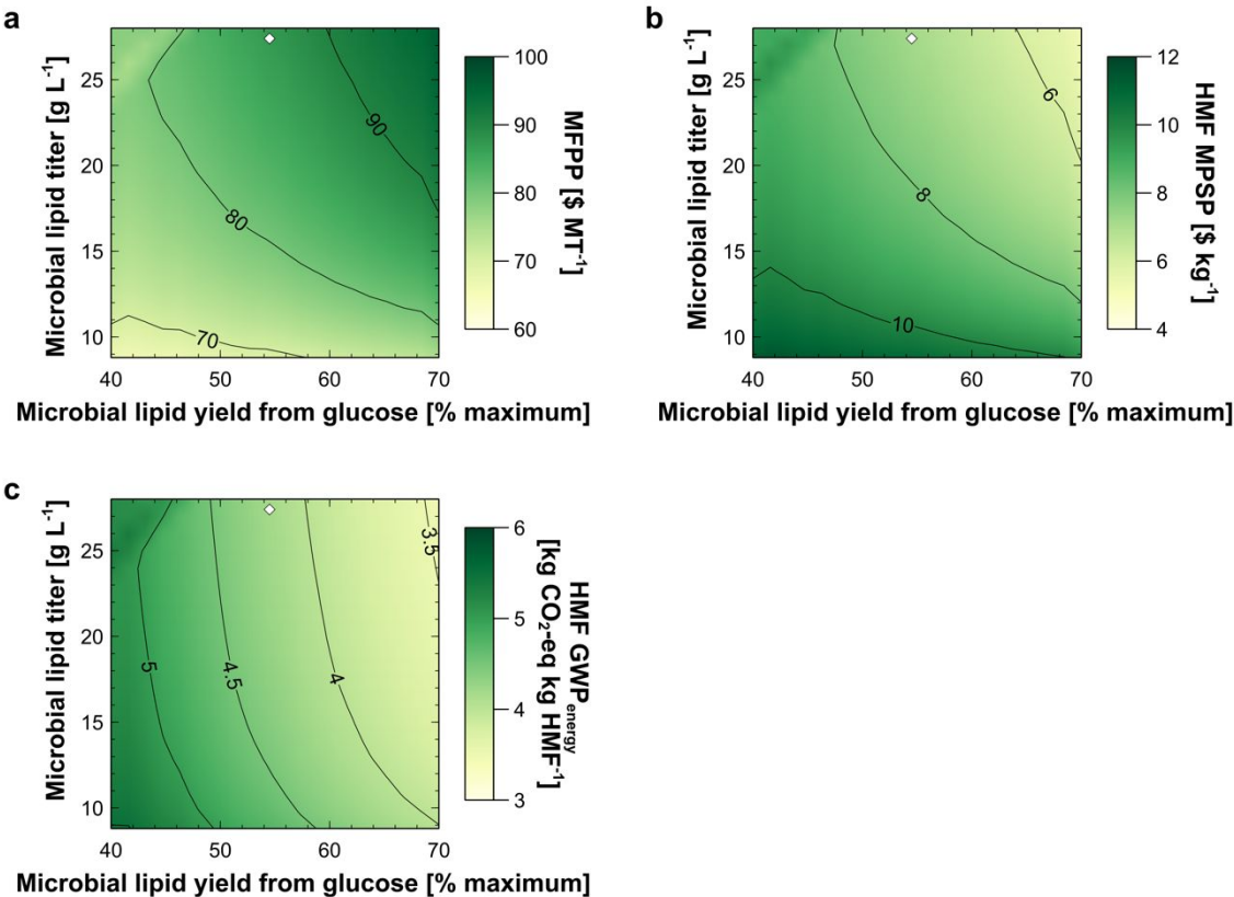
Figure 4. a) MFPP, b) HMF MPSP and c) HMF GWP 100 using energy allocation at different combinations of microbial lipid yield from glucose and microbial lipid titer using baseline assumptions of other parameters. Diamond markers represent values obtained from the baseline biorefinery.
