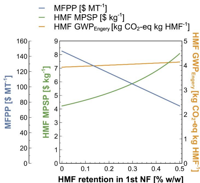
Figure 6. MFPP, HMF MPSP and HMF GWP 100 using energy allocation at different HMF retention in 1 st NF (nanofiltration) using baseline assumptions of other parameters.
