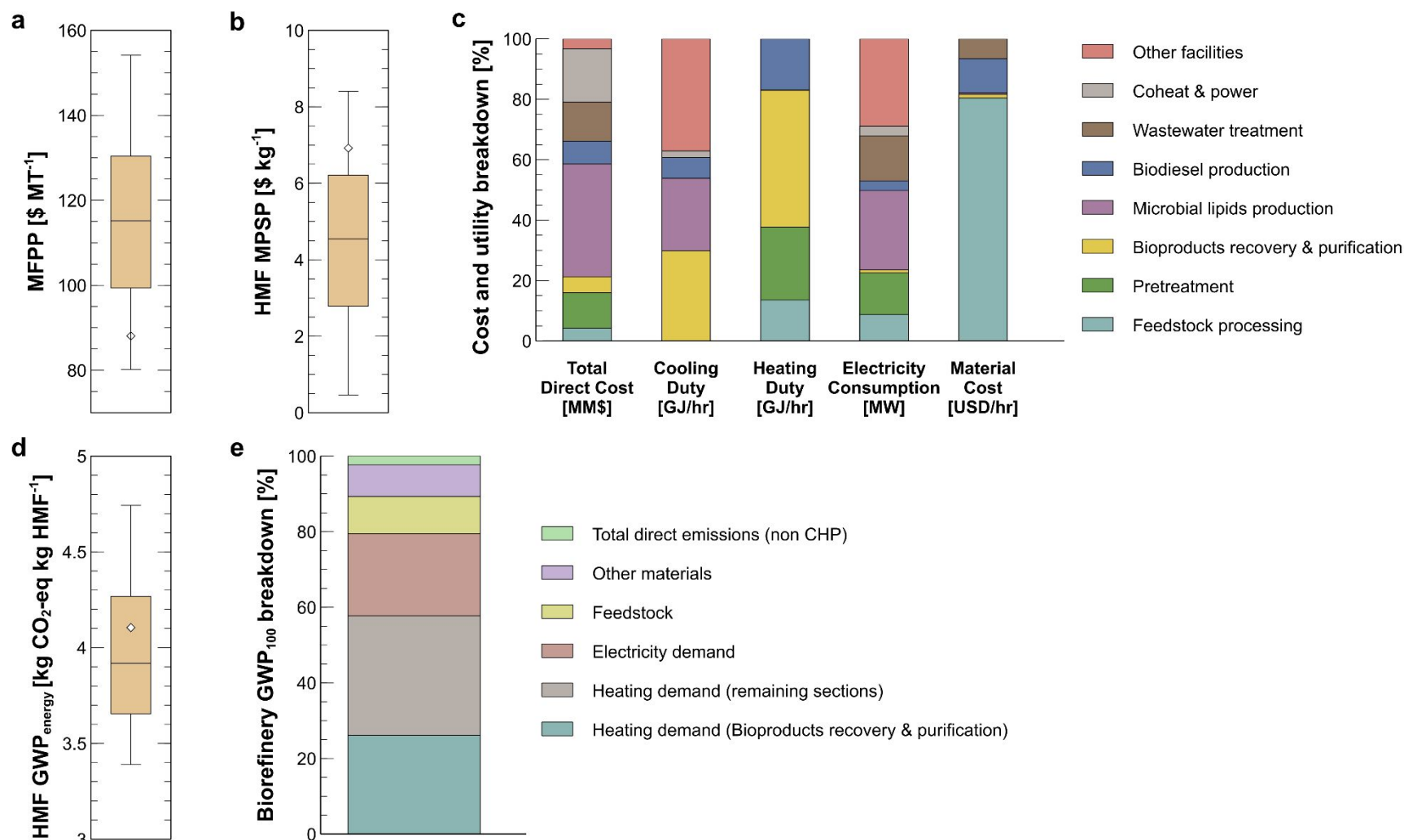
Figure 2: Cost estimation and environmental impacts of the biorefinery. Box and whisker plots of a) MFPP and b) HMF MPSP, c) breakdown of total direct cost and utility usage of baseline biorefinery, d) box whisker plot and e) breakdown of HMF GWP 100 . Diamond markers in box and whisker plots represent values obtained from baseline biorefinery.
