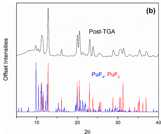
Figure 4: (a) Thermal decomposition of PuF 4 ·xH 2 O under nitrogen heated to 800 °C at a ramp rate of 5 °C/min. (b) ICDD patterns for PuF 4 (#00-041-1218, blue) and PuF 3 (#00-006-0327, red) in comparison to post-TGA PuF 4 ·xH 2 O.
