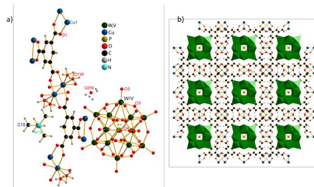
Fig. 2 (a) A structural fragment of \text{PVW}_{11}@HKUST-1 . The vanadium and tungsten atoms occupy the same crystallographic site in each [\text{PVW}_{11}\text{O}_{40}]^{4-} anion, with occupancies of 0.08 and 0.92, respectively. (b) Structure of \text{PVW}_{11}@HKUST-1 viewed along the [100] direction. Positional disorder of encapsulated Keggin anions is not depicted. Selected bond lengths [Å] and angles [°]: 1 : W1-O3 1.890(4), W1-O2 1.681(13), W1-O4 2.478(14), Cu1-Cu1 4 2.639(4), Cu1-O1 1.948(6), Cu1-O1W 2.187(15), P1-O4 1.52(3); O3-W1-O3 86.8(5), O3-W1-O3 155.7(8), O3-W1-O3 88.2(6), O3-W1-O4 92.8(5), O2-W1-O3 102.1(4), O2-W1-O4 159.3(5), O1-Cu1-Cu1 84.61(19), O1-Cu1-O1 90.2(4), O1-Cu1-O11 87.4(4), O1-Cu1-O11 103.2(4), O4-P1-O4 109.471(2). a 1/2-X, 1-Y, 1/2-Z (See ESI)
