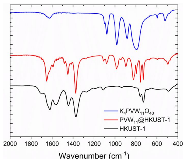
Fig. 3 FTIR spectra of 1 and its constituents HKUST-1 and the mono-vanadium substituted Keggin POM K 4 [α-PVW 11 O 40 ] in the 2000 – 400 cm -1 range. Prominent bands in the FTIR spectrum of 1 (cm -1 ): 1651 (s), 1591 (m), 1483 (m), 1448 (s), 1417 (m, sh), 1375 (s), 1281 (w), 1109 (w), 1080 (w), 986 (w), 947 (w), 897 (w), 824 (s), 797 (m), 756 (s), 729 (s), 669 (w), 596 (w), 496 (w), 478 (w, sh).
