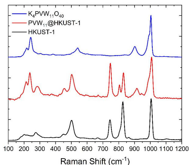
Fig. 4 Raman spectra of 1 and its constituents HKUST-1 and the mono-vanadium substituted Keggin POM K 4 [α-PVW 11 O 40 ] in the 100 – 1200 cm -1 range.
