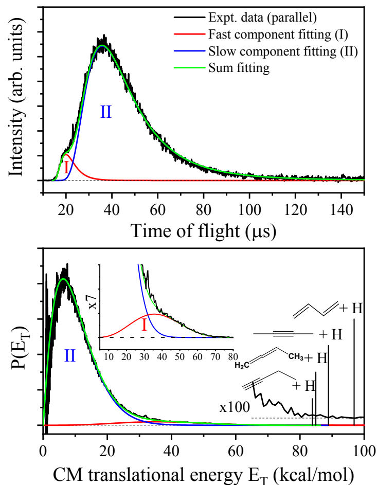
Fig. 7 The 236-nm photodissociation of 2-buten-2-yl with the polarization of the linearly polarized photolysis radiation parallel ( \parallel , \theta = 0^\circ ) to the TOF axis: (a) deconvolution fitting of the TOF spectrum with a fast component (I, red line) and a slow component (II, blue line). The deconvolution fitting results in the CM translational energy distribution is displayed in (b). The vertical lines in the bottom panel denote the maximum translational energies associated with the H-atom product channels. See text for more details.
