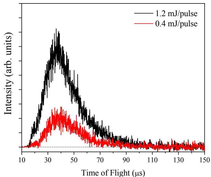
Fig. 4 Photolysis laser power dependence: the H-atom product TOF spectra of the 2-buten-2-yl at 236 nm with photolysis energy 0.4 and 1.2 mJ/pulse. The TOF spectra are normalized by the number of laser shots and are plotted on the same scale. The H-atom product signals have a linear dependence on the photolysis laser power.
