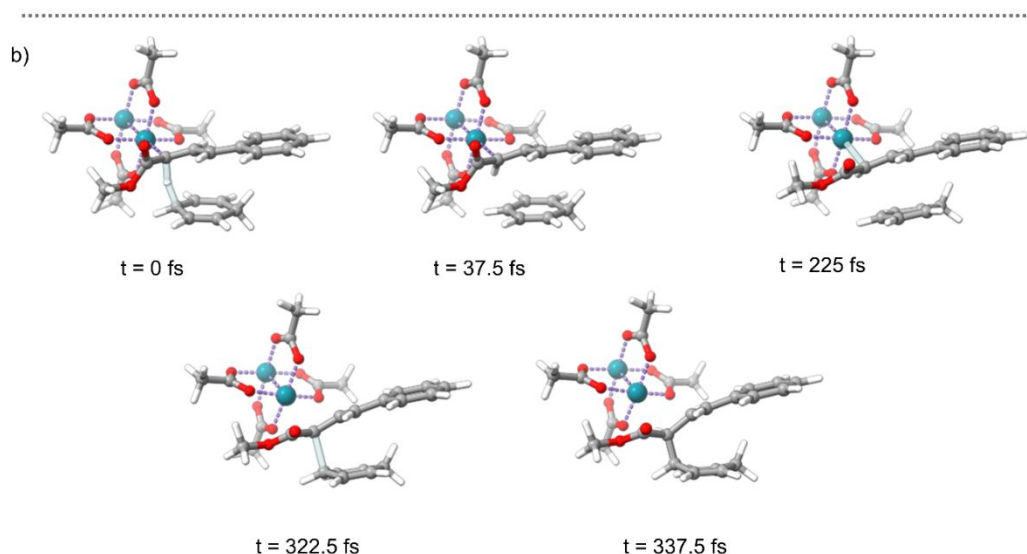
Figure 3. a) Snapshots from a dynamic reaction coordinate analysis starting from s-cis TS1 and proceeding in the forward direction. b) Snapshots from a dynamic reaction coordinate analysis starting from s-trans TS1 and proceeding in the forward direction.
