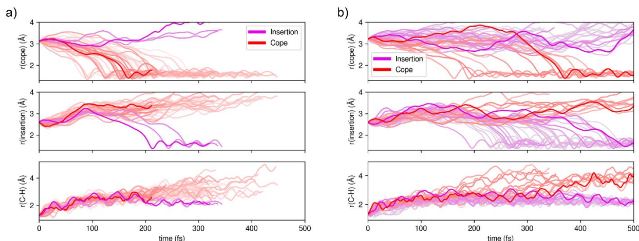
Figure 5. a) Plot of key distances (in Å) versus time (in fs) for forward progress during trajectories starting at s-cis TS1. b) Plot of key distances (in Å) versus time (in fs) for forward progress during trajectories starting at s-trans TS1. R(\text{cope}) and r(\text{insertion}) are the C-C distances for the atoms involved in forming the corresponding product. R(\text{C-H}) is the breaking C-H bond length.
