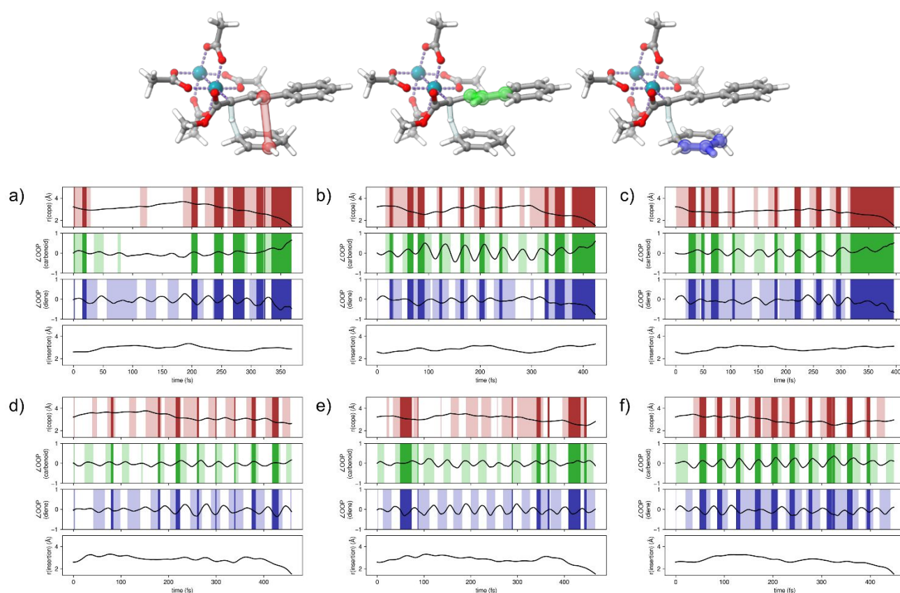
Figure 7. Plots of key coordinates for the Cope and insertion reaction for two different MD simulations starting from s-trans TS1. a-c plot of key coordinates for a trajectory that resulted in the Cope product. d-f plot of key coordinates for a trajectory resulting in the insertion product. Red regions highlight when the Cope C-C bond length is decreasing. Green areas highlight when the carbenoid carbon for the Cope product is bending away from the diene. Conversely, blue areas highlight when the Cope carbon on the diene is bending away from the carbenoid. Darker regions are when all three of these happen simultaneously.
