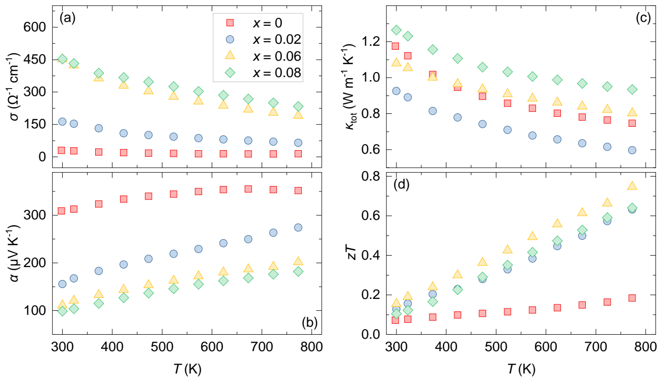
Fig. 3 Temperature dependence of the (a) electrical conductivity \sigma , (b) Seebeck coefficient \alpha , (c) total thermal conductivity \kappa_{\text{tot}} , and (d) the figure of merit zT for Bi 1-x Pb x Cu 1-x SeO ( x = 0, 0.02, 0.06 , and 0.08 ) samples.
