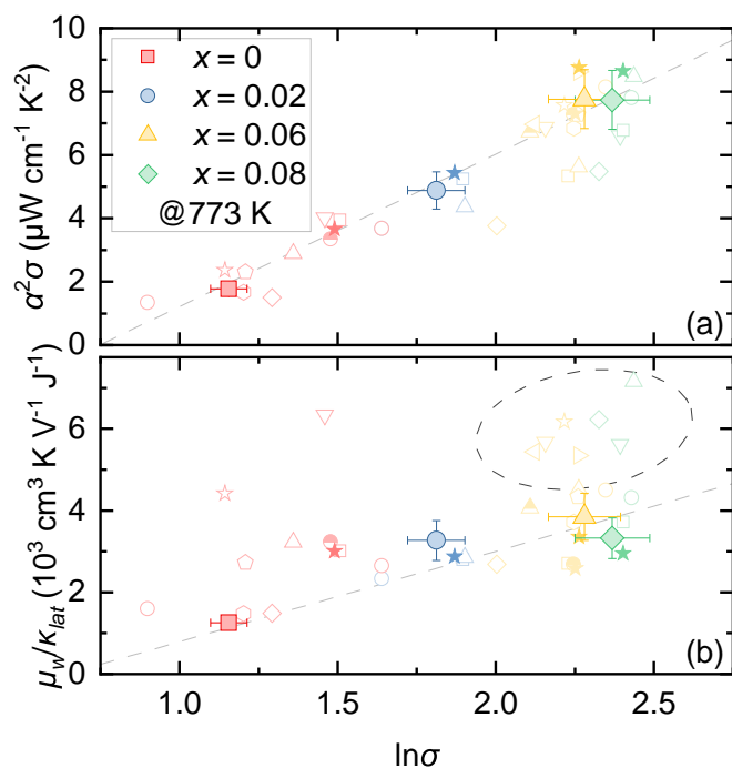
Fig. 4 (a) Power factor \alpha^2\sigma and (b) \mu_w/\kappa_{lat} ratio as functions of \ln\sigma for the \text{Bi}_{1-x}\text{Pb}_x\text{Cu}_{1-x}\text{SeO} ( x = 0, 0.02, 0.06 , and 0.08 ) samples. Literature data for other \text{Bi}_{1-x}\text{Pb}_x\text{CuSeO} -based oxyselenides are also shown for comparison (Chen et al., 24 Gu et al., 29,32 Lan et al., 18 Lei et al., 33 Li et al., 34 Liang et al., 35 Liu et al., 36 Pan et al., 37 Ren et al., 30,31 Xu et al., 38 Zhu et al. 14 ). All displayed data points correspond to values obtained at 773 K.
