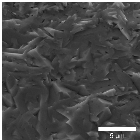
Fig. 2 SEM micrograph of the fractured cross-section of \text{Bi}_{0.94}\text{Pb}_{0.06}\text{Cu}_{0.94}\text{SeO} sample.
