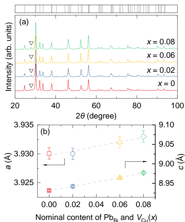
Fig. 1 (a) Powder XRD patterns of the \text{Bi}_{1-x}\text{Pb}_x\text{Cu}_{1-x}\text{SeO} ( x = 0, 0.02, 0.06, \text{ and } 0.08 ) samples. Bragg's reflections for the \text{BiCuSeO} phase are indicated by gray ticks on the top part of the figure. Diffraction peak corresponding to the \text{Bi}_2\text{O}_3 secondary phase is indicated by a black triangles ( \nabla ). (b) Lattice parameters ( a and c ) as a function of nominal concentration of \text{Pb}_{\text{Bi}} and V_{\text{Cu}} .
