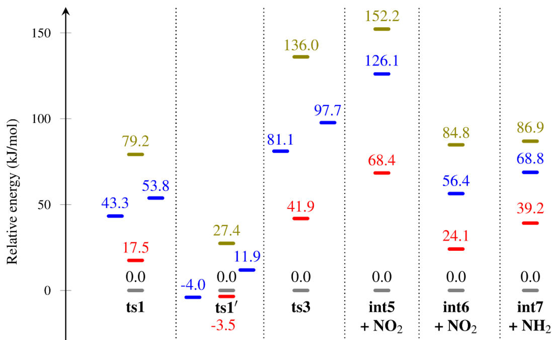
Figure 8: Change in relative energy for different species optimized in various environments: gas-phase (grey); sheet (red); surface (blue); bulk (olive). The relative energy of different species optimized in the gas phase is set to zero and are reported in kJ/mol.
