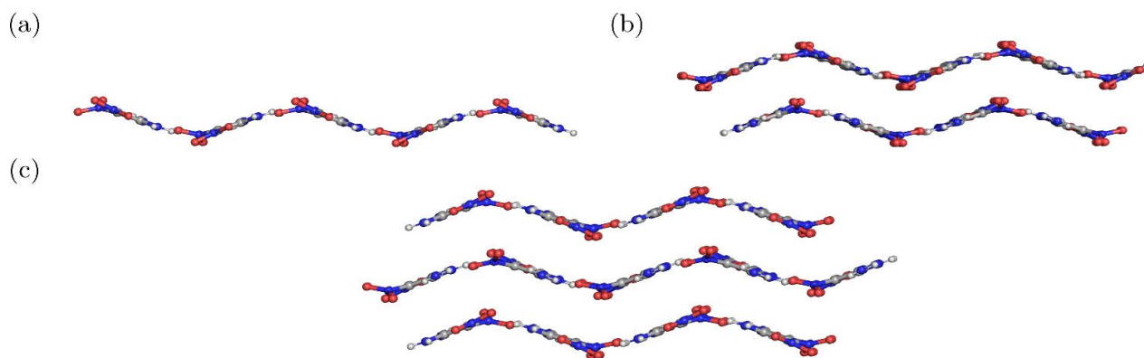
Figure 2: Representation of \alpha -FOX-7 (a) one-layer (sheet), (b) two-layer (surface), and (c) three-layer (bulk) used for the calculations.
