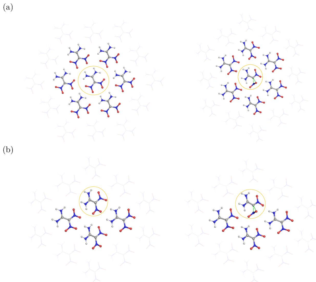
Figure 4: A representation of the neighbouring molecules to the central FOX-7 molecule (enclosed in an orange circle) for FOX-7 (left) and ts1 (right). (a) shows all the molecules in the first solvation FOX-7 and (b) shows the minimum number of neighbouring molecules for ts1 .
