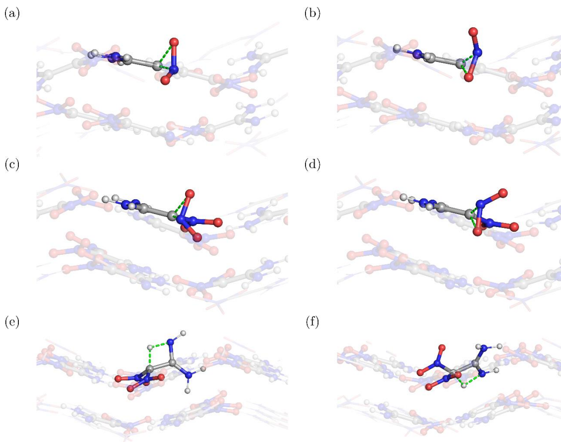
Figure 6: The structure of ts1 i.e., nitro-to-nitrite isomerization occurring facing the (a) vacuum, ts1v , and (b) bulk, ts1b , ts1' facing (c) vacuum, ts1v' and (d) facing bulk, ts1b' , and H-transfer transition state ( ts3 ) facing (e) vacuum, ts3v , and (f) bulk ts3b .
