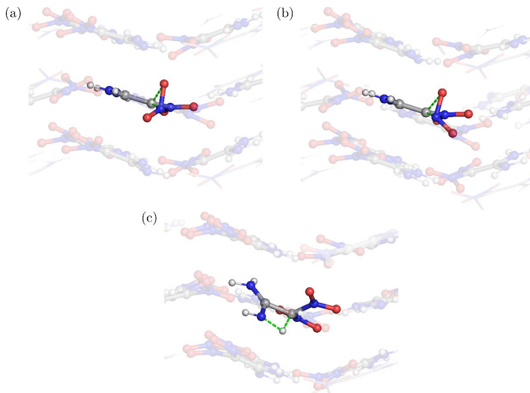
Figure 7: Side view of the transition states obtained using the bulk model (a) ts1 , (b) ts1' , and (c) ts3 .
