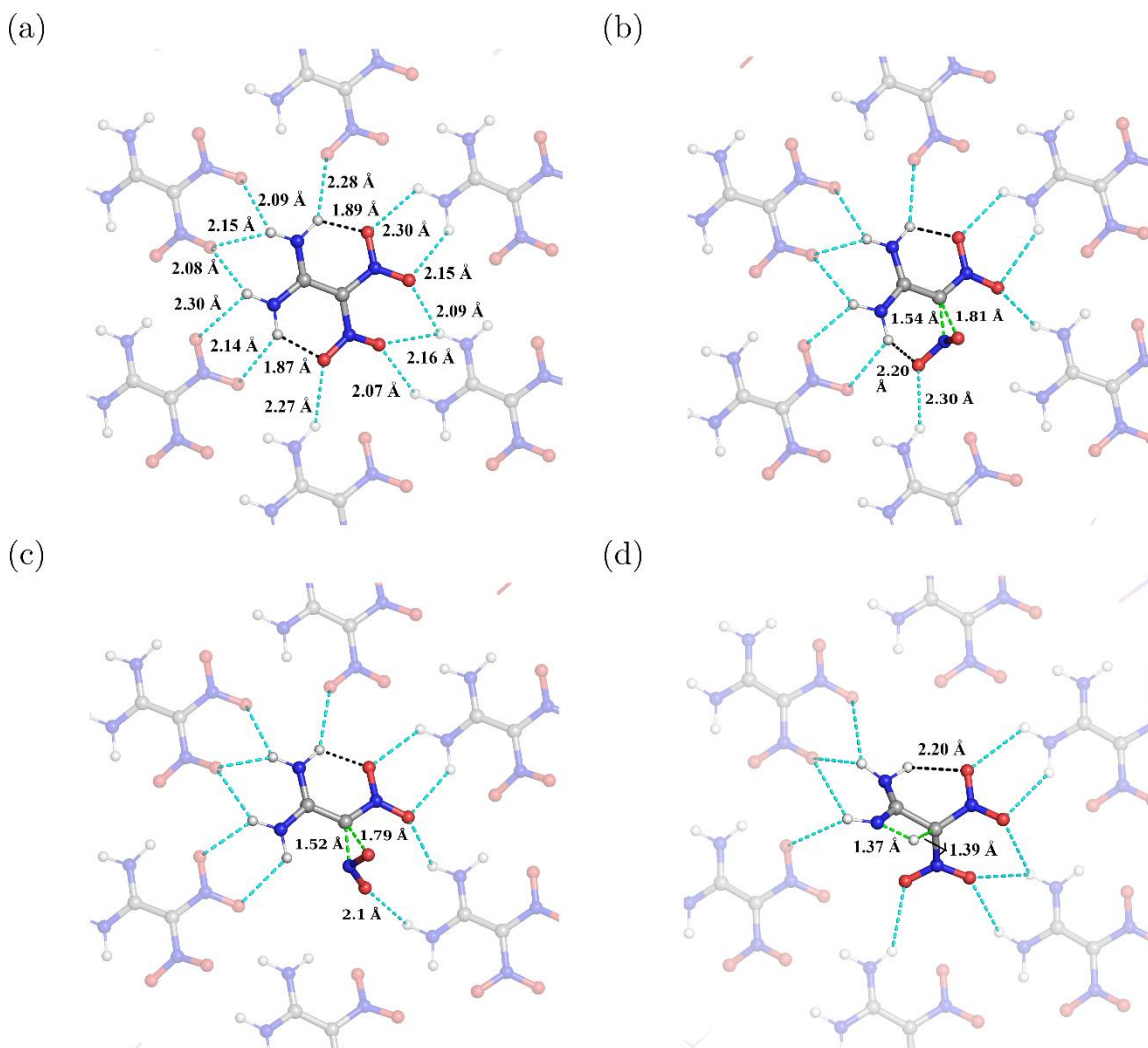
Figure 5: The restructures of important intra-(black) and intermolecular (cyan) hydrogen bonds of (a) FOX-7, (b) ts1 , (c) ts1' , and (d) ts3 .
