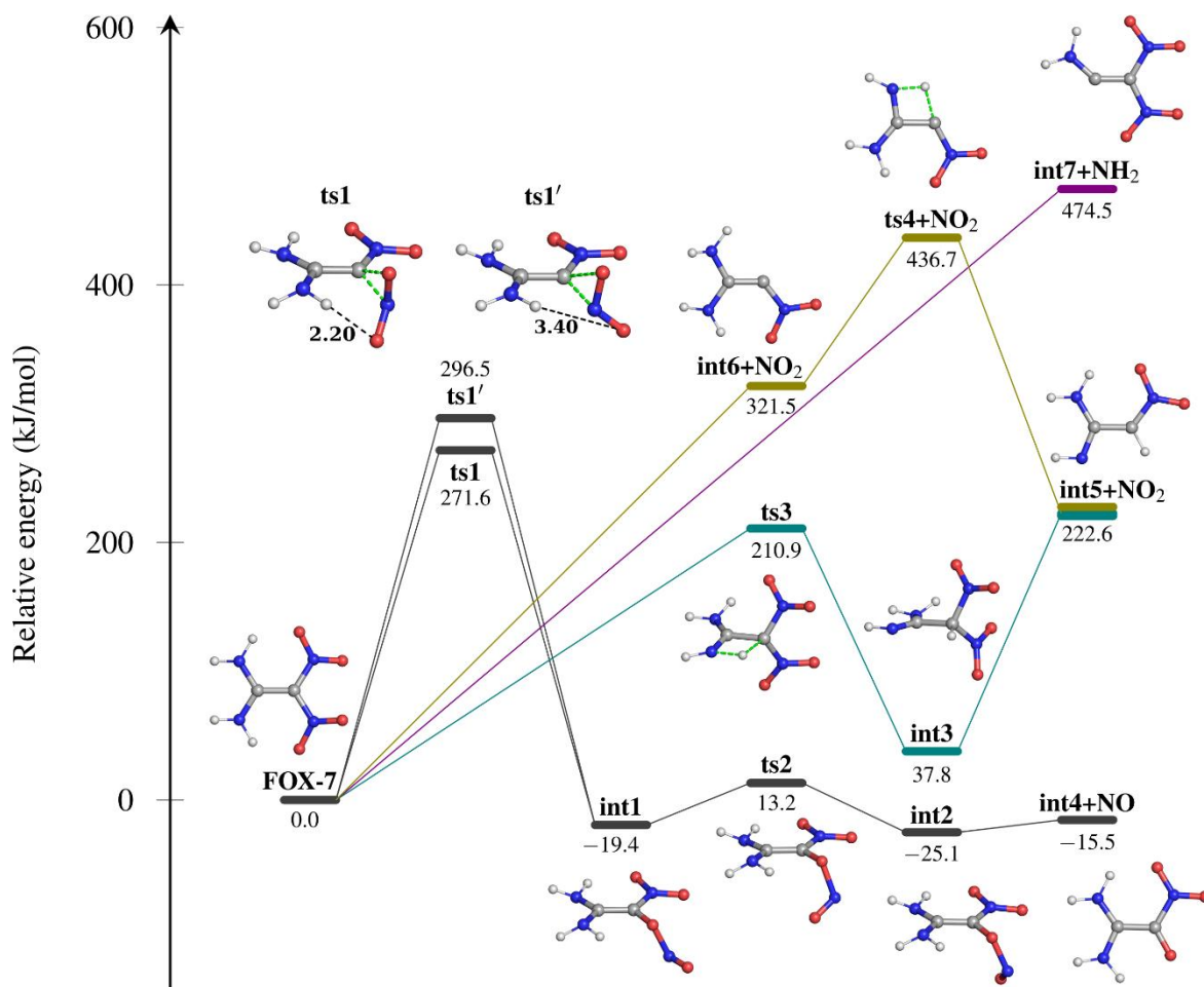
Figure 3: Potential energy profile (in kJ/mol, zero-point energy included) for the initial decomposition pathways of FOX-7 in the gas-phase at M06-2X-D3/6-31G(d) level of theory. Pathway (i), black; pathway (ii), green; pathway (iii), olive; pathway (iv), purple.
