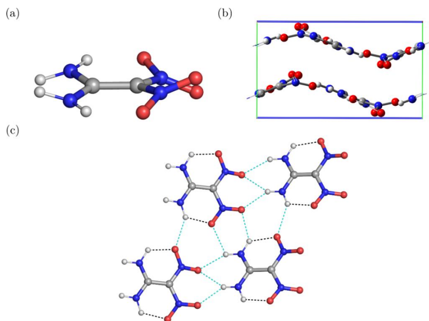
Figure 1: (a) Molecular structure of FOX-7 in the gas phase; (b) unit cell of \alpha -FOX-7; (c) top view of \alpha -FOX-7 with intramolecular (black) and intermolecular (cyan) H-bonds highlighted.
